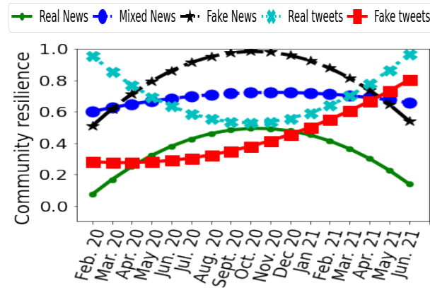
Fig 8. Output-oriented analysis of community resilience measured based on different types of news and tweets for Feb.2020–Jun. 2021.
