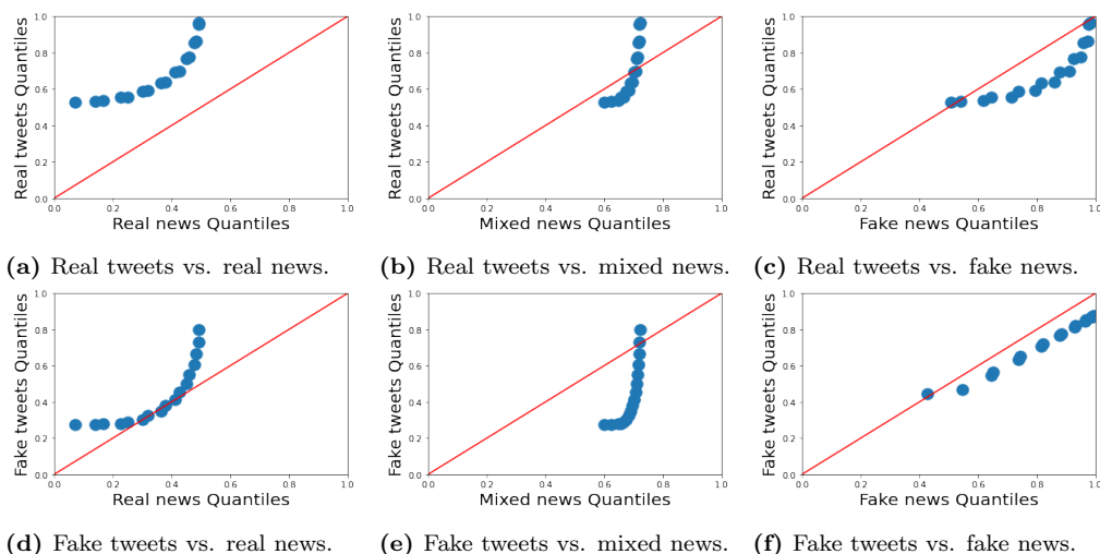
Fig 10. The Quantile-Quantile (Q-Q)-plot of news and tweets used to measure community resilience where x-axis refers to the quantiles of real, mixed, or fake news and y-axis indicates the quantiles of real, fake, or all tweets.
