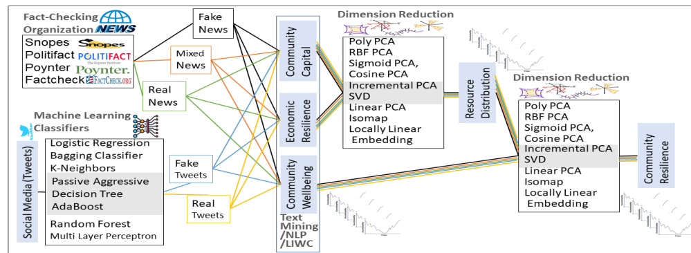
Fig 1. The proposed framework for assessing community resilience of various types of news/tweets via machine learning, natural language processing, and dimension reduction techniques.
