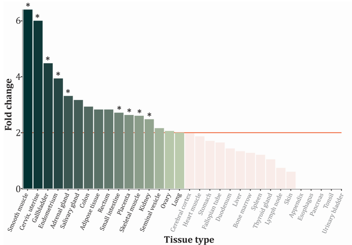
Supplementary Figure 1. Tissue enrichment identifies tissue types where the target genes are most likely to be differentially expressed. Color gradient represents decreasing fold change and light reds are insignificant associations. Stars indicate statistical significance in the tests.
