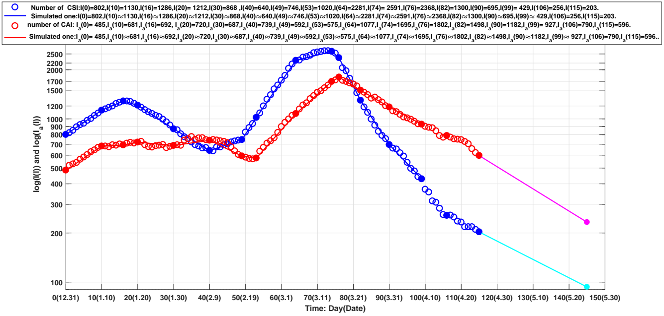
Figure 3: Blue circles: outcome of the number of the current symptomatic individuals (CSI), blue line: outcome of the corresponding simulations of equation (2). Red circles: outcome of the numbers of the current asymptomatic individuals (CAI) charged in medical observations, red line: outcome of the corresponding simulations of equation (2). The lines colored by cyan and magenta correspond to the virtual simulation results of equation (2). See Section Foreign Input Epidemic Virtual Simulations for details.
