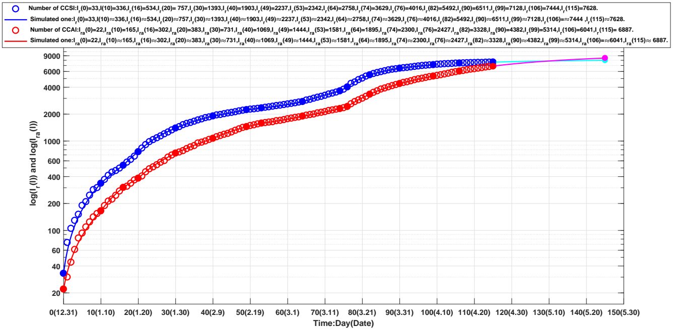
Figure 4: Blue circles: outcome of the number of the current cumulative recovered symptomatic individuals (CCSI), blue line: outcome of the corresponding simulations of equation (2). Red circles: outcome of the numbers of the current cumulative asymptomatic individuals (CCAI) discharged in medical observations, red line: outcome of the corresponding simulations of equation (2). The lines colored by cyan and magenta correspond to the virtual simulation results of equation (2). See Section Foreign Input Epidemic Virtual Simulations for details.
