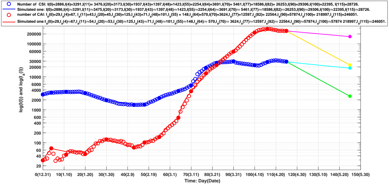
Figure 1 Blue circles: outcome of the number of the current symptomatic individuals (CSI), blue line: outcome of the corresponding simulations of equation (1). Red circles: outcome of the numbers of the current asymptomatic individuals (CAI) charged in medical observations, red line: outcome of the corresponding simulations of equation (1). The lines colored by cyan, magenta, green and yellow correspond to the virtual simulation results of equation (1). See Section Mainland Epidemic Virtual Simulations for details.
