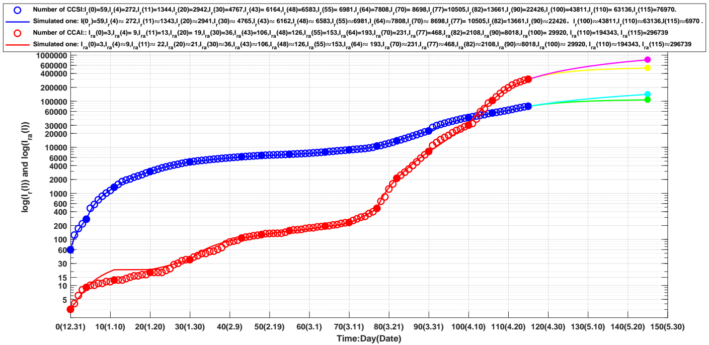
Figure 2: Blue circles: outcome of the number of the current cumulative recovered symptomatic individuals (CCSI), blue line: outcome of the corresponding simulations of equation (1). Red circles: outcome of the numbers of the current cumulative asymptomatic individuals (CCAI) discharged in medical observations, red line: outcome of the corresponding simulations of equation (1). The lines colored by cyan, magenta, green and yellow correspond to the virtual simulation results of equation (1). See Section Mainland Epidemic Virtual Simulations for details.
