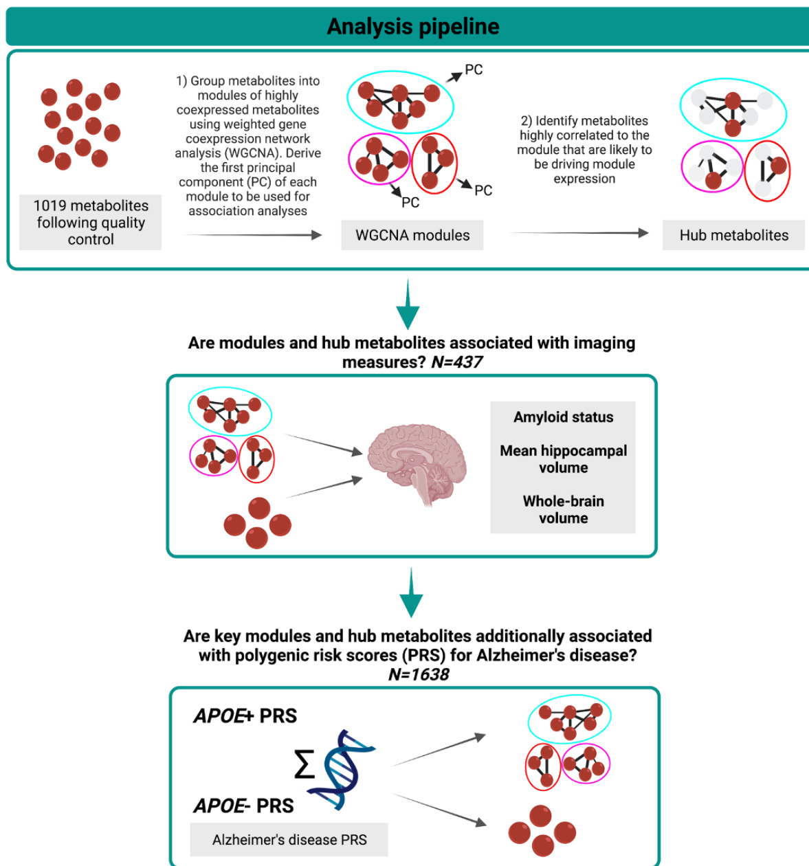
Figure 1. Analysis pipeline.
