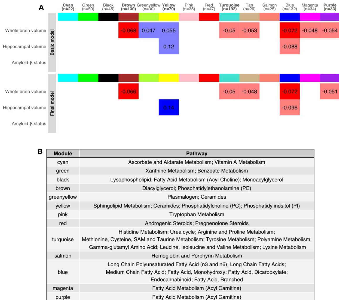
Figure 2. Module results.
