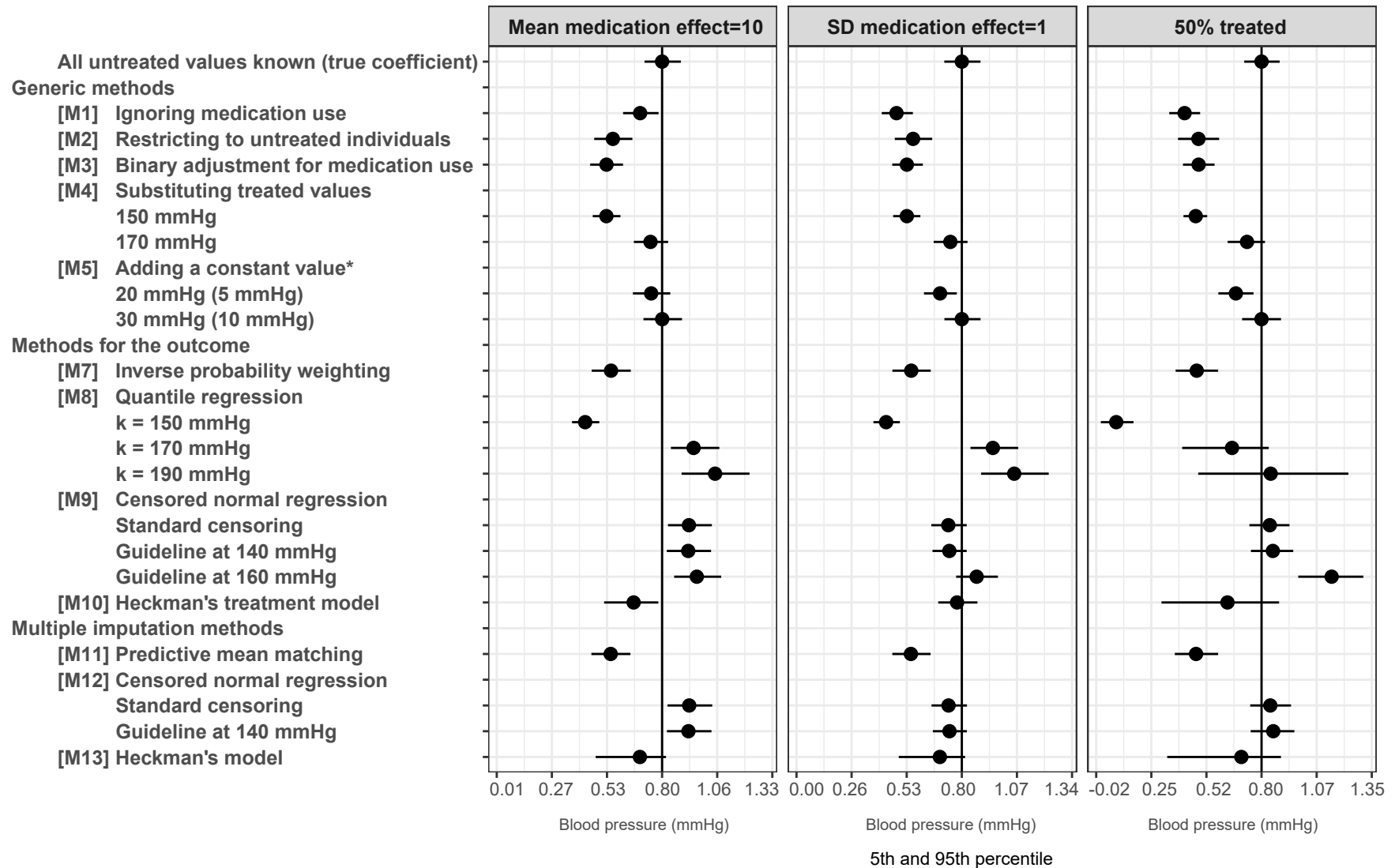
Supplementary Material 4. Regression coefficients and 5th and 95th percentile estimated from modified scenarios of Simulation setting 2, where we estimated the effect of BMI on SBP. One grid unit represents 2.5 standard deviation of the true coefficient, estimated from 1000 simulation runs.
