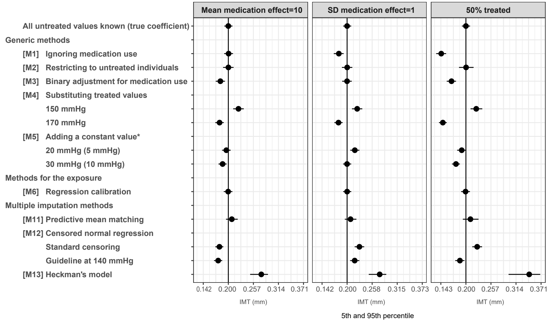
Supplementary Material 3. Regression coefficients and 5th and 95th percentile estimated from modified scenarios of Simulation setting 1, where we estimated the effect of SBP on IMT measurement. One grid unit represents 2.5 standard deviation of the true coefficient, estimated from 1000 simulation runs. * In the scenario where mean medication effect was 10 mmHg, 5 mmHg and 10 mmHg were added.
