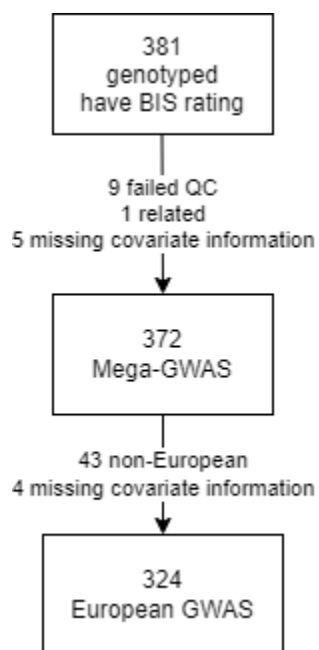
Supplementary Fig. 2. Flowchart of inclusion for the mega-GWAS and the European GWAS. The mega-GWAS includes individuals of all ethnic backgrounds, while the main European GWAS includes those individuals within six standard deviations from the 1000 Genomes-defined European cluster.
