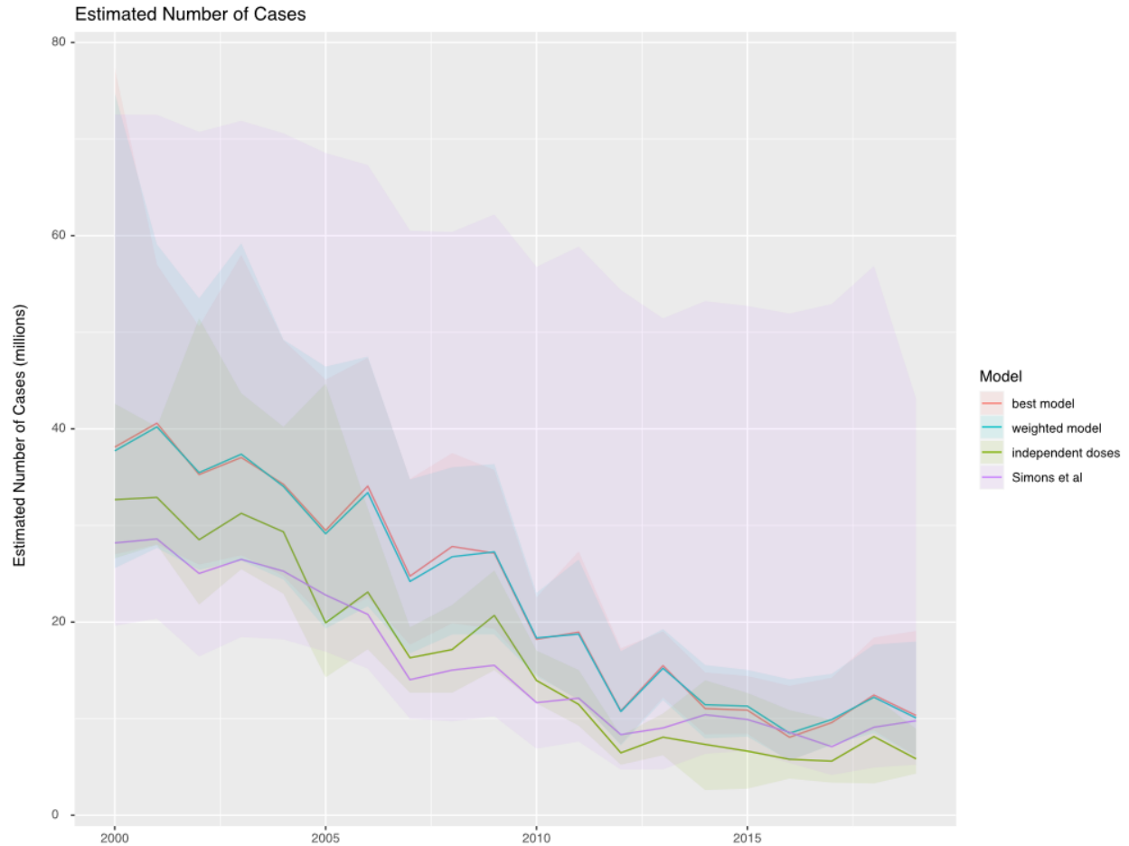
Figure S1. Estimated total burden of measles infection in 193 countries using 4 methods: the country-specific best model (red), the country-specific model-weighted average (blue), the optimistic total assuming independent doses (green), and the Simons et al model (purple). Solid lines indicate the mean estimate and shading indicates the 2.5 th and 97.5 th percentile.
