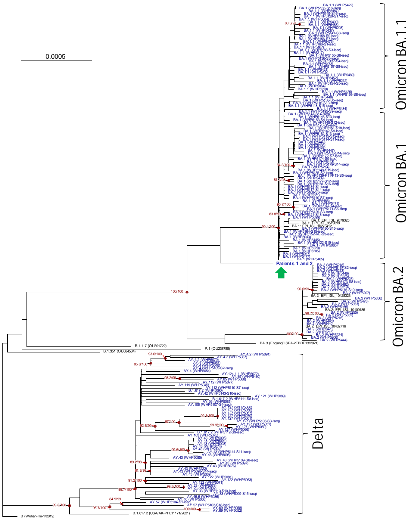
Appendix Figure 2. Phylogeny of SARS-CoV-2 variants identified in incoming travelers. The Maximum likelihood phylogenetic tree was generated using IQ-TREE employing the GTR+F+I nucleotide substitution model with Wuhan-Hu-1 (GenBank: MN908947.3) as the outgroup. Viral genomes generated from this study (blue) and references sequences used in the analysis are shown as indicated. The recombinant virus detected from Patients 1 and 2 is highlighted by an arrow. The red node points show strongly supported branches by SH-aLRT/ultrafast bootstrap. Scale bar indicates estimated genetic distance.
