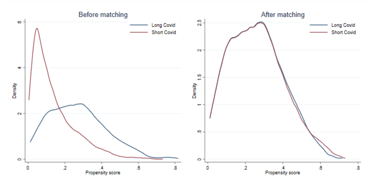
Fig S3. Propensity score density before and after matching
