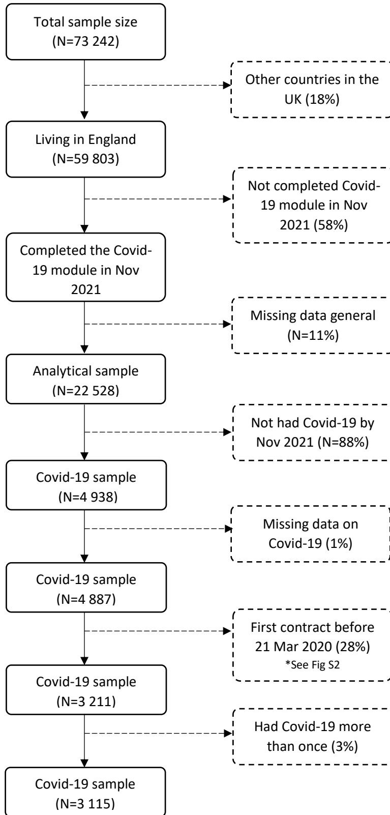
Fig S1. Sample selection process
