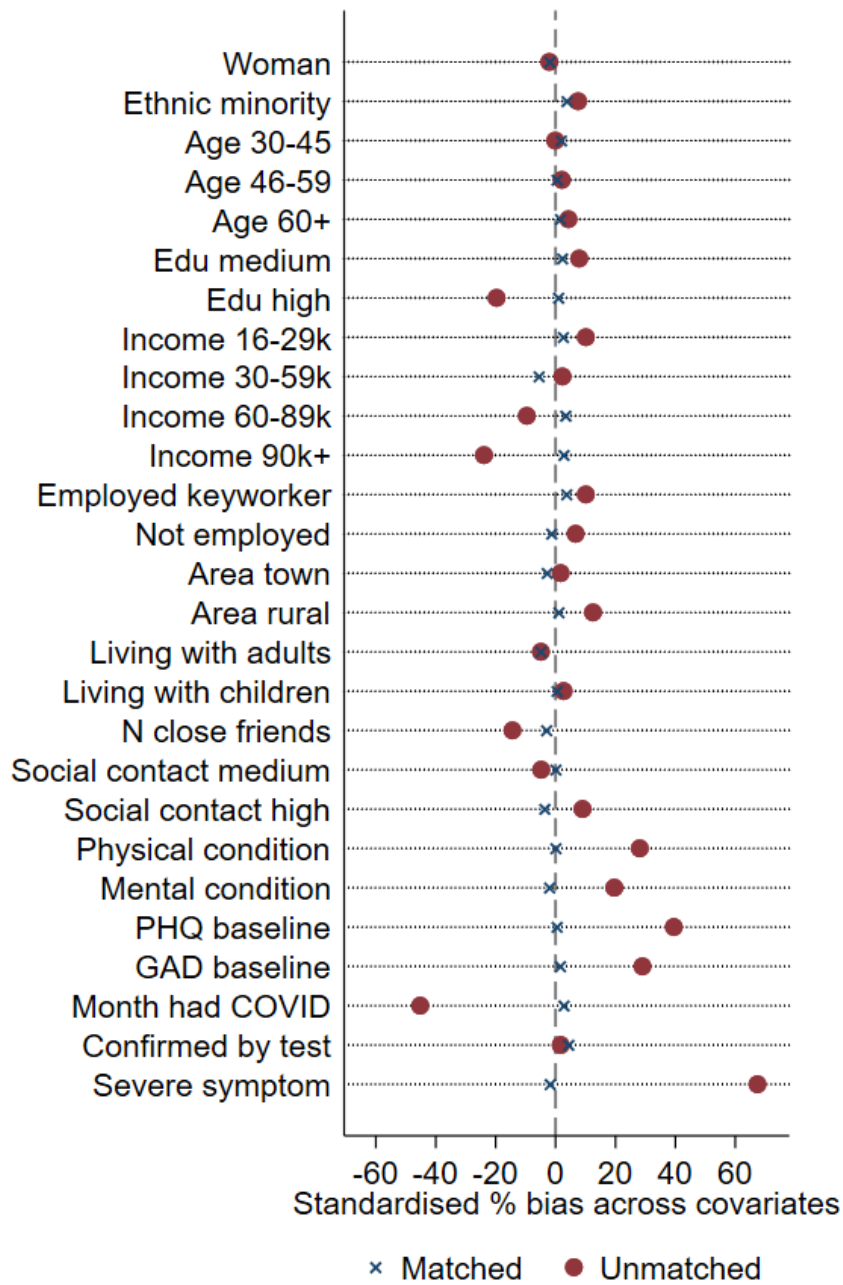
Fig S4. Standardised percentage bias for each covariate before and after matching
