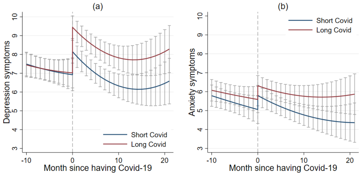
Fig S5. Predicted growth trajectories by Covid-19 group with 95% confidence intervals
