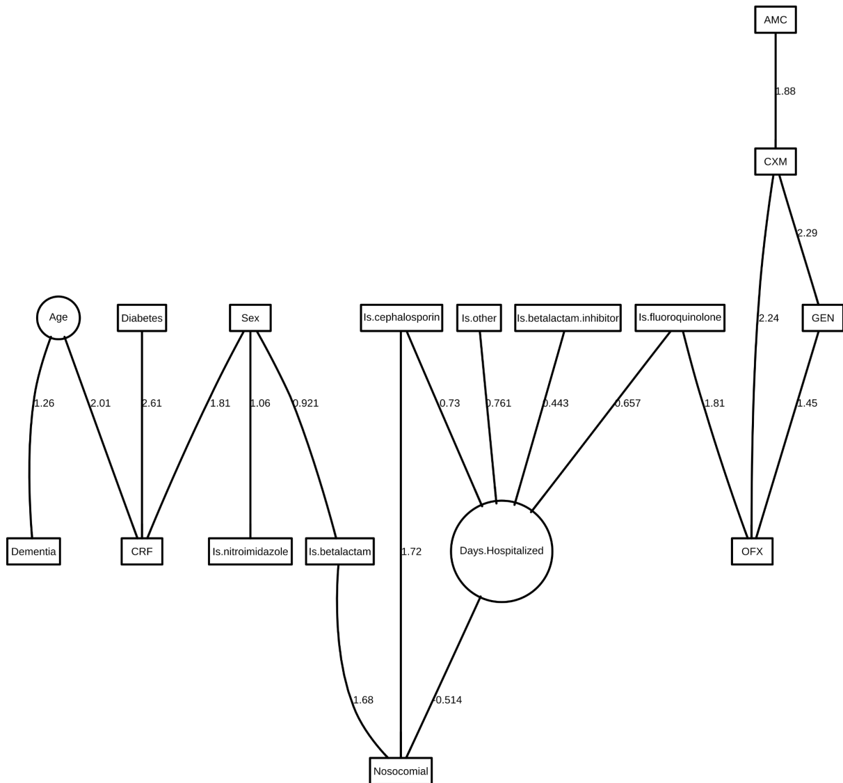
Figure S11: Final DAG for P mirabilis in wound.
