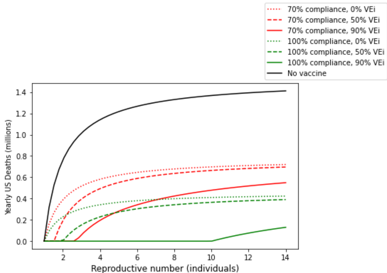
Figure 5. Relationship between R_0 and yearly US deaths is nonlinear. Assuming the duration of natural immunity is 18 months, the IFR is 0.7%, and VE_m is 90%, endemic US COVID-19 death tolls were simulated under a variety of vaccination scenarios.
