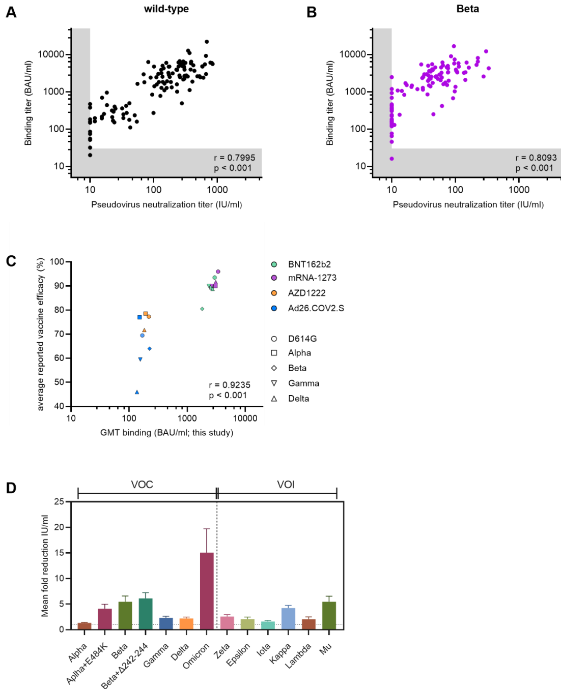
Figure S3: Binding and neutralization post-vaccination titers against VOCs correlated. Correlation between wild-type (A) and Beta (B) binding (BAU/ml) and neutralization titers (IU/ml). Spearman's rank correlation coefficients with p-values are indicated. (C) GMT (BAU/ml) of wild-type and VOCs plotted against the average reported vaccine efficacy against symptomatic infection (Table S4). Vaccine groups are indicated by colors with BNT162b2 in green, mRNA-1273 in purple, AZD1222 in orange and Ad26.COV2.S in blue. Circles represent WT data, squares for Alpha, diamond for Beta, nabla triangle for Gamma and delta triangle for Delta. Spearman's rank correlation coefficients with p-values are indicated. (D) Mean \pm SEM fold reductions in neutralization IC_{50} titers for the serum pools combined against the VOCs and VOIs pseudoviruses in comparison to IC_{50} titers against D614G pseudovirus.
