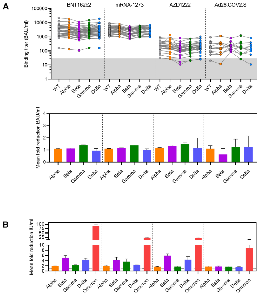
Figure S2: Binding and neutralization titers post-vaccination against the VOCs. (A) Paired binding titers to wild-type and VOCs S protein (BAU/ml) of 1:100,000 diluted sera collected post complete vaccination for the four vaccination groups (upper plot). The lower cut-off for binding was set at a 30 BAU/ml (grey shading). Mean \pm SEM fold reductions in binding titers against the VOCs in comparison to wild-type (lower plot). (B) Mean \pm SEM fold reductions in neutralization IC 50 titers against the VOCs pseudoviruses in comparison to neutralization IC 50 titers against D614G pseudovirus.
