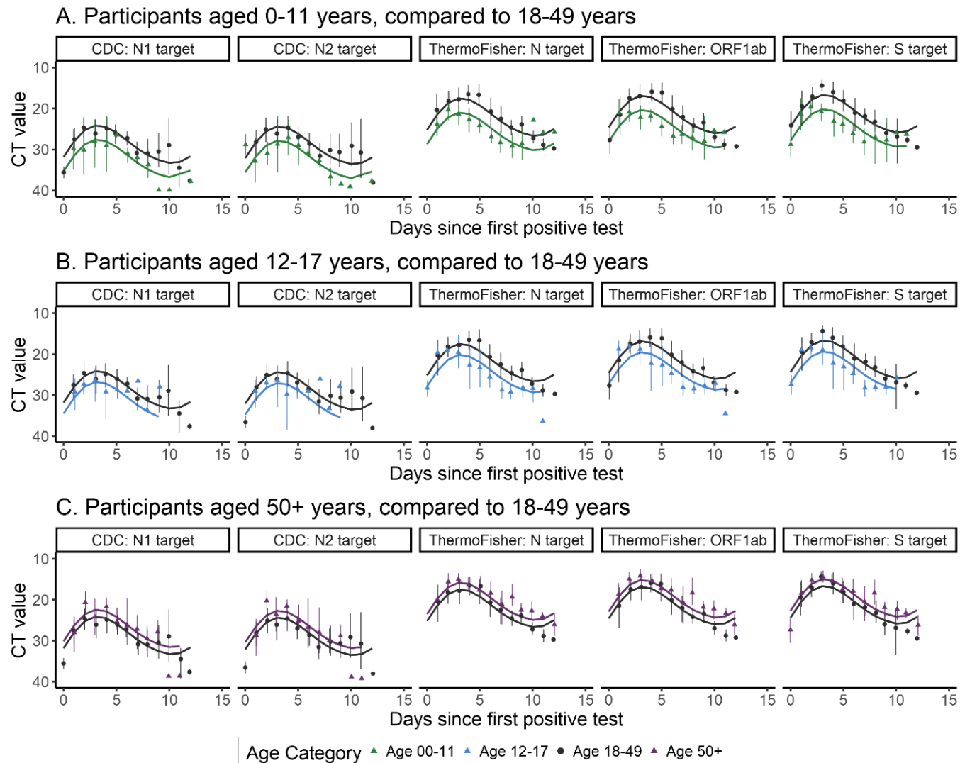
Figure 1. Ct value curves over time since each participant first tested positive against each target, within age groups
