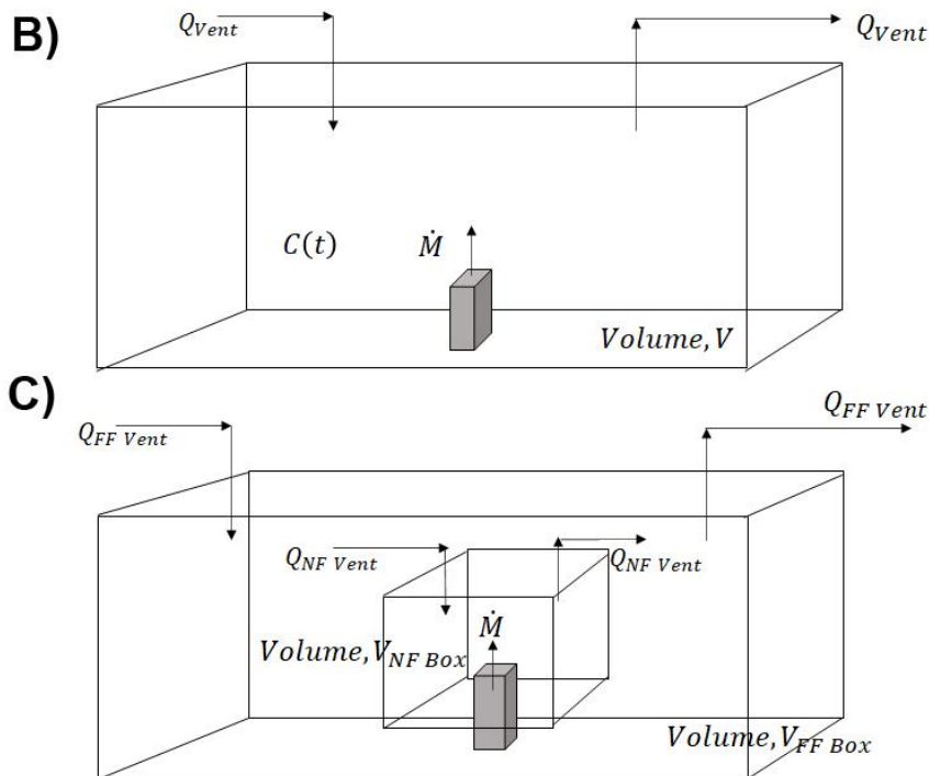
Figure S1. The different box models for CEAT. A) Factors Included in COVID-19 Exposure Assessment Tool Interface (CEAT). A summary of the factors and mechanisms affecting the comparative dose and exposure risks. B) Single Zone Well-Mixed Box Model. Basic box model assumes emissions are instantaneously well mixed. C) Near Field (NF) and Far Field (FF) Box Model. “Box-within-a-box” approach provides localized higher concentration in the vicinity of the source.
