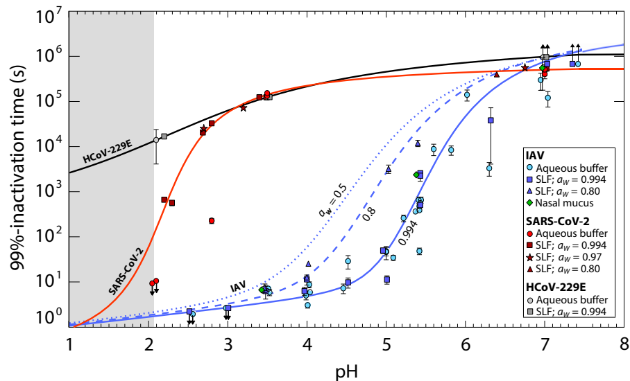
Figure 1. Time required for 99% titer reduction of influenza A virus (IAV), SARS-CoV-2 and human coronavirus HCoV-229E measured in various bulk media ( > 10 \mu\text{l} ) at 22^\circ\text{C} . Data points represent inactivation times in aqueous citric acid/ \text{Na}_2\text{HPO}_4 buffer, synthetic lung fluid (SLF) or nasal mucus with pH between 7.4 and 2. SLF concentrations correspond to water activity a_w = 0.994 ( 1\times SLF; squares), a_w = 0.97 ( 5\times SLF; stars) and a_w = 0.8 ( 18\times SLF; triangles); buffer (circles) and nasal mucus (diamonds) correspond to a_w \sim 0.99 . Each experimental condition was tested in replicate with error bars indicating 95% confidence intervals. While IAV displays a pronounced reduction in infectivity around pH 5, SARS-CoV-2 develops a similar reduction only close to pH 2, and HCoV-229E is largely pH-insensitive. Solid lines are arctan fits to SLF data with a_w = 0.994 (blue: IAV; red: SARS-CoV-2; black: HCoV-229E). The dashed line is an arctan fit to the SLF data with a_w = 0.80 . The dotted line is an extrapolation to a_w = 0.5 ( 24\times SLF). Upward arrows indicate insignificant change in titer over the course of the experiment, and downward arrows indicate inactivation below the level of detection at all measured times. The fitted curves below pH 2 (grey shaded area) are extrapolated with high uncertainty. Examples of measured inactivation curves are shown in Fig. S1. The arctan fit equations, which are also used for the model simulations, are given by Eqns. S28, S29, and S30.
