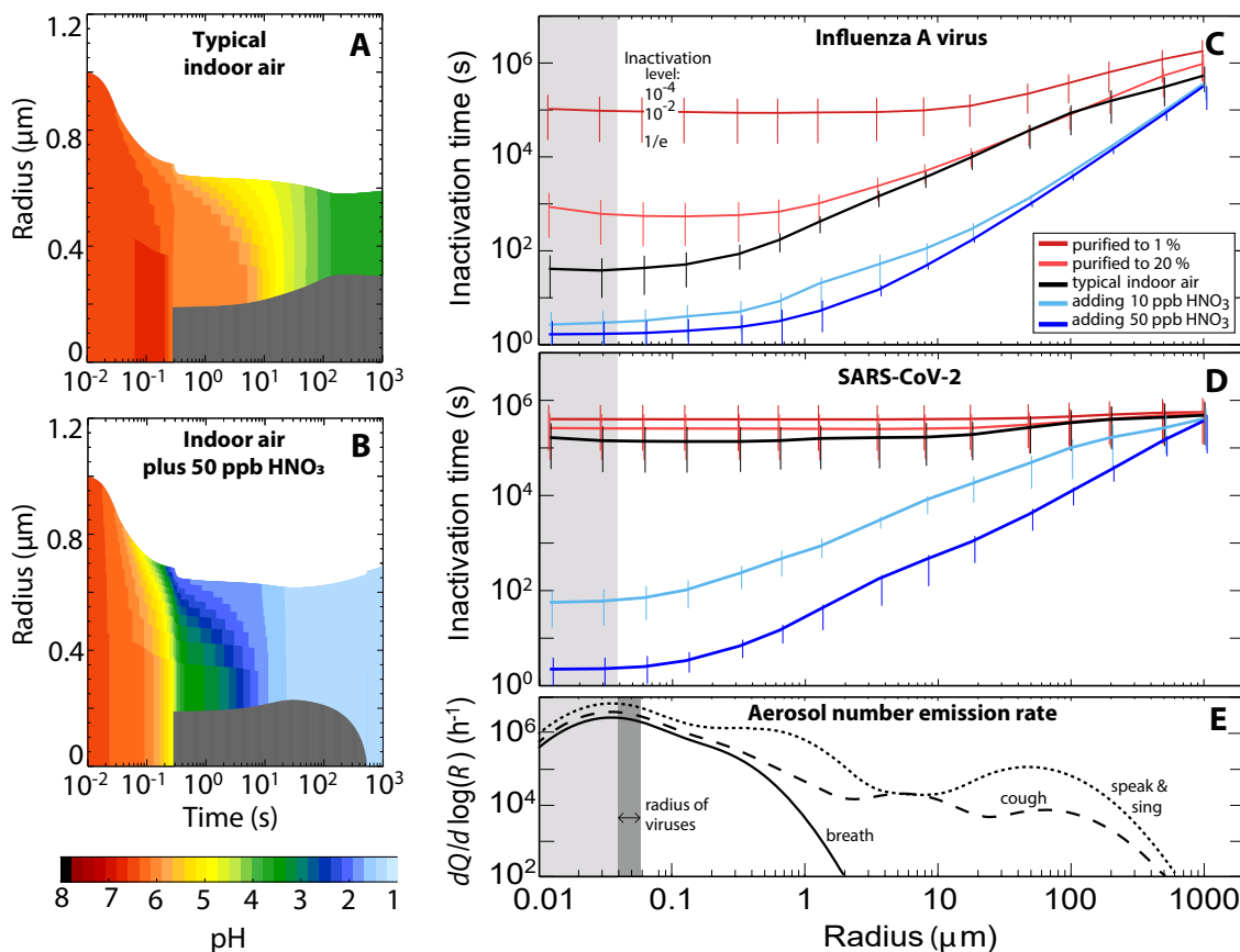
Figure 4. Impact of nitric acid vapor (HNO 3 ) in indoor air on virus inactivation in expiratory particles. (A) Modeled pH value in an expiratory particle with properties of synthetic lung fluid with initially 1 μm radius in indoor air (20°C, 50% RH) of typical composition (identical to 3F, but with different color scale). (B) Same, but in indoor air enriched with 50 ppb HNO 3 , reducing the time to reach pH 4 from 2 minutes to less than 2 seconds. (C and D) Inactivation times of IAV and SARS-CoV-2 as function of particle radius under various conditions: indoor air with typical composition (black), enriched with 10 or 50 ppb HNO 3 (blue), or purified air with HNO 3 and NH 3 reduced to 20% or 1% (red). Whiskers show reductions of virus load to 10 -4 (upper end), 10 -2 (intersection with line) and 1/e (lower end). The exhaled air mixes with the indoor air by turbulent eddy diffusion (see Fig. 3). For sensitivity tests see Figs. S11B and S12B. The gas phase compositions of exhaled air and the various cases of indoor air are defined in Table S4. (E) Mean size distribution (35) of number emission rates of expiratory aerosol particles ( dQ/d\log(R) ) for breathing (solid line), speaking and singing (dotted line) and coughing (dashed line). Dark grey range indicates virus radii. Light grey shading shows conditions for particles smaller than a virus, referring to an equivalent coating volume with inactivation times indicated. (Radius values in (C)-(E) refer to the particle size 1 s after exhalation.)
