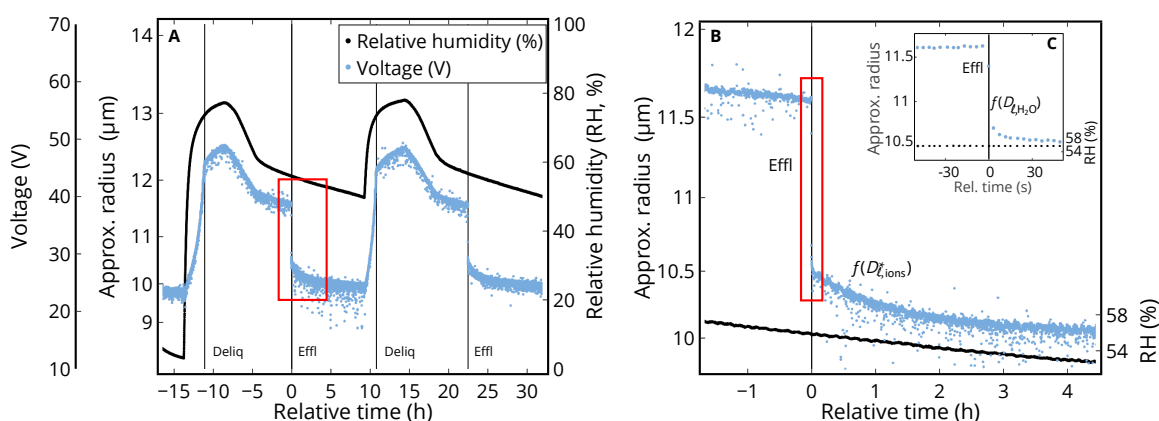
Figure 2. Measured hygroscopicity cycles of a synthetic lung fluid (SLF) particle in an electrodynamic balance (EDB) forced by prescribed changes in relative humidity (RH). The voltage required to balance the particle in the EDB against gravitational settling and aerodynamic forces is a measure of the particle's mass-to-charge ratio, allowing the particle radius R to be estimated. (A) Two humidification cycles of an SLF particle with a dry radius R_0 \sim 9.7 \mu\text{m} . The experiment spanned about 2 days with slow humidity changes, allowing the thermodynamic and kinetic properties of SLF to be determined. Deliquescence/efflorescence points are marked by "Deliq/Effl". (B) Zoom on the drying phase (red box in (A)) with salts in the droplet (mainly NaCl) efflorescing around 56% RH (black line): very fast initial crystal growth ( < 10 \text{ s} ) with rapid loss of \text{H}_2\text{O} from the particle, followed by slow further crystal growth (1 h). The latter is caused by the abrupt switch from \text{H}_2\text{O} diffusion to the diffusion of \text{Na}^+ and \text{Cl}^- ions through the viscous liquid, resulting in an ion diffusion coefficient of D_{l,ions}^* \approx 10^{-10} \text{ cm}^2/\text{s} . The insert (C) highlights the minute before and after efflorescence, which allows a lower bound of the \text{H}_2\text{O} diffusivity (namely D_{l,H_2O} > 10^{-7} \text{ cm}^2/\text{s} ) to be determined.
