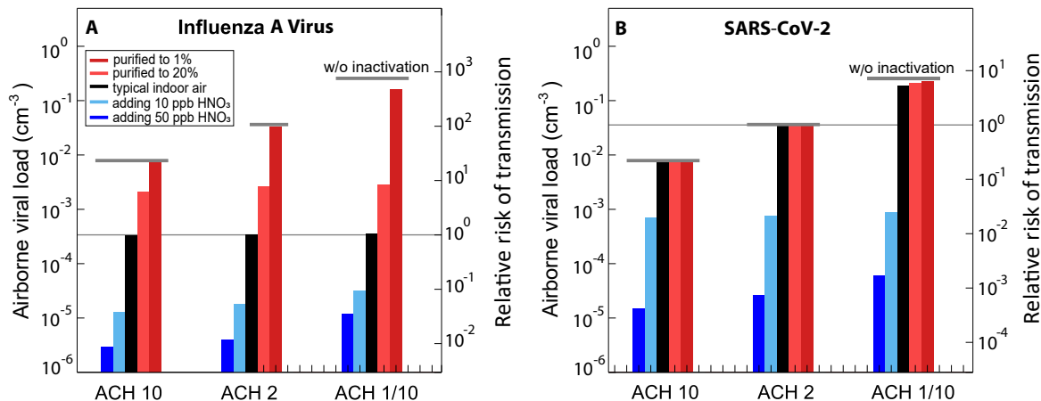
Figure 5. Airborne viral load (# viruses per volume of air) and relative risk of transmission of (A) IAV and (B) SARS-CoV-2 infection in a room subject to various air treatments, such as addition of HNO 3 or supply of purified air with different ventilation rates, Air Changes per Hour (ACH). The room is assumed to accommodate one infected person per 10 m 3 of air volume, emitting virus-laden aerosol by normal breathing (solid curve in Figure 4E), and assuming one infectious virus per aerosol particle. (Corresponding plots assuming a virus concentration that is proportional to the size of the aerosol particles are shown in Fig. S16.) Steady state virus loading, i.e. number of infectious viruses per cubic centimeter of air (left axes), is calculated as the balance of exhaled viruses and their removal by ventilation, deposition, and inactivation. Results are shown for three different ventilation strengths. Virus inactivation is calculated according to Figure 4C-D, starting from radius 0.05 μm. Note, that the mixing speed of the exhalation plume with indoor air depends on ACH (following (32), see Supplementary Text). Right axes show the transmission risk under these treatments relative to the risk in a room with typical indoor air (see Table S4) and ACH 2 (thin horizontal line). Typical indoor air is shown by black bars, filtered air with removal of trace gases to 20% and 1% by red bars, and air enriched with 10 or 50 ppb HNO 3 by blue bars. Thick grey horizontal lines indicate the viral load and relative transmission risk in the absence of any inactivation. Results for 2 and 5 ppb HNO 3 are shown in Fig. S17. Results for HCoV-229E, along with analogous analyses for coughing and speaking/singing are shown in Fig. S15.
