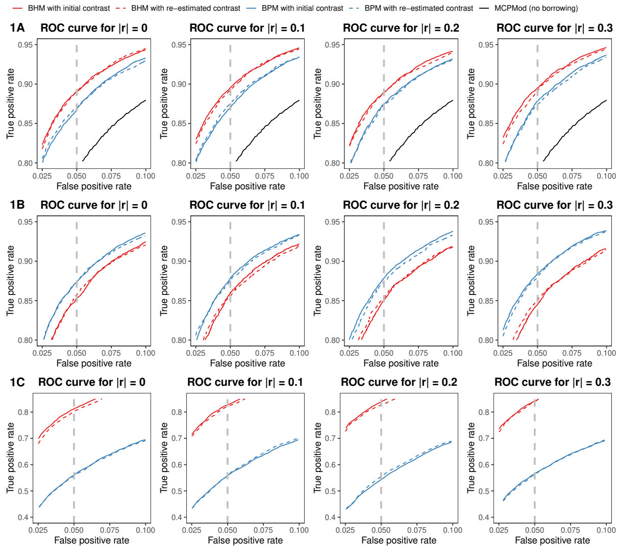
Figure 2: The ROC curves of MCPMod, Bayesian pooling model (BPM) and Bayesian hierarchical model(BHM) with four different levels of prognostic heterogeneity for scenario 1. The dashed grey line denotes 5% false positive rate, i.e., 5% type I error rate.
