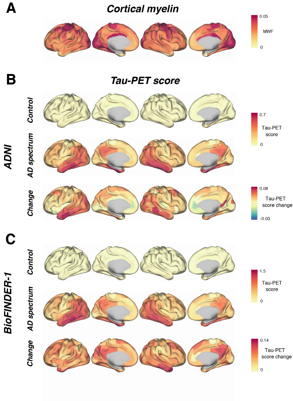
Supplementary figure 1: Brain renderings of cortical myelin within the MWF template and tau-PET scores among controls and AD participants.
