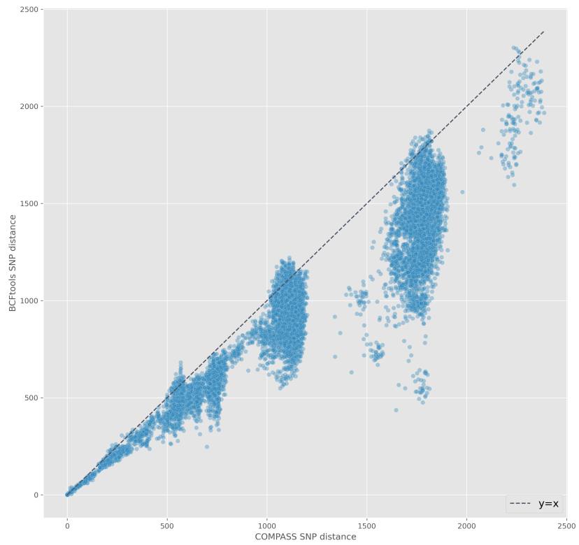
Figure S2: Pairwise SNP distance relationship between Illumina (COMPASS; x-axis) and Nanopore (bcftools; y-axis). Each point represents the SNP distance between two isolates. The black, dashed line shows the identity line (i.e. y = x ).
