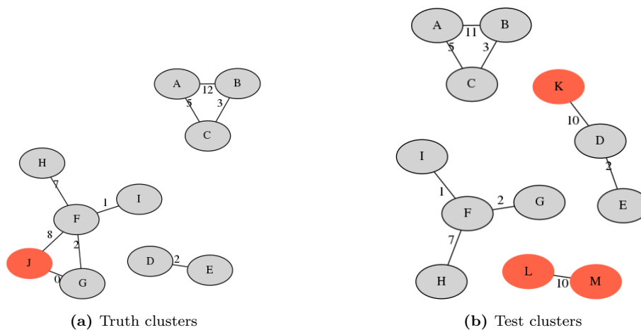
Figure S1: Illustrative examples of transmission clustering. a) represents truth clusters, while b) is clustering from some “test” method we would like to compare to a) . The nodes represent samples with the numbers on the edges connecting them indicating the distance between those two samples. The red nodes indicate samples with a clustering disparity between the two clusterings. Note, we do not show singletons (disconnected nodes) - e.g., J is missing from (b) .
