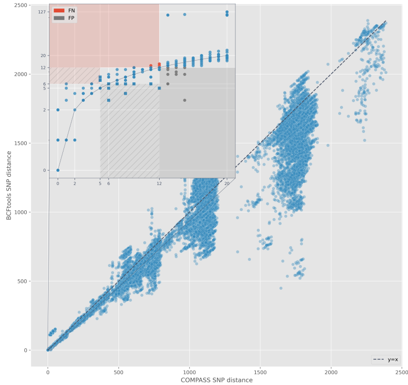
Figure S5: Pairwise SNP distance relationship between Illumina (COMPASS; x-axis) and mixed COMPASS-bcftools calls (y-axis). Each point represents the SNP distance between two isolates. The black, dashed line shows the identity line (i.e., y=x ). The zoomed inset shows all pairs where the COMPASS distance is \leq 20 . The red area and points indicate pairs with a mixed distance \geq 12 , but an Illumina distance \leq 12 . These pairs are deemed false negative (FN) connections. The red area with stripes indicates pairs that are FN connections at an Illumina threshold of 5 (mixed threshold 6), but not when the threshold is expanded to 12. These pairs are shown as square points. The grey area and points is the inverse - i.e., false positive (FP) connections. Note, the y-axis in the inset window is log-scaled.
