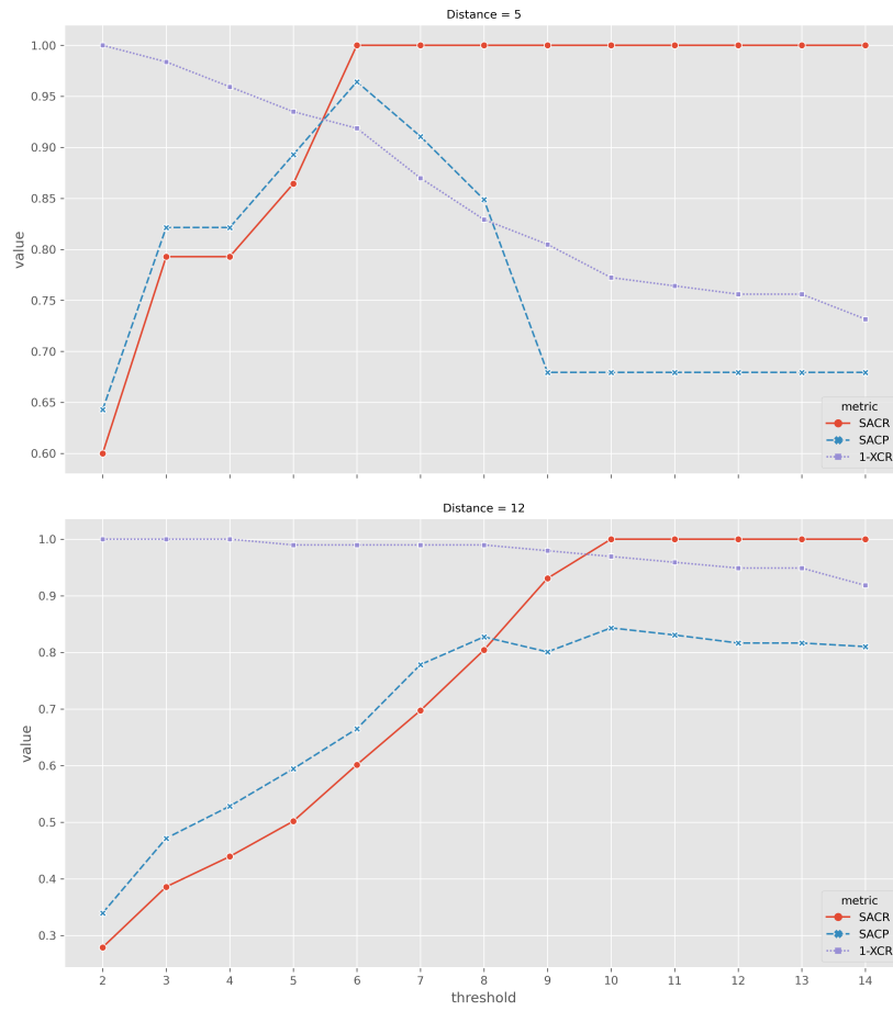
Figure S3: Illumina and Nanopore ( bcftools ) transmission cluster similarity for various SNP distance threshold. Each subplot compares the Nanopore clustering for the threshold on the x-axis to the Illumina clustering based on the distance (threshold) in the subplot title. SACR (red), SACP (blue), and 1-XCR are represented by the solid, dashed, and dotted lines, respectively. SACR=sample-averaged cluster recall; SACP=sample-averaged cluster precision; XCR=excess clustering rate.
