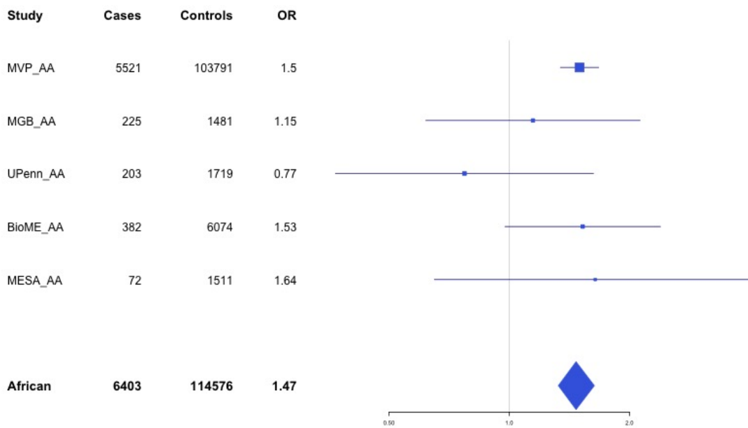
Supplementary Figure 4.3 – rs529326506 (chr3:90503764) in locus 26 (EPA3;NONE)
