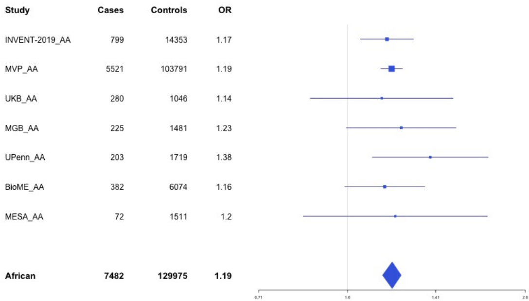
Supplementary Figure 4.5 – rs2066864 (chr4:155525695) in locus 39 (FGG)
