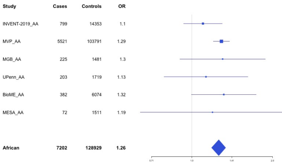
Supplementary Figure 4.8 – rs57950734 (chr12:6145649) in locus 87 (VWF)
