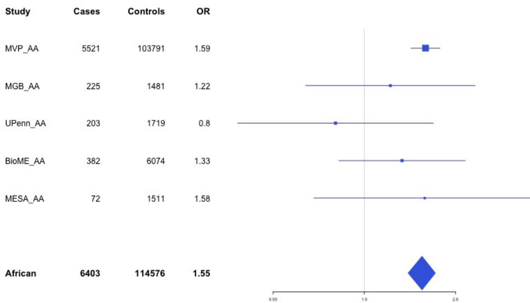
Supplementary Figure 4.4 – rs80133433 (chr3:93791551) in locus 27 (NSUN3)
