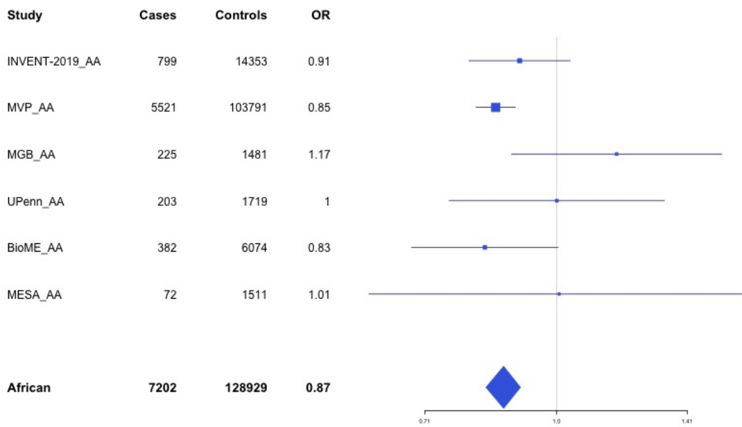
Supplementary Figure 4.13 – rs73174952 (chr22:43111733) in locus 130 (A4GALT)
