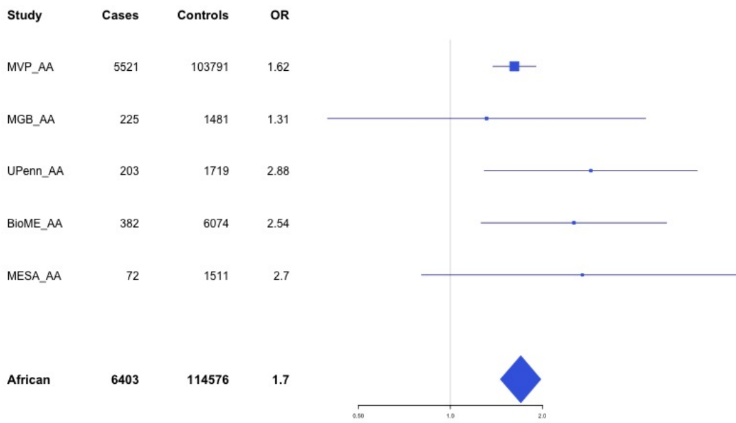
Supplementary Figure 4.1 – rs10800427 (chr1:169272451) in locus 9 (NME7)
