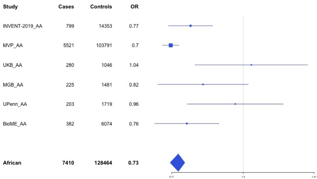
Supplementary Figure 4.7 – rs8176719 (chr9:136132908) in locus 66 (ABO)
