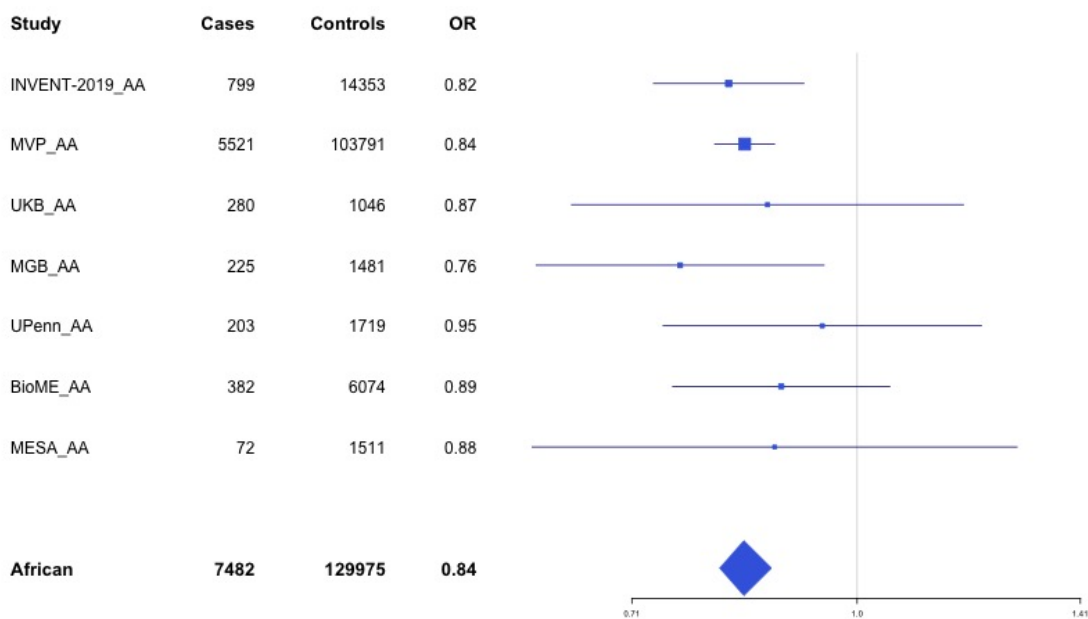
Supplementary Figure 4.6 – rs56810541 (chr4:187200550) in locus 40 (F11)
