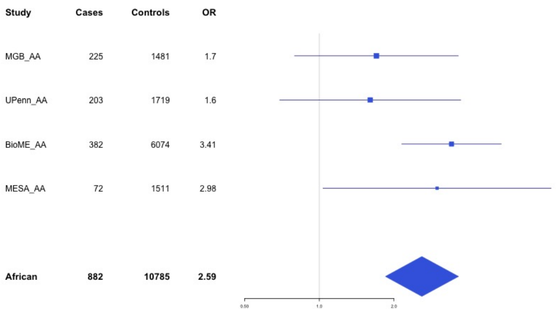
Supplementary Figure 4.12 – rs114102448 (chr21:47523605) in locus 128 (COL6A2)
