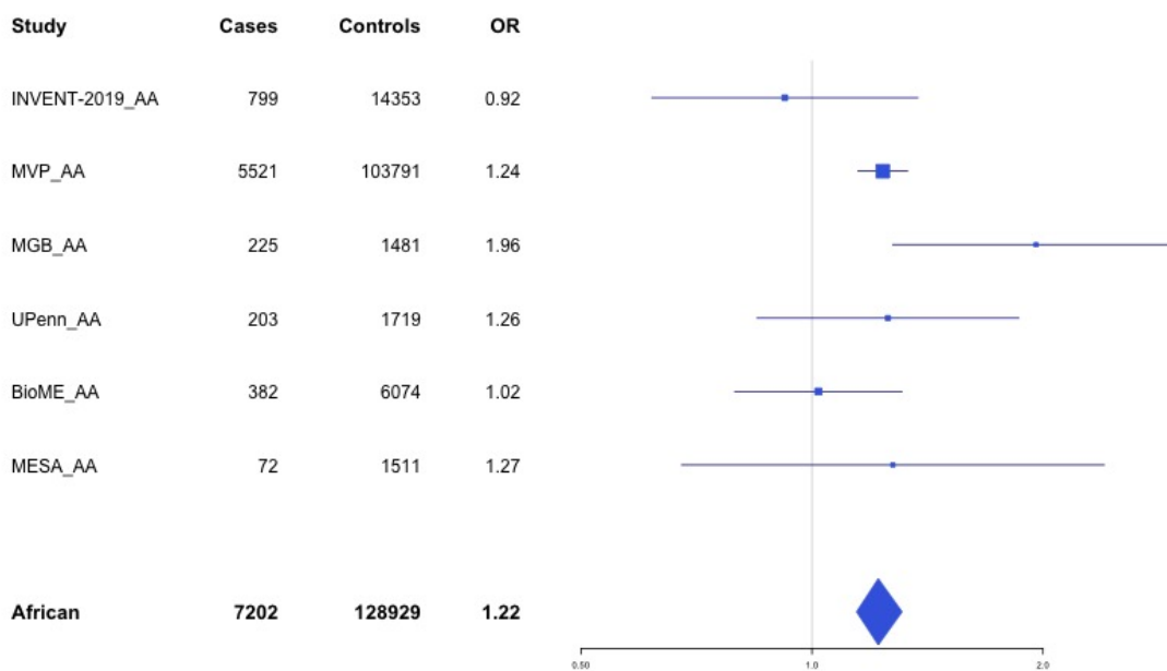
Supplementary Figure 4.10 – rs13306849 (chr20:23030199) in locus 126 (THBD)
