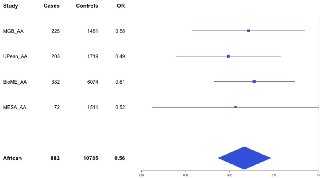
Supplementary Figure 4.9 – rs76668186 (chr16:6686083) in locus 104 (RBFOX1)
