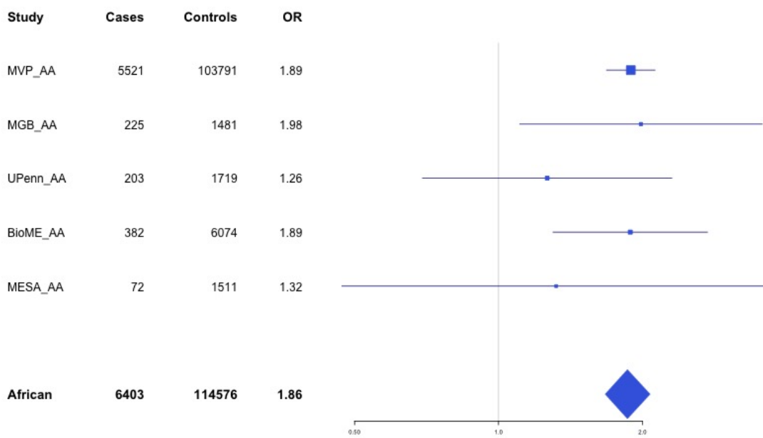
Supplementary Figure 4.2 – rs182293241 (chr2:128029746) in locus 18 (ERCC3)
