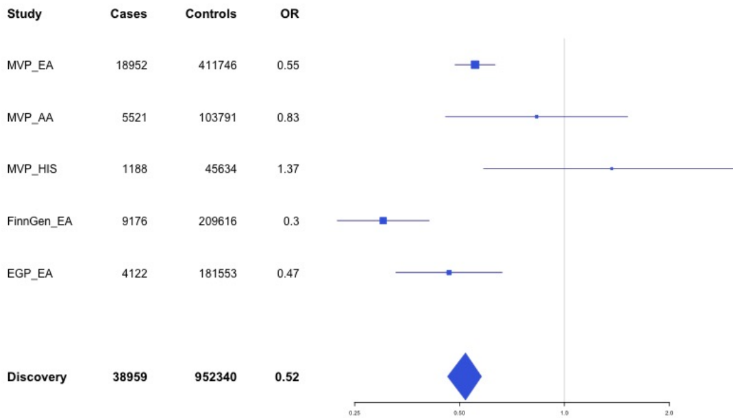
Supplementary Figure 1.49 – rs141687379 (chr11:56666822) in locus 80 (FADS2B)
