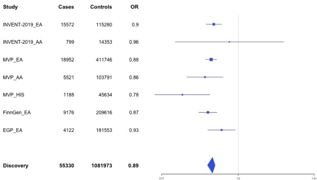
Supplementary Figure 1.72 – rs8110055 (chr19:10739143) in locus 119 (SLC44A2)
