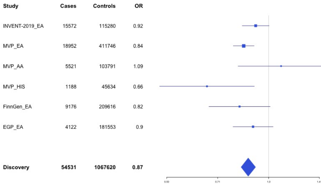
Supplementary Figure 1.61 – rs55707100 (chr15:43820717) in locus 100 (MAP1A)
