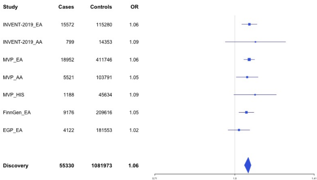
Supplementary Figure 1.64 – rs12443808 (chr16:30996871) in locus 106 (HSD3B7)
