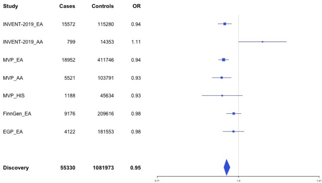
Supplementary Figure 1.31 – rs9390460 (chr6:147694334) in locus 52 (STXBP5)
