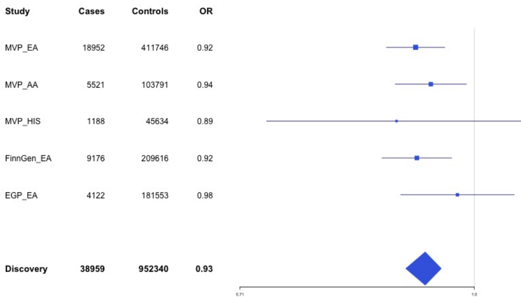
Supplementary Figure 1.70 – rs142140545 (chr17:64191540) in locus 116 (CEP112;APOH)
