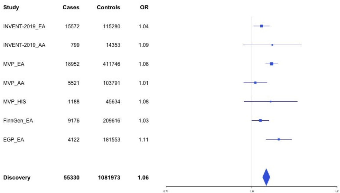
Supplementary Figure 1.36 – rs2685417 (chr8:27807434) in locus 60 (SCARA5)
