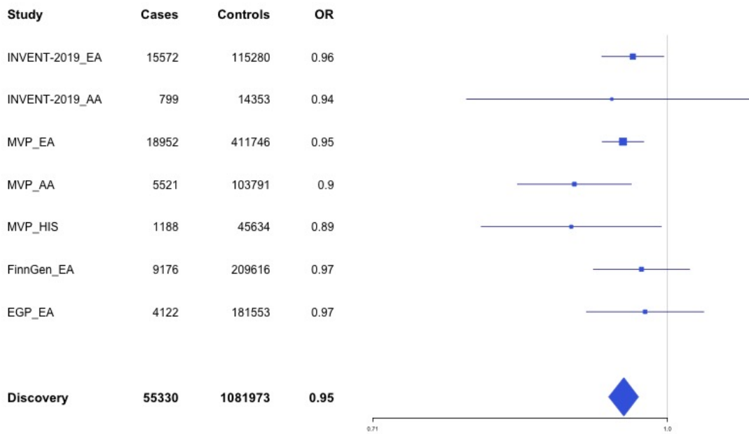
Supplementary Figure 1.69 – rs62054822 (chr17:43927708) in locus 115 (MAPT-AS1)
