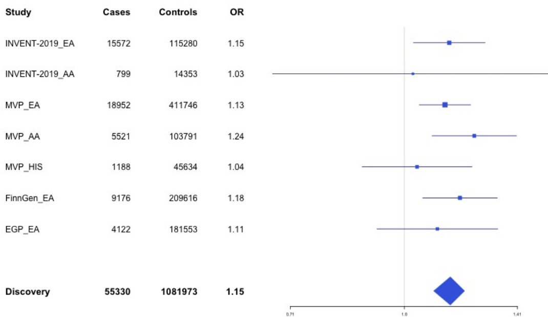
Supplementary Figure 1.44 – rs16937003 (chr10:80938499) in locus 73 (ZMIZ1)
