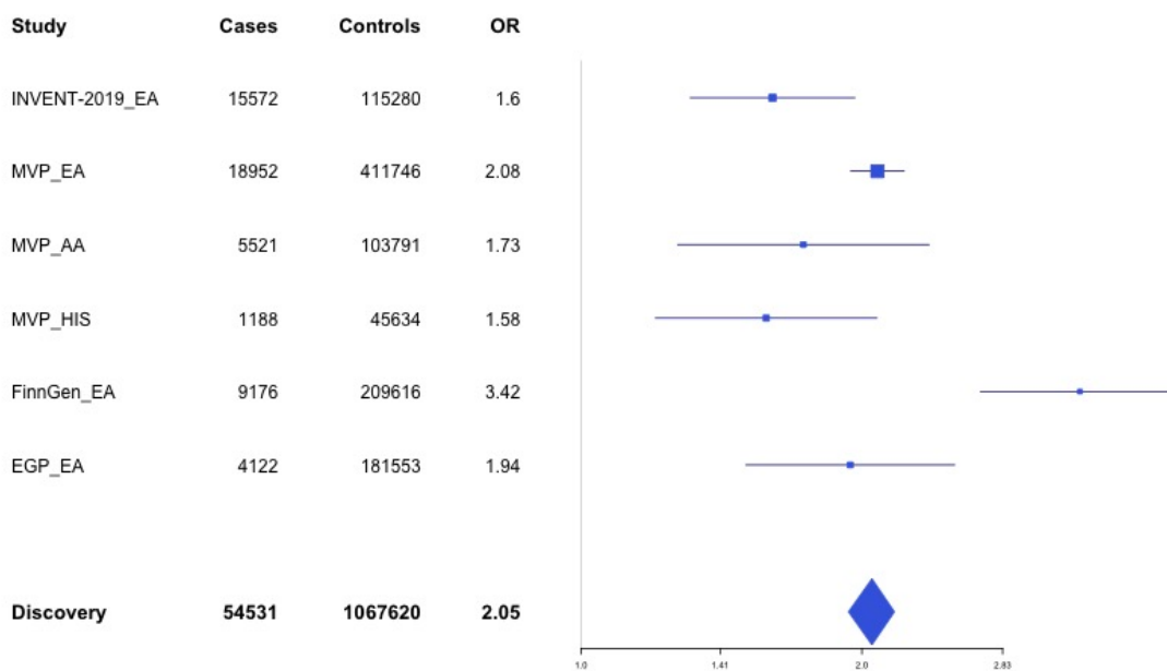
Supplementary Figure 1.48 – rs1799963 (chr11:46761055) in locus 79 (F2)
