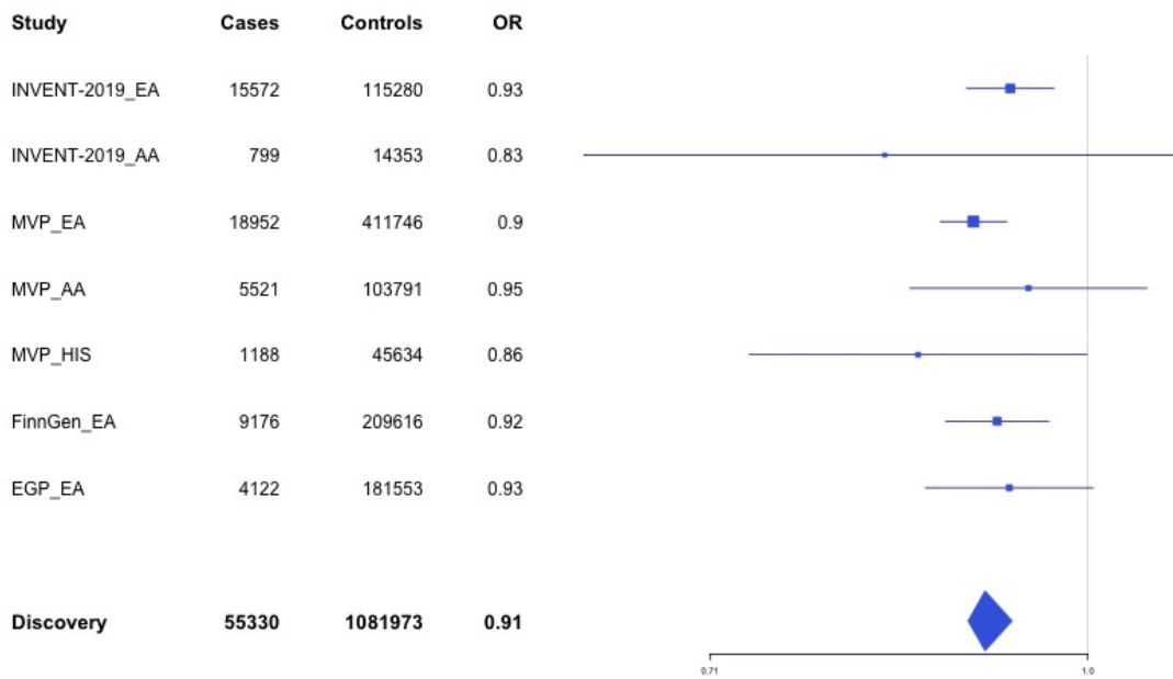
Supplementary Figure 1.75 – rs1654425 (chr19:55538980) in locus 124 (GP6)
