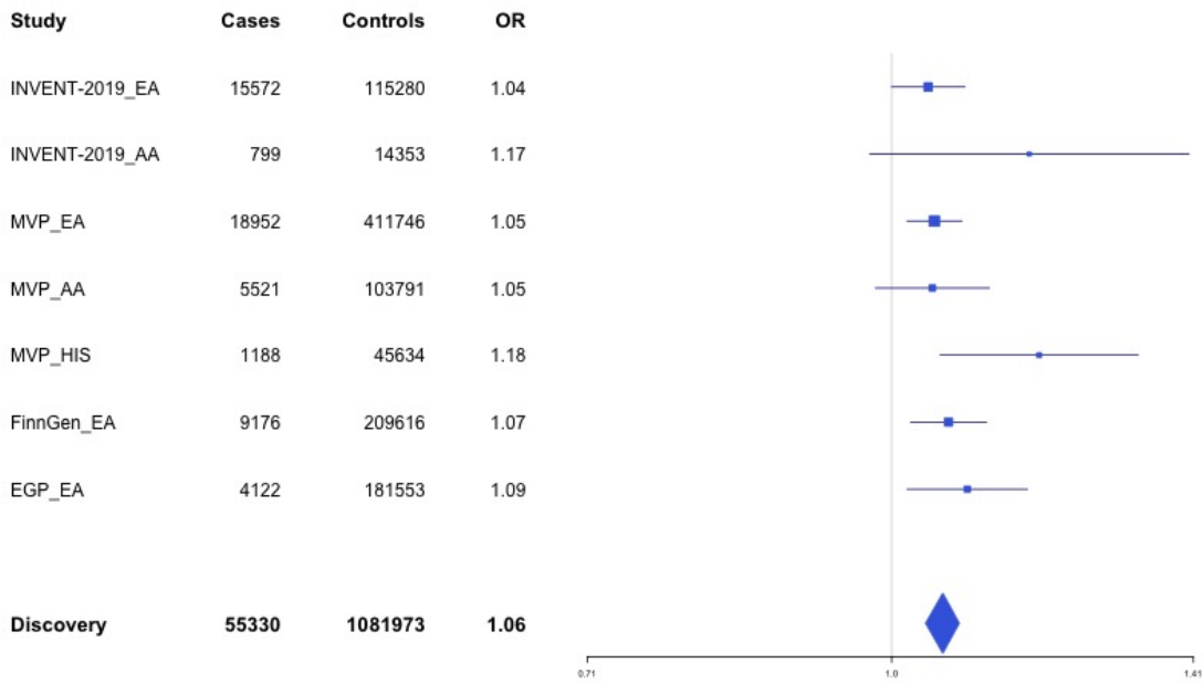
Supplementary Figure 1.23 – rs17010957 (chr4:86719165) in locus 37 (ARHGAP24)
