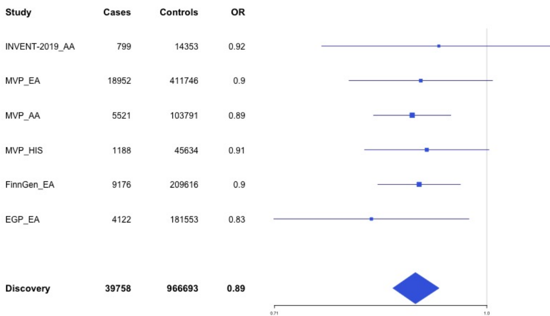
Supplementary Figure 1.76 – rs2631628 (chr19:56645250) in locus 125 (ZNF787;ZNF444)
