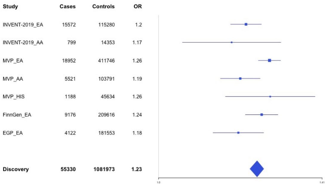
Supplementary Figure 1.24 – rs2066864 (chr4:155525695) in locus 39 (FGG)
