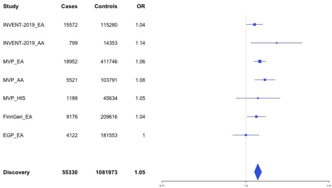
Supplementary Figure 1.2 – rs3767812 (chr1:118155620) in locus 5 (TENT5C)
