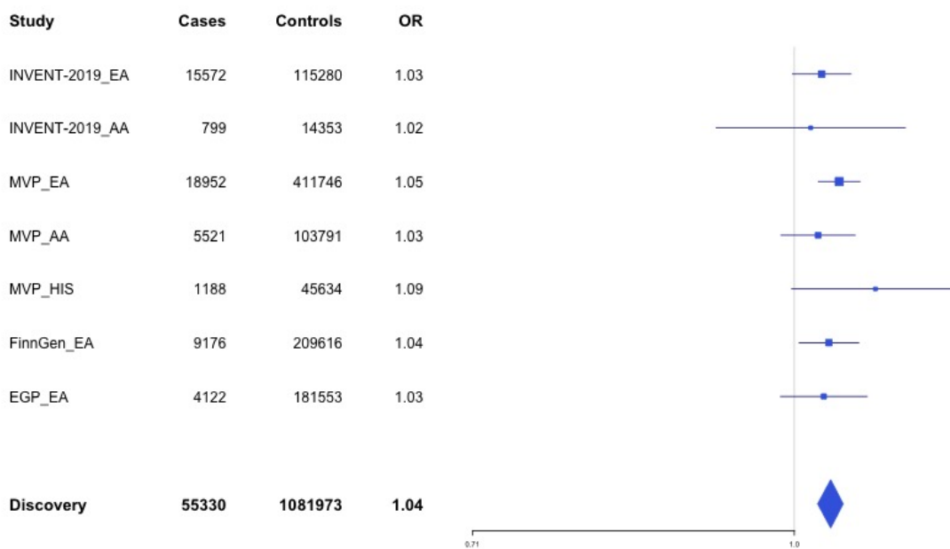
Supplementary Figure 1.12 – rs2960420 (chr3:12314512) in locus 23 (SYN2;PPARG)
