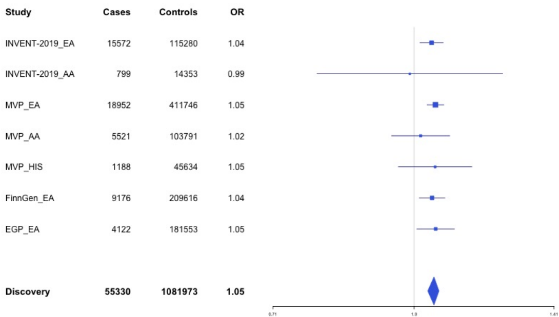
Supplementary Figure 1.56 – rs3184504 (chr12:111884608) in locus 91 (SH2B3)
