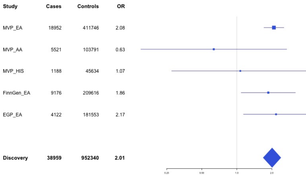
Supplementary Figure 1.15 – rs562281690 (chr3:90177913) in locus 26 (EPHA3;NONE)
