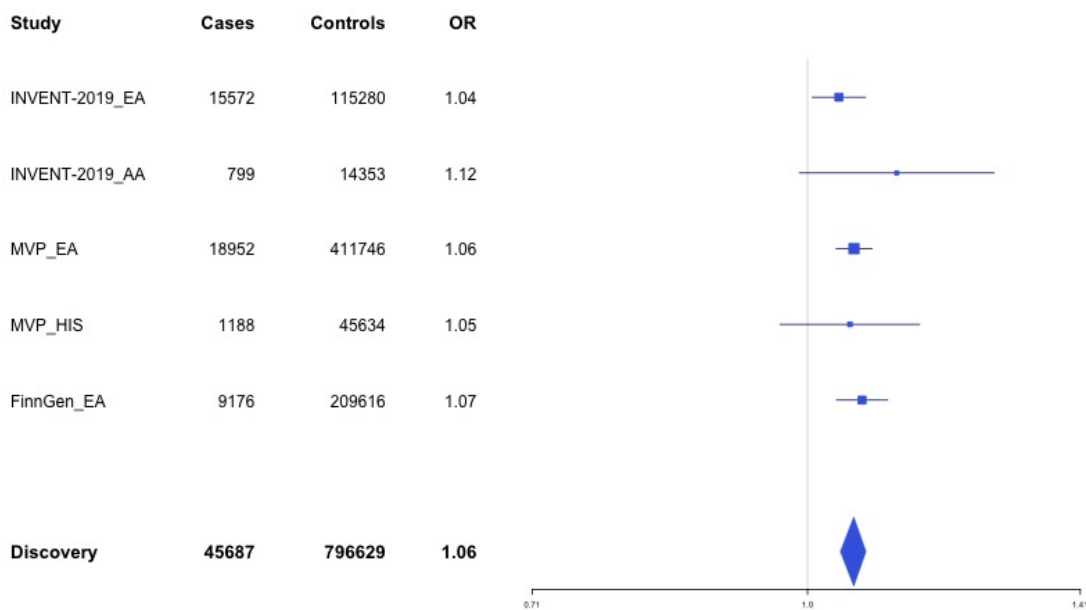
Supplementary Figure 1.66 – rs28634651 (chr16:88553198) in locus 111 (ZFPM1)
