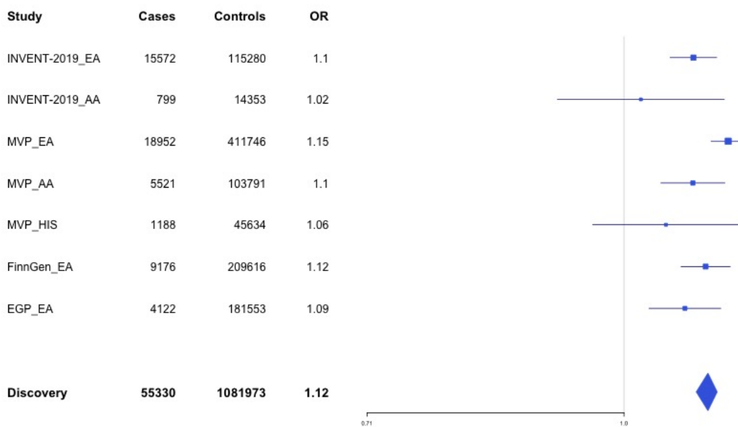
Supplementary Figure 1.78 – rs6060288 (chr20:33772243) in locus 127 (MMP24-AS1-EDEM2)
