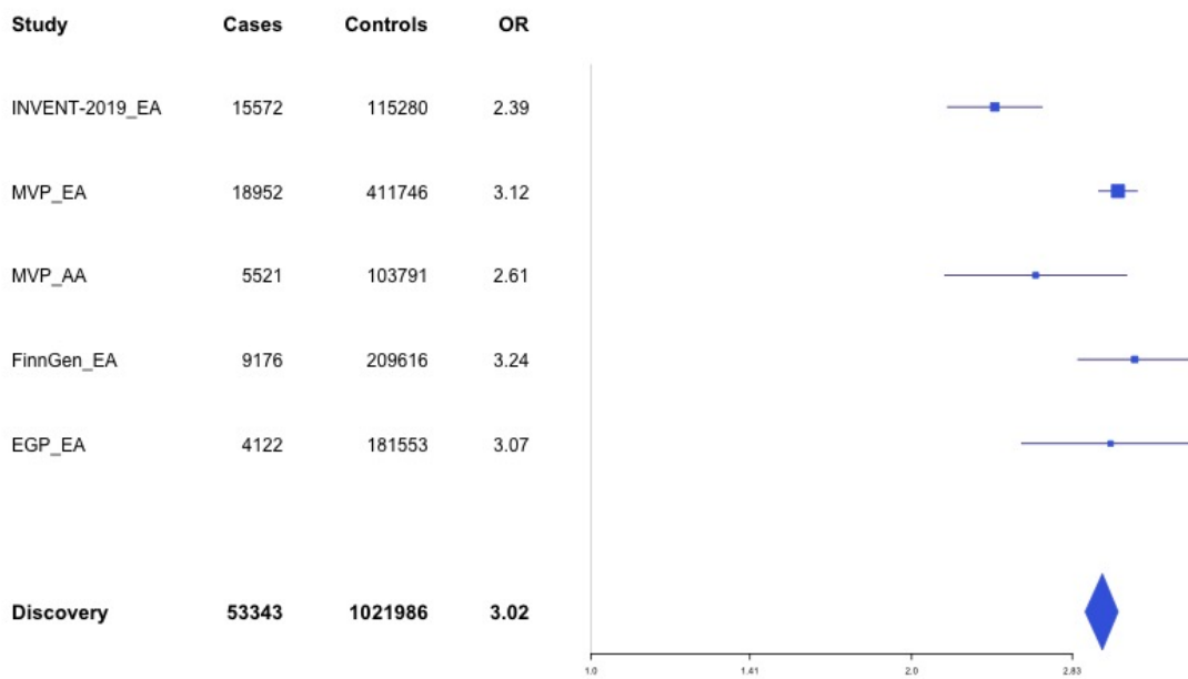
Supplementary Figure 1.3 – rs6025 (chr1:169519049) in locus 9 (F5)
