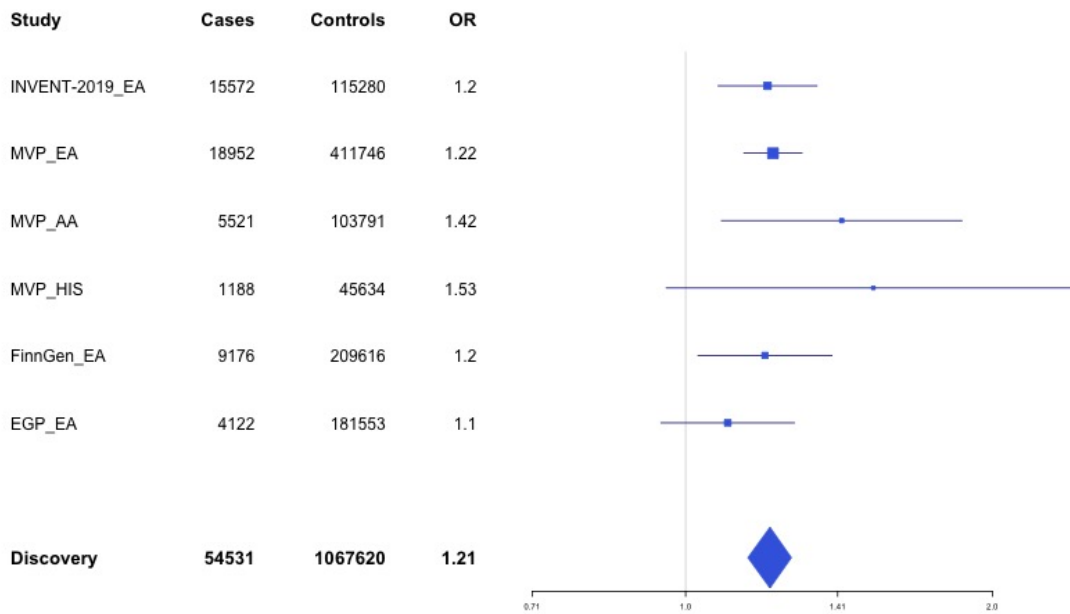
Supplementary Figure 1.51 – rs35257264 (chr11:126296816) in locus 85 (ST3GAL4)
