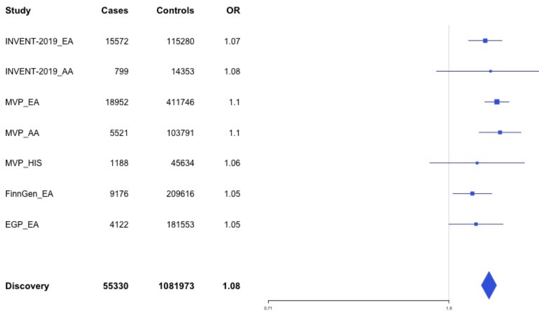
Supplementary Figure 1.37 – rs6993770 (chr8:106581528) in locus 62 (ZFPM2)
