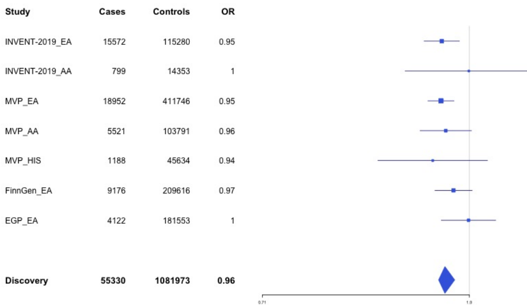
Supplementary Figure 1.68 – rs7225756 (chr17:6893691) in locus 113 (ALOX12-AS1)
