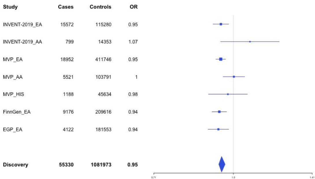
Supplementary Figure 1.58 – rs3211752 (chr13:113787459) in locus 94 (F10)
