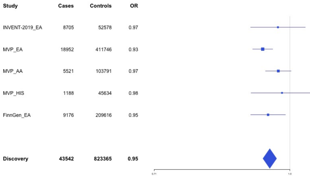
Supplementary Figure 1.81 – rs34609587 (chr23:11657363) in locus 131 (ARHGAP6)
