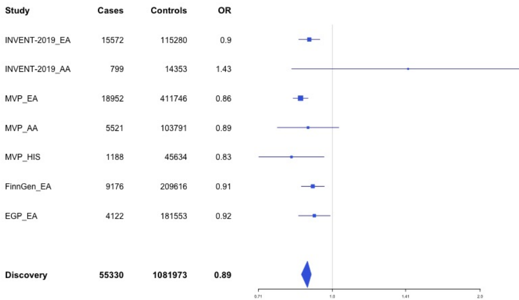
Supplementary Figure 1.46 – rs10886430 (chr10:121010256) in locus 75 (GRK5)
