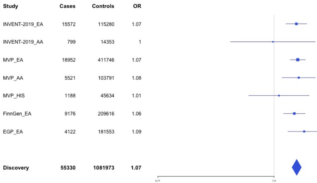
Supplementary Figure 1.59 – rs57035593 (chr14:92268096) in locus 97 (TC2N)
