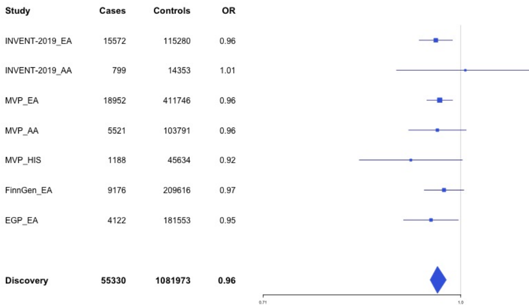
Supplementary Figure 1.62 – rs59442804 (chr15:60899031) in locus 101 (RORA-AS1)
