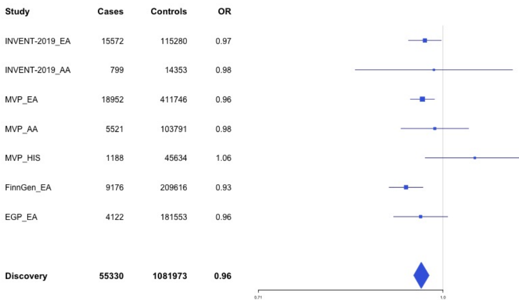
Supplementary Figure 1.34 – rs67694436 (chr8:6654220) in locus 56 (AGPAT5;XKR5)
