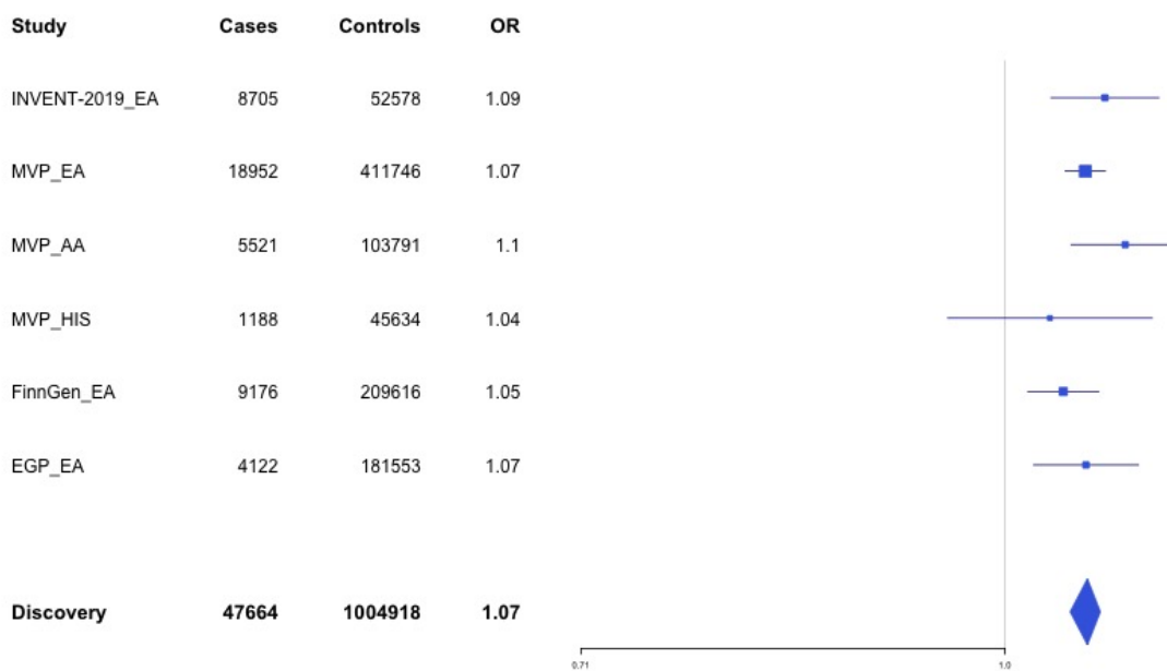
Supplementary Figure 1.84 – rs6048 (chr23:138633280) in locus 134 (F9)
