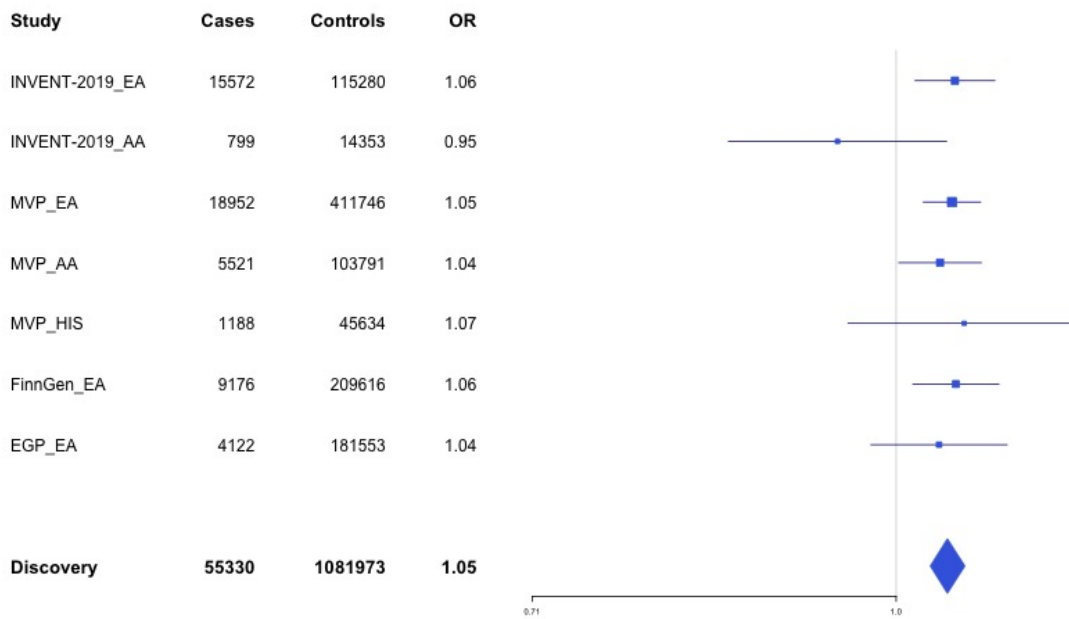
Supplementary Figure 1.47 – rs11032074 (chr11:32993887) in locus 78 (QSER1)
