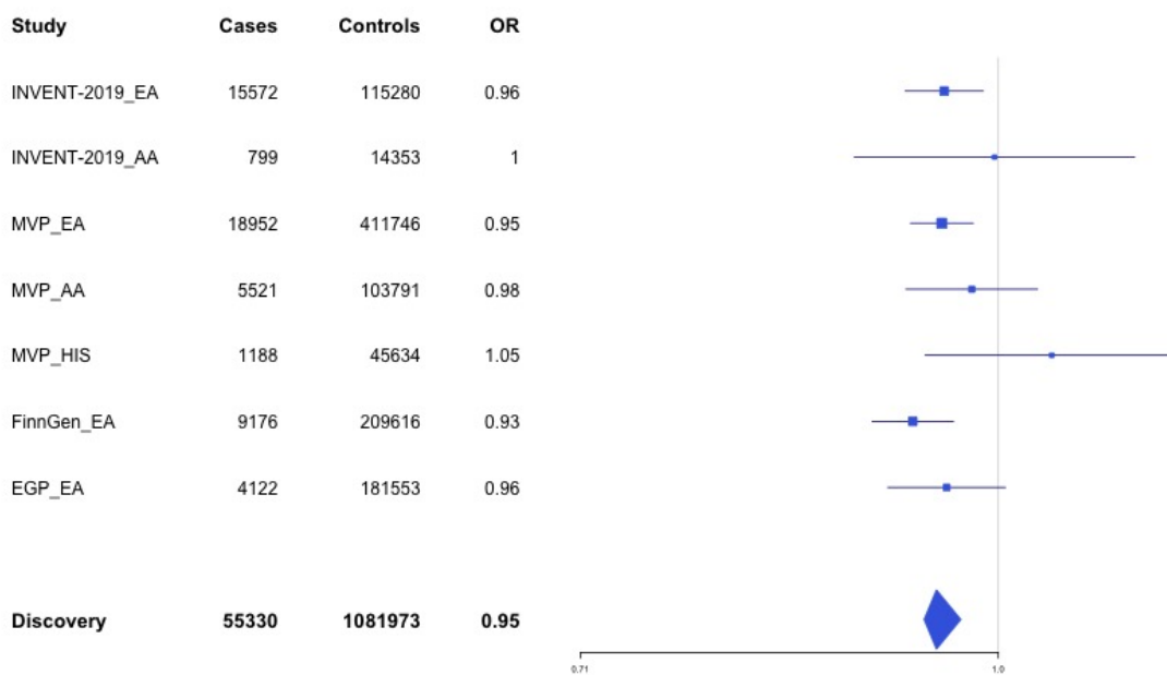
Supplementary Figure 1.10 – rs715 (chr2:211543055) in locus 21 (CPS1)
