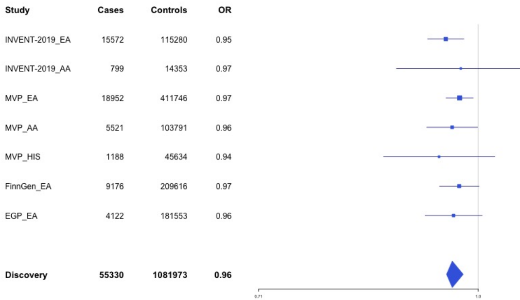
Supplementary Figure 1.41 – rs1887091 (chr10:14535113) in locus 67 (MIR1265 ;FAM107B)
