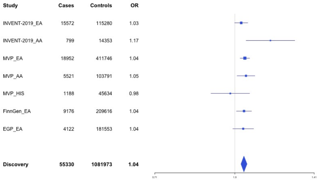
Supplementary Figure 1.45 – rs2274224 (chr10:96039597) in locus 74 (PLCE1)
