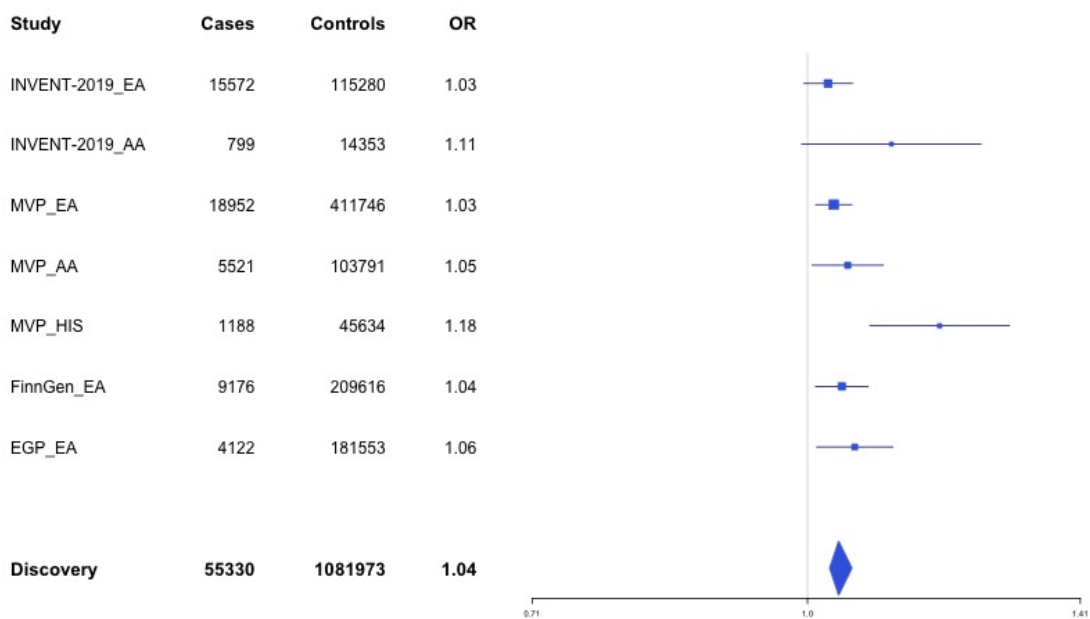
Supplementary Figure 1.60 – rs8013957 (chr14:103140254) in locus 99 (RCOR1)
