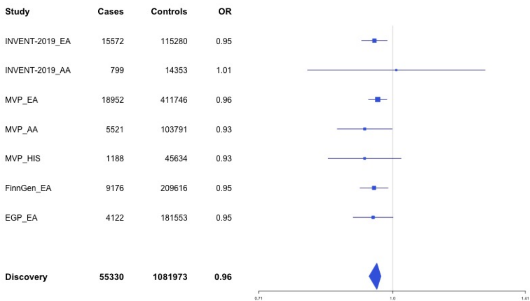
Supplementary Figure 1.32 – rs42036 (chr7:92241451) in locus 54 (CDK6)
