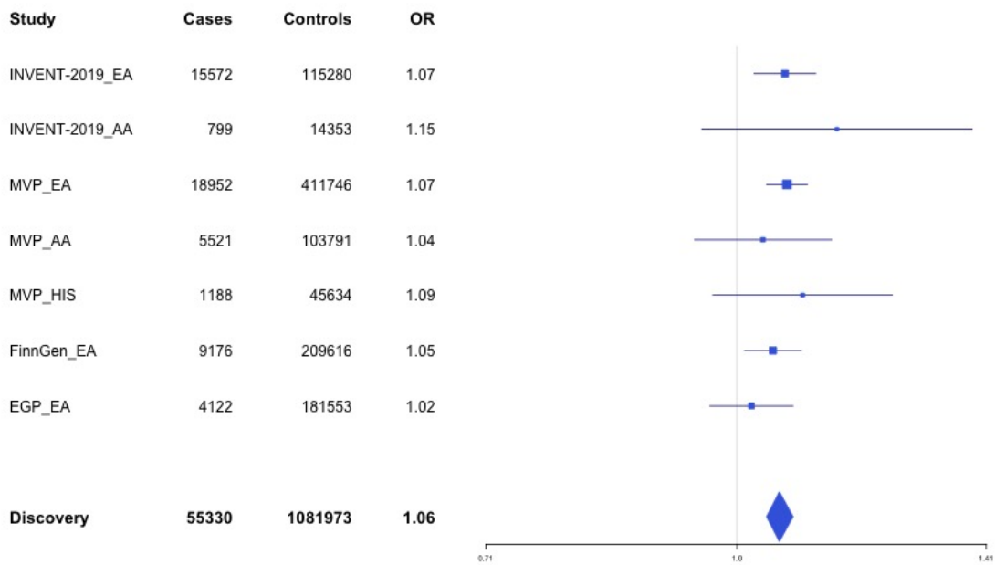
Supplementary Figure 1.11 – rs13412535 (chr2:224874874) in locus 22 (SERPINE2)
