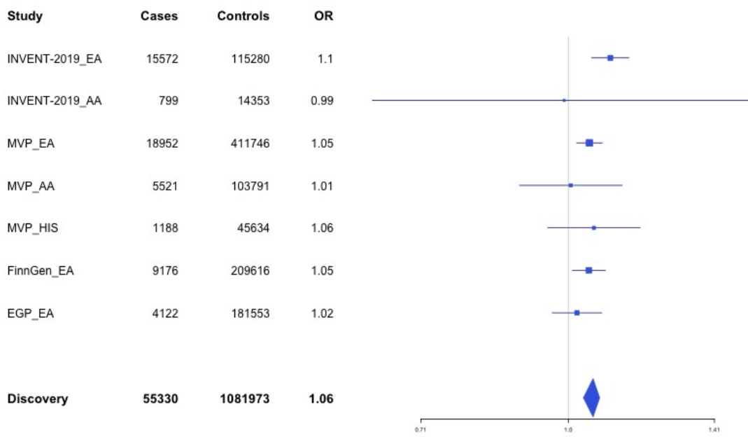
Supplementary Figure 1.2 – rs3767812 (chr1:118155620) in locus 5 (TENT5C)
