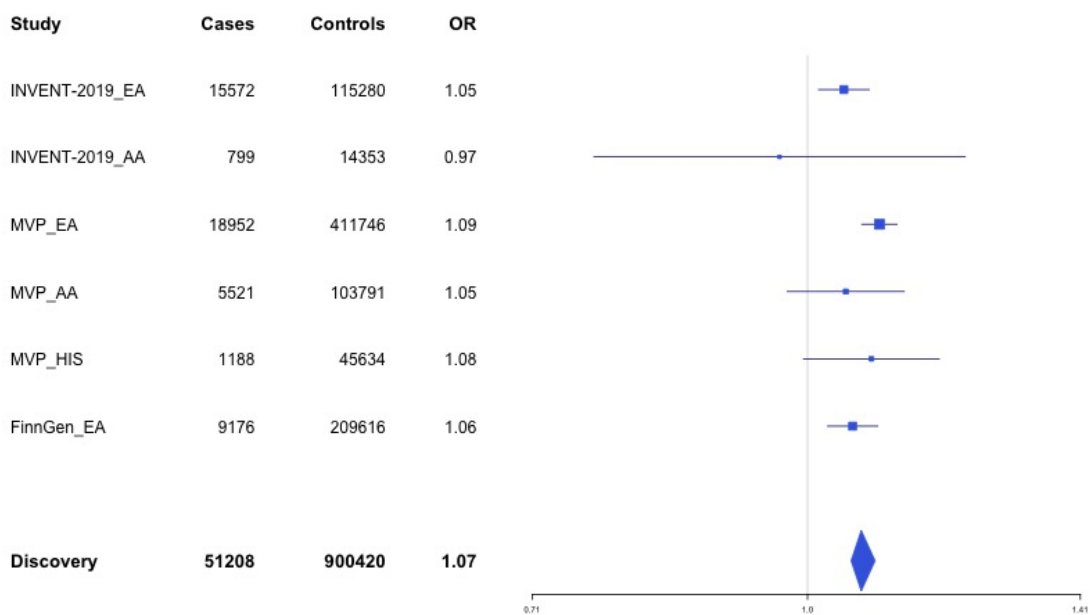
Supplementary Figure 1.50 – rs174551 (chr11:61573684) in locus 82 (FADS1)
