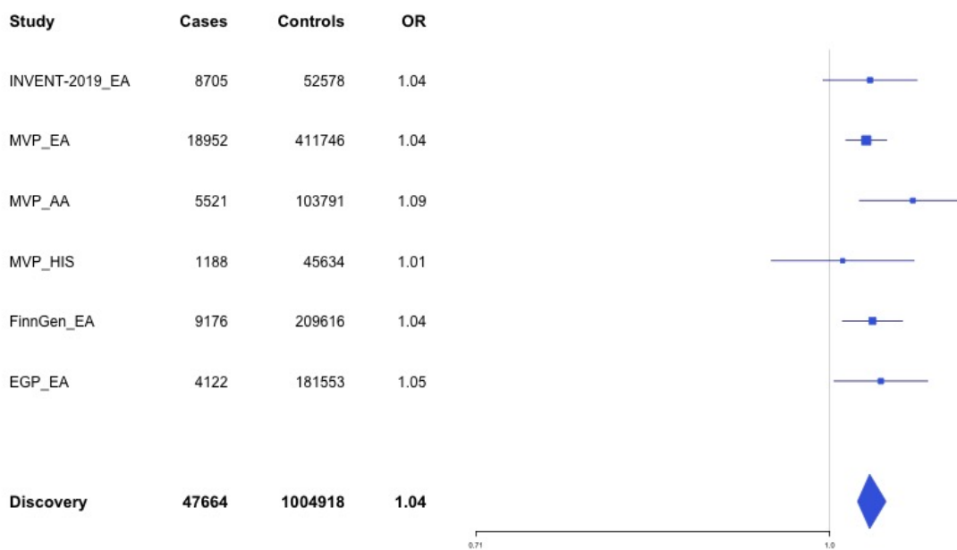
Supplementary Figure 1.82 – rs6632109 (chr23:34894638) in locus 132 (TMEM47;FAM47B)
