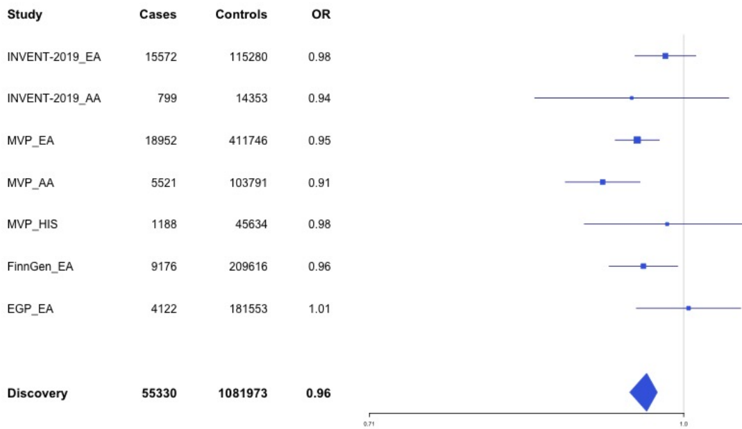
Supplementary Figure 1.35 – rs7010926 (chr8:10626791) in locus 58 (PINX1)
