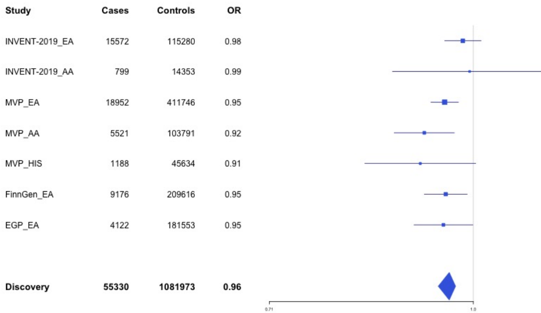
Supplementary Figure 1.53 – rs7311483 (chr12:9053661) in locus 88 (A2ML1 ;PHC1)
