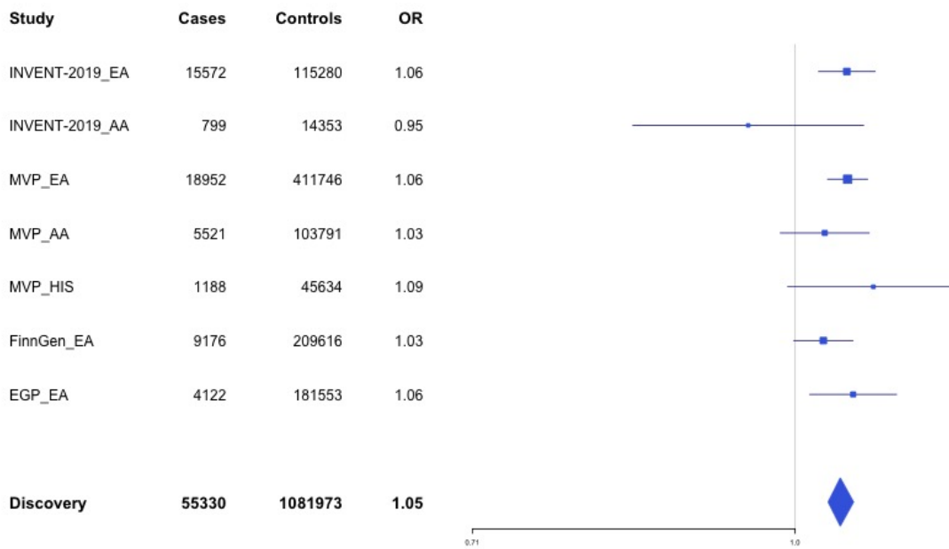
Supplementary Figure 1.67 – rs6503222 (chr17:1977862) in locus 112 (SMG6)
