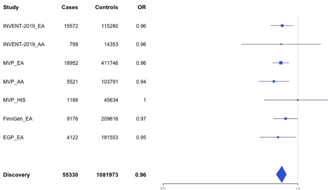
Supplementary Figure 1.74 – rs1688264 (chr19:49209560) in locus 123 (FUT2)
