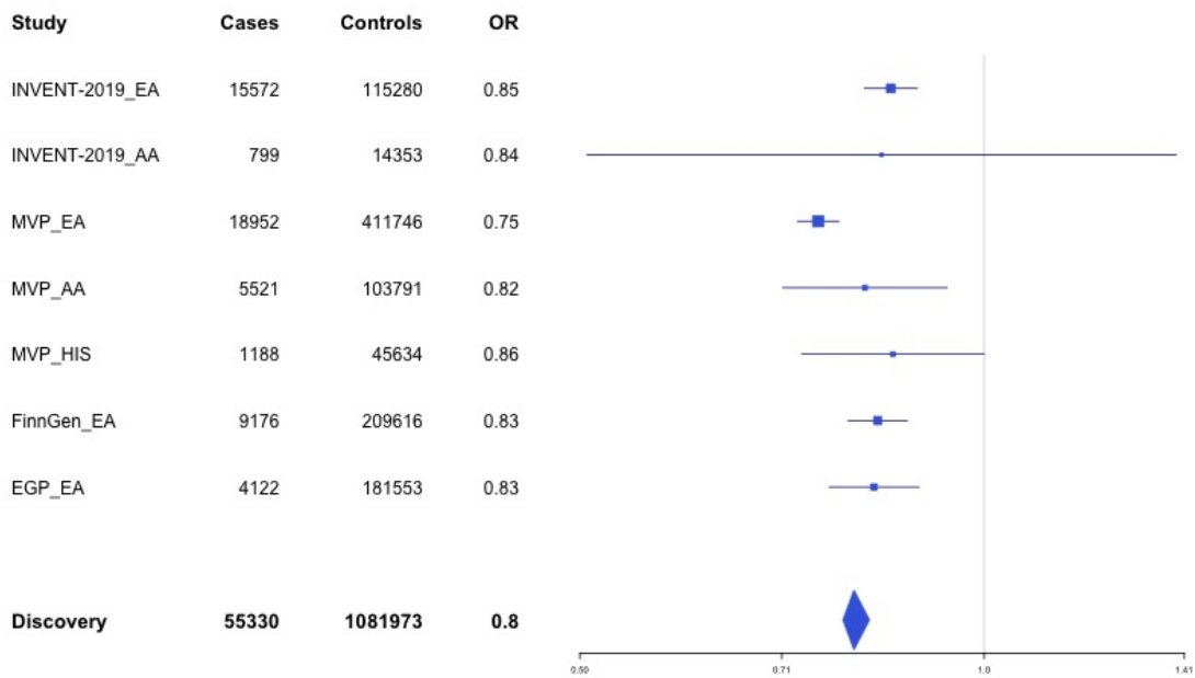
Supplementary Figure 1.43 – rs17490626 (chr10:71218646) in locus 72 (TSPAN15)
