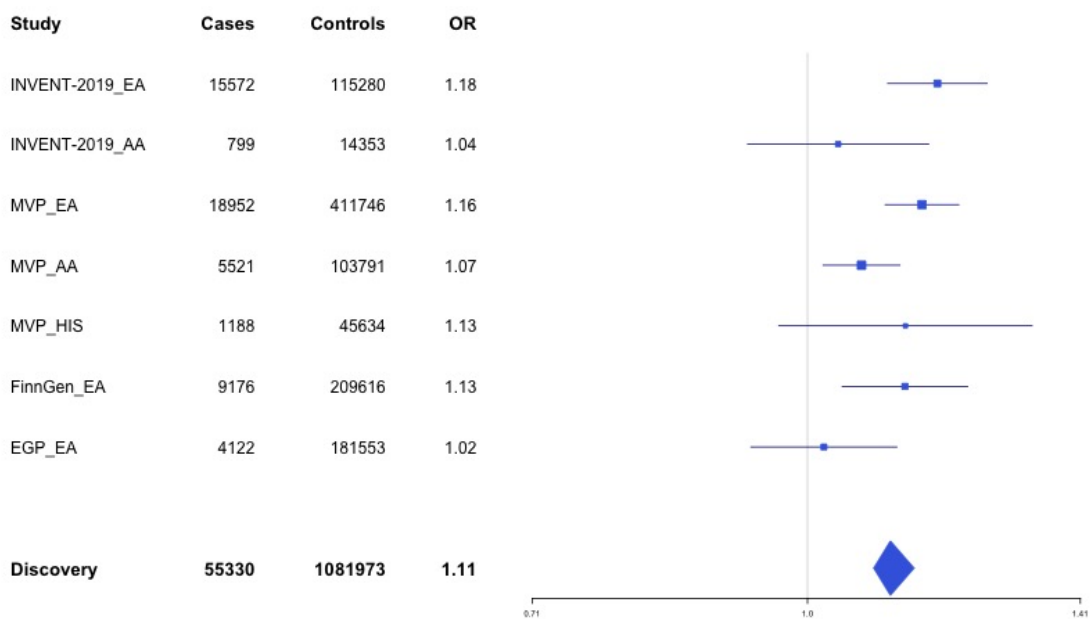
Supplementary Figure 1.4 – rs2842700 (chr1:207282149) in locus 13 (C4BPA)
