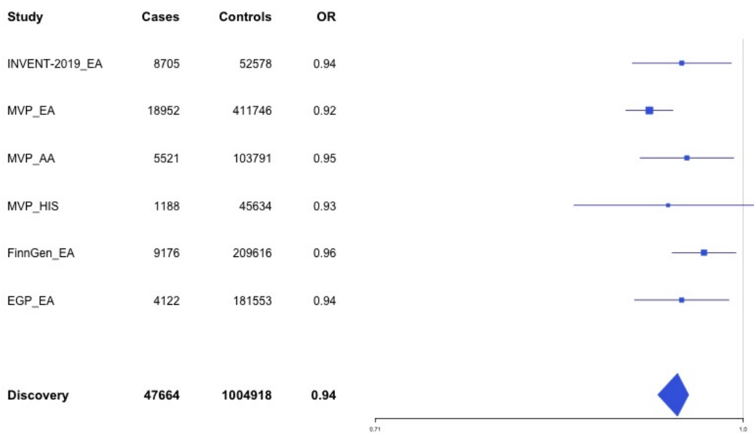
Supplementary Figure 1.85 – rs2084408 (chr23:154346709) in locus 135 (BRCC3)
