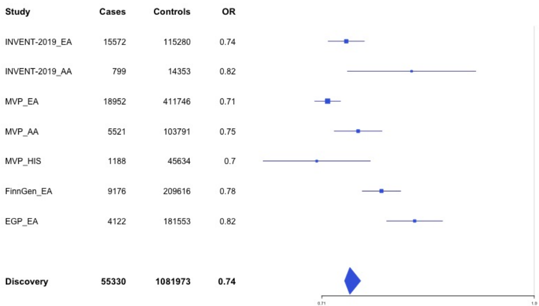
Supplementary Figure 1.40 – rs505922 (chr9:136149229) in locus 66 (ABO)
