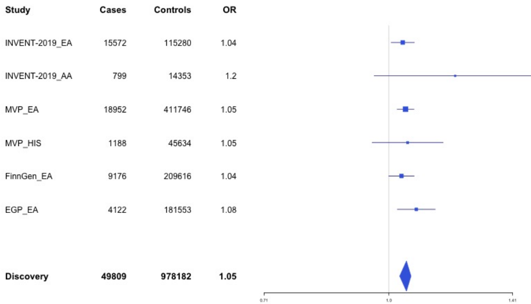
Supplementary Figure 1.79 – rs4820093 (chr22:33160208) in locus 129 (SYN3)
