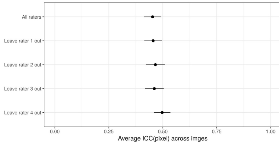
Figure S6: Leave-one-rater out sensitivity analysis of the average pixel-level ICC measure.
