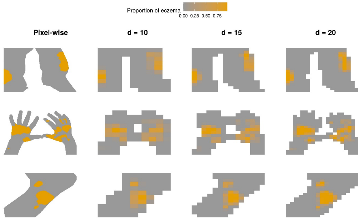
Figure S1: Illustration of area-level segmentation compared to pixel-level segmentation, for the same images as in Figure 1, for the segmentation for rater 1. Rows correspond to images and columns to pixel- and area-level segmentation for different image resolutions ( d ).
