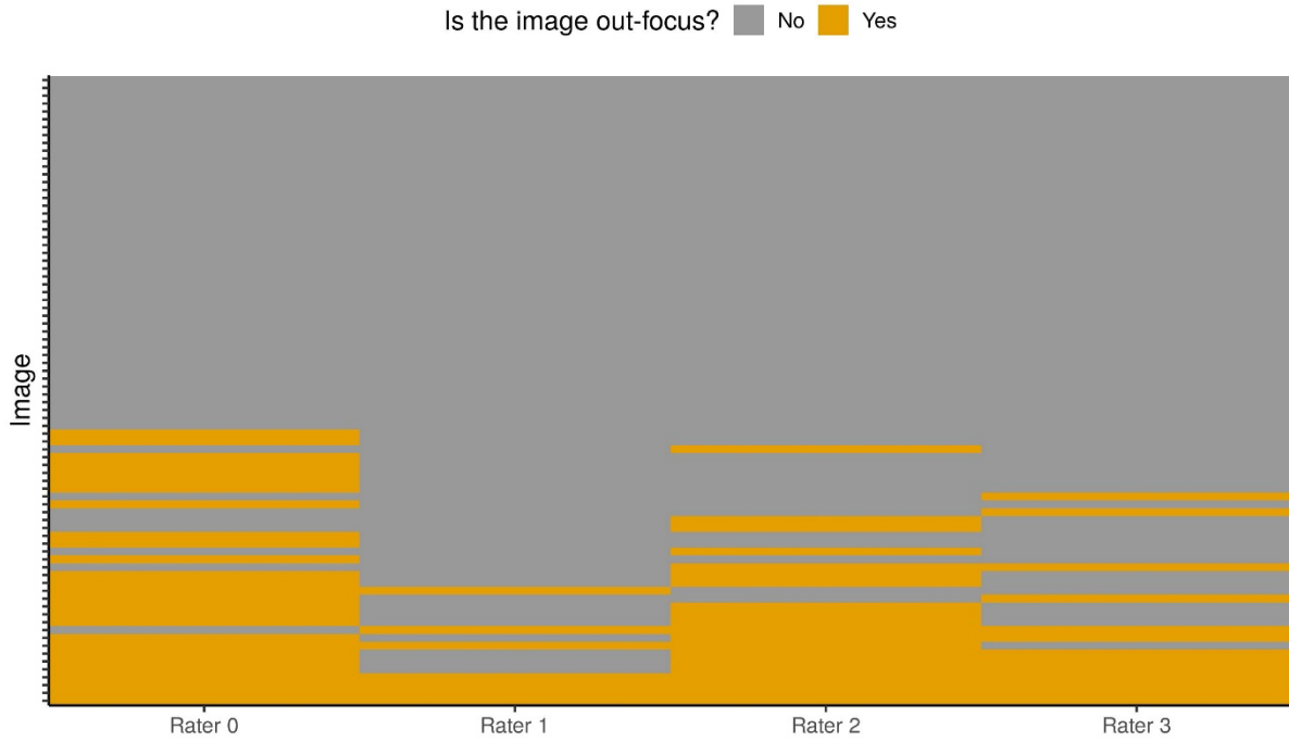
Figure S2: Distribution of out-of-focus assessments by the four raters (x-axis) for each image (y-axis). The orange represents that the rater deemed the image out-of-focus. 17 images were deemed out-of-focus by only one rater, 8 images by two raters, 6 images by three raters and 4 images by all the four raters.
