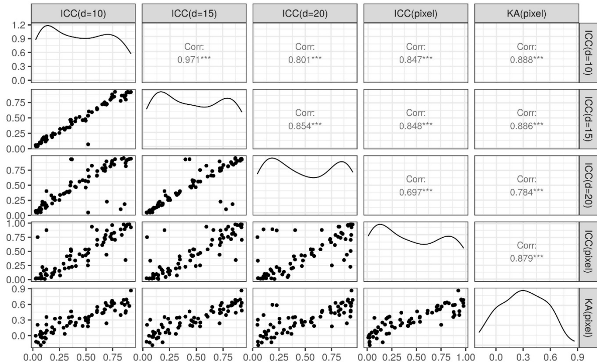
Figure S4: Comparison between the IRR metrics considered in this study (scatter plots, density plots and Pearson correlations).
