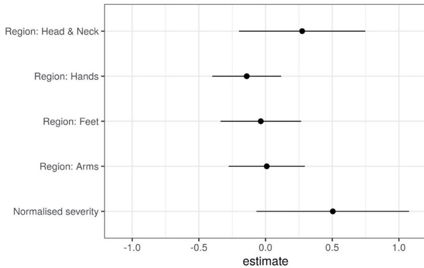
Figure S3: Estimated coefficients (and 95% CI) for variables in a linear model that predicts the mean image quality score across raters. The coefficients for the regions quantify the difference in the intercept from that of the default region (legs).
