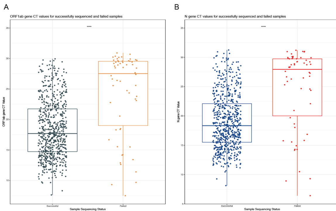
Supplementary Figure 1. Comparison of two SARS-CoV-2 genes targets of TaqPath RT-PCR for failed and successfully sequenced samples (A) Comparison of ORF1ab gene CT values among all samples that generated high or low-quality genomes. The first, second, and third quartiles are within the box, with the median line bolded. Samples are displayed as points with outliers included. P-values were generated using Wilcoxon rank-sum test and asterisks indicate P-value < 0.05 ( p < 0.0001 ). (B) Comparison of N gene CT values among all samples that generated high or low-quality genomes. (S gene CT values are not included as a third comparison from RT-PCR target because SGTF presence or value of 0 would greatly affect comparisons).
