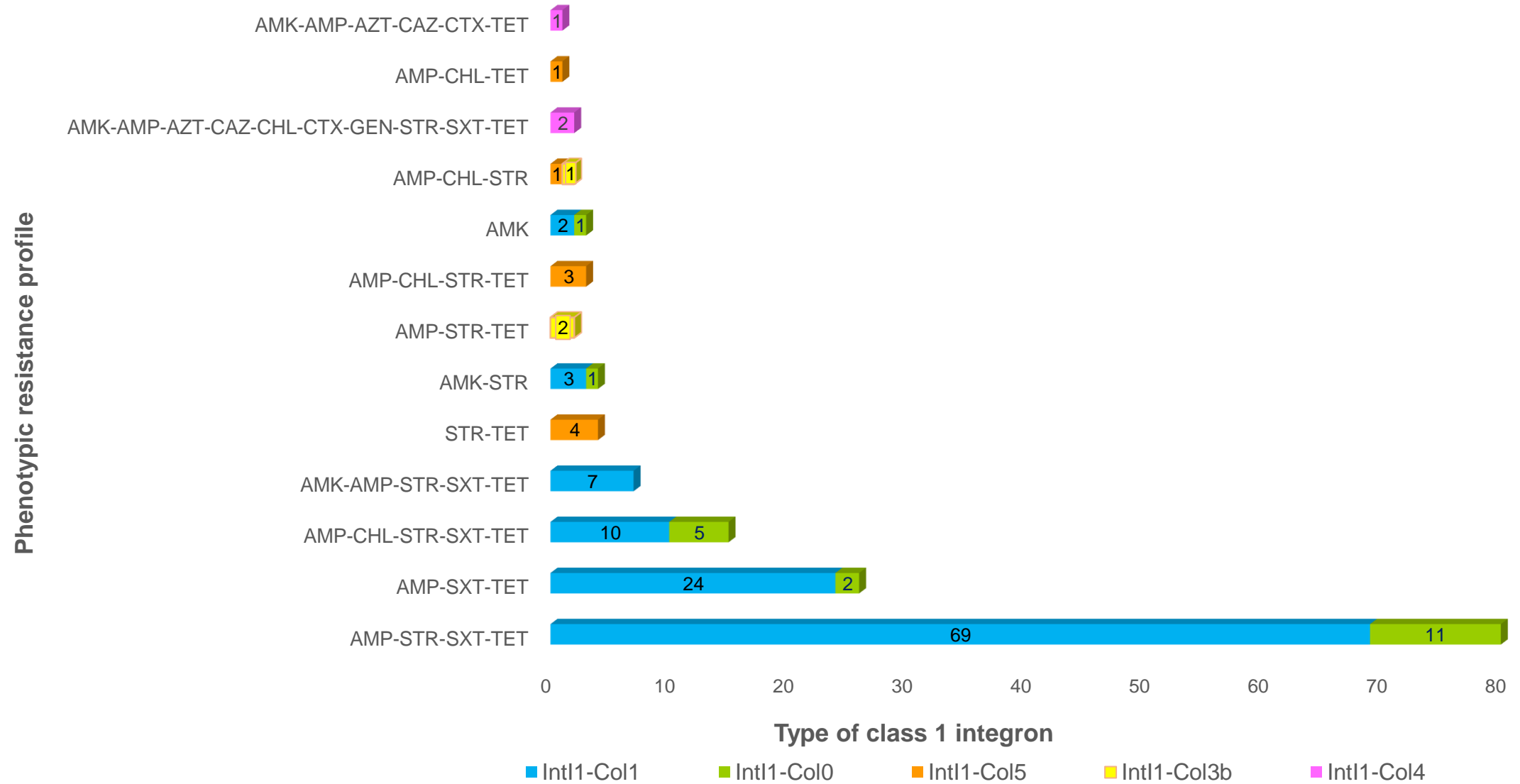
Figure S1. Susceptibility profile and main types of class 1 integrons ( n \geq 3 ) detected in S. Typhimurium isolates from Colombian clinical samples, during 1997-2017.
