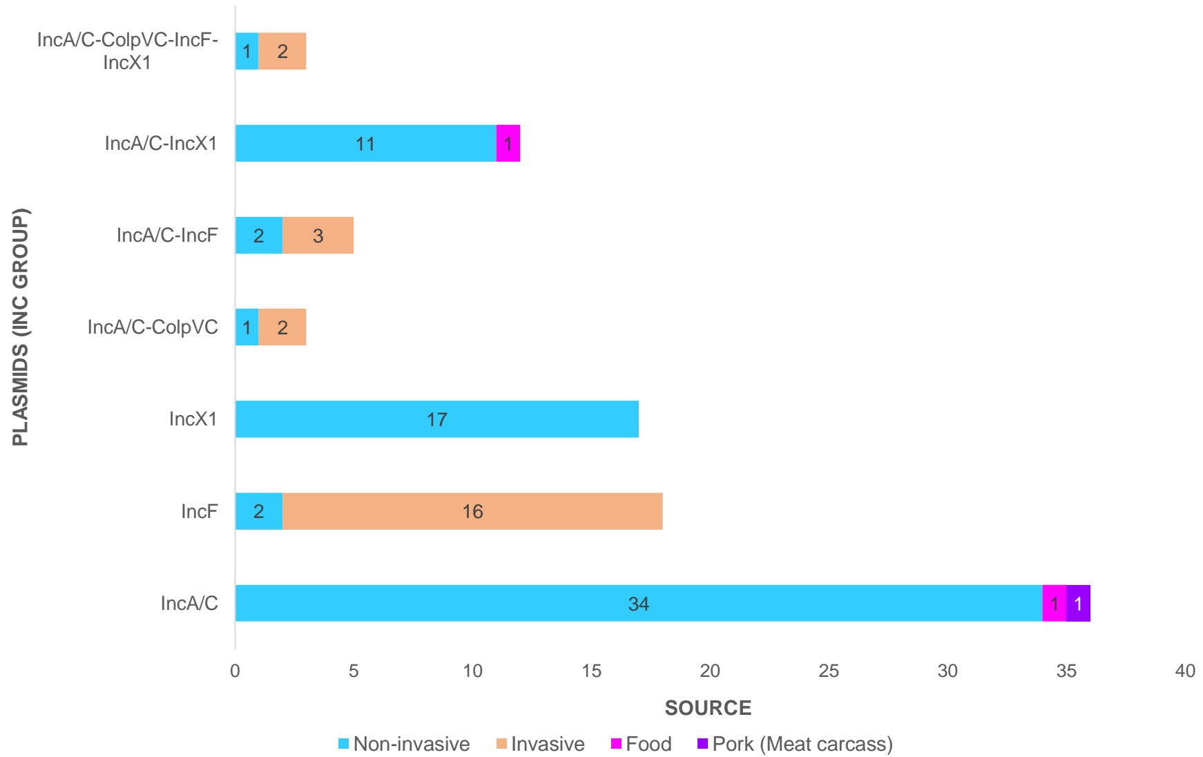
Figure S3. Inc groups of plasmids (n≥3) and source in S. Typhimurium isolates from Colombia, during 1997-2017.
