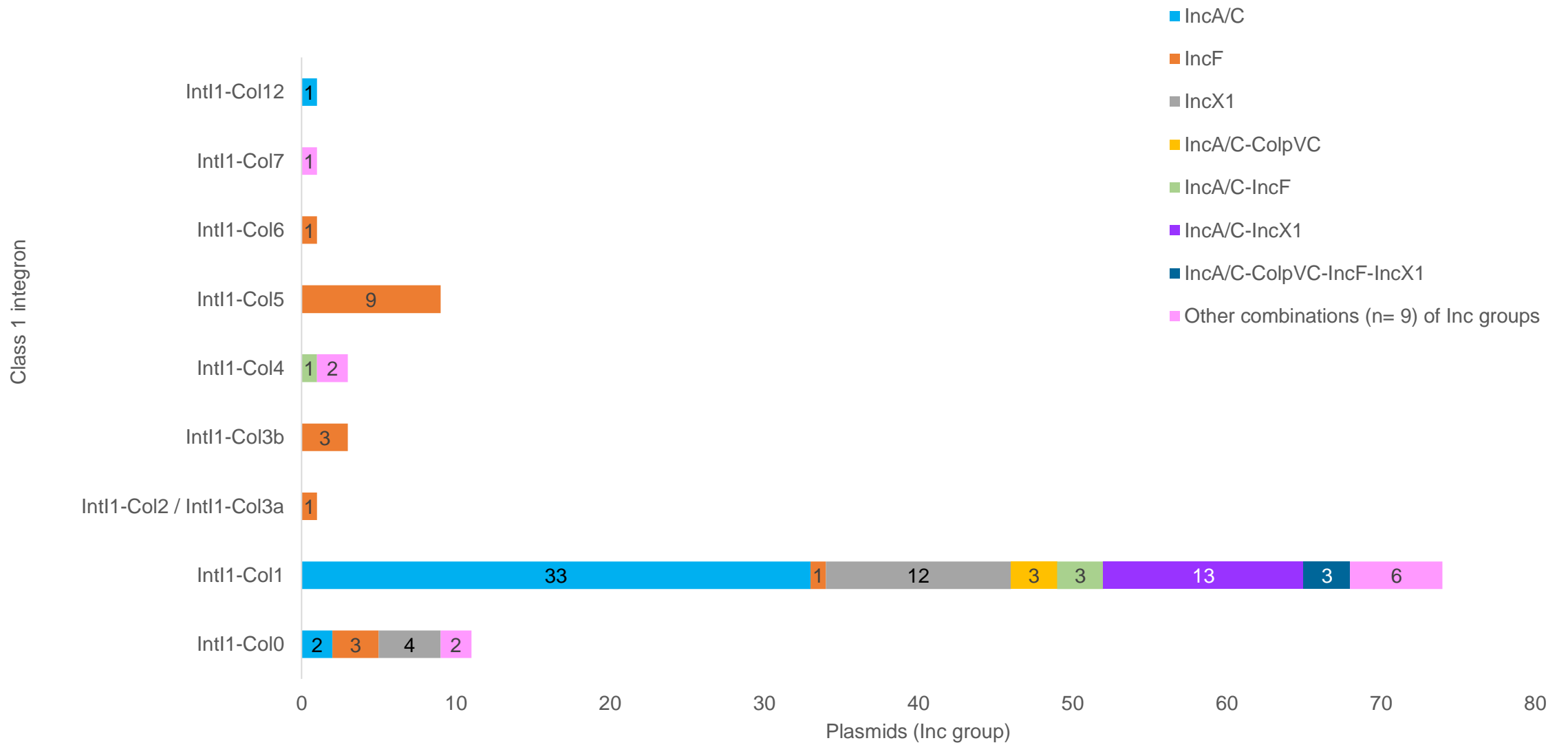
Figure S2. Class 1 integrons types and Inc groups of plasmids in S. Typhimurium from Colombia (Col), 1997-2017.
