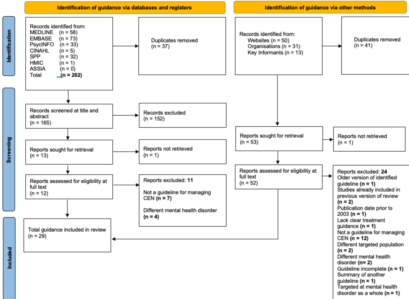
Figure 1. PRISMA diagram.
