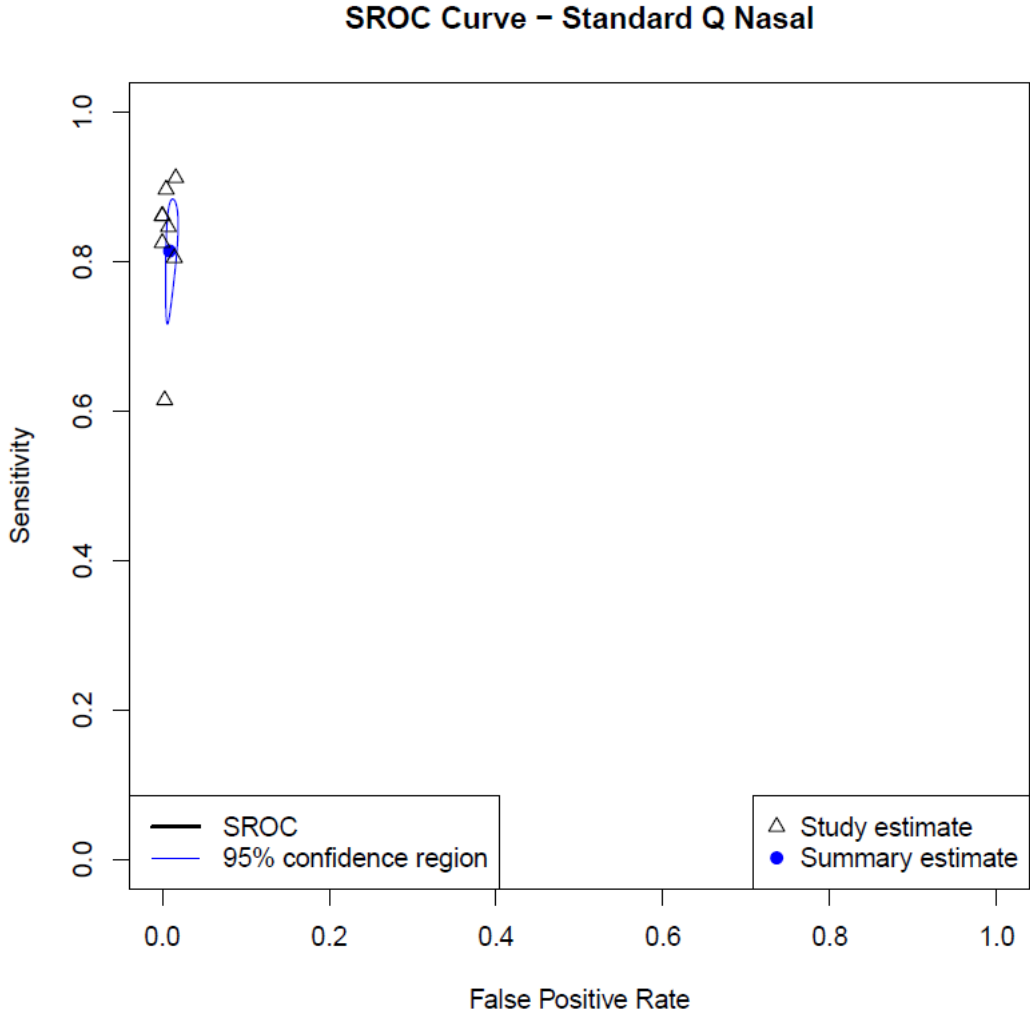
Fig A – HSROC curve Standard Q nasal
