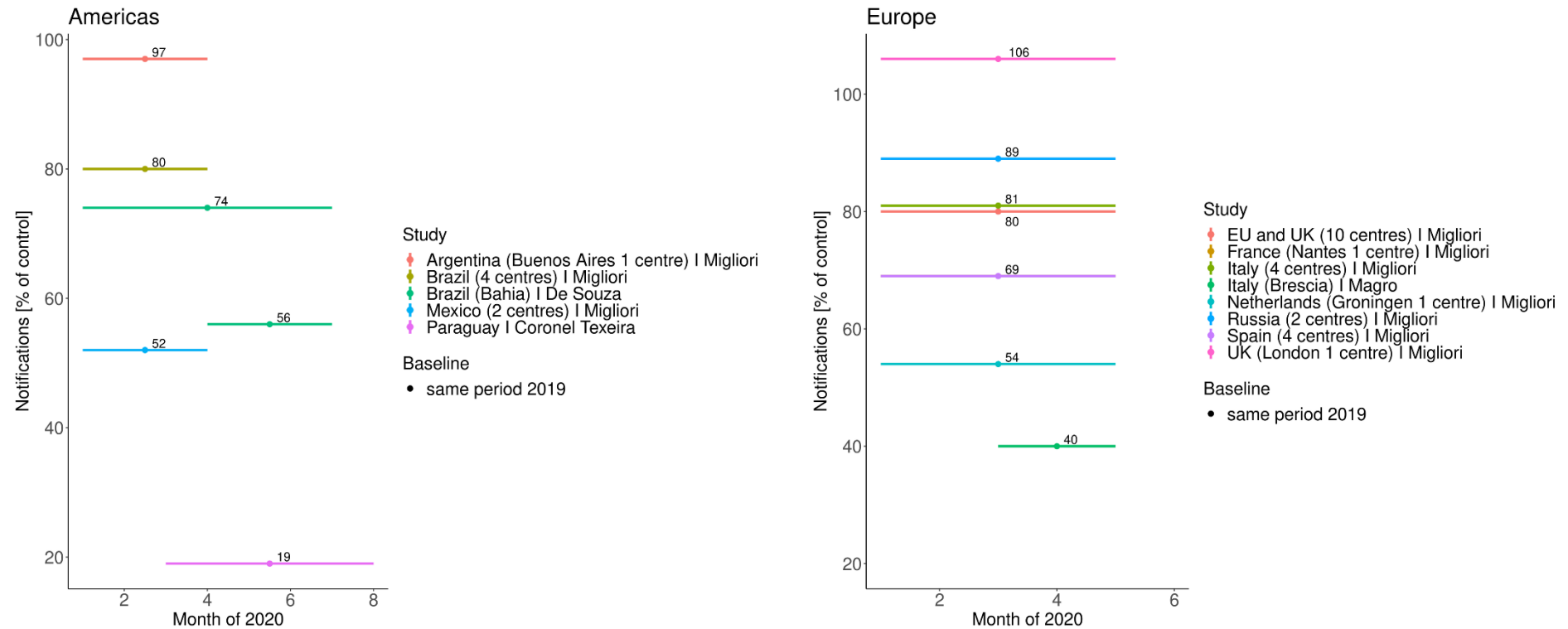
S1 Fig. 5 TB notifications in Americas and Europe. Overview of notifications registered over a certain period (depicted by the horizontal lines) as percentage of notifications in a control period (referred to as Baseline in the legend). Thus, a value of 20% means a relative decrease of 80%.
