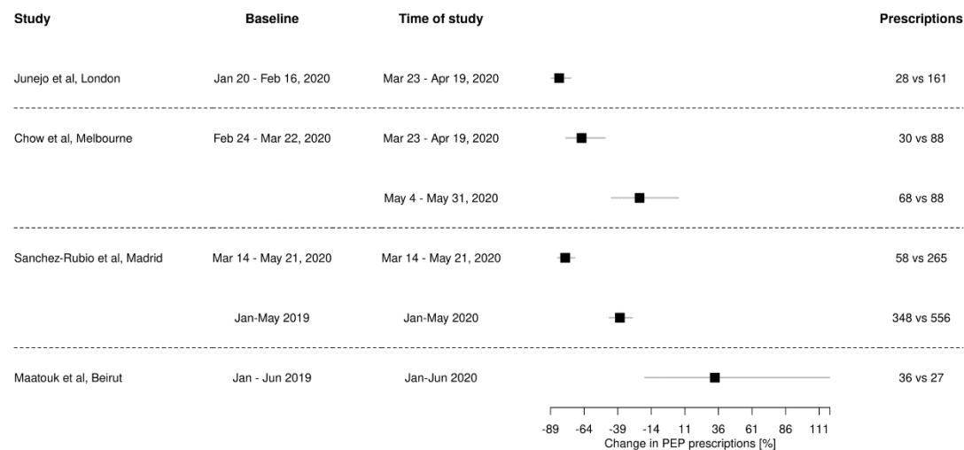
S1 Fig. 8 Reduction in PEP prescriptions. Shown are 95% confidence intervals based on the assumption of a Poisson distribution for the observed counts. Although the numbers were not reported, Sanchez-Rubio et al. [159] commented that the numbers started to increase even before the lockdown was at the end, which is what Chow et al. [160] observed as well.
