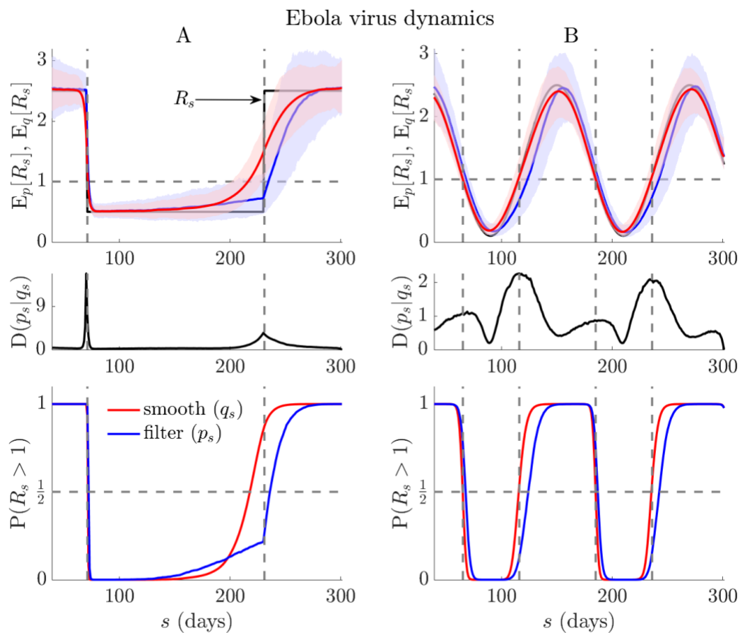
Fig 2: Resurgence and control dynamics of Ebola virus. Using renewal models with the generation time from [46], we simulate 1000 realisations of Ebola virus epidemics ( t = 300 ) with step (A panels) and seasonally (B panels) changing transmissibility (true R_s in black). Top panels show posterior mean estimates from the filtered ( E_p[R_s] , blue) and smoothed ( E_q[R_s] , red) distributions from every realisation (computed using EpiFilter [15]). Middle panels average the Kullback-Liebler divergences from those simulations, D(p_s|q_s) , and bottom panels display the overall filtered ( P(R_s > 1 | I_1^s) , blue), and smoothed ( P(R_s > 1 | I_1^t) , red) probabilities of resurgence. We find fundamental and striking delays in detecting resurgence, often an order
