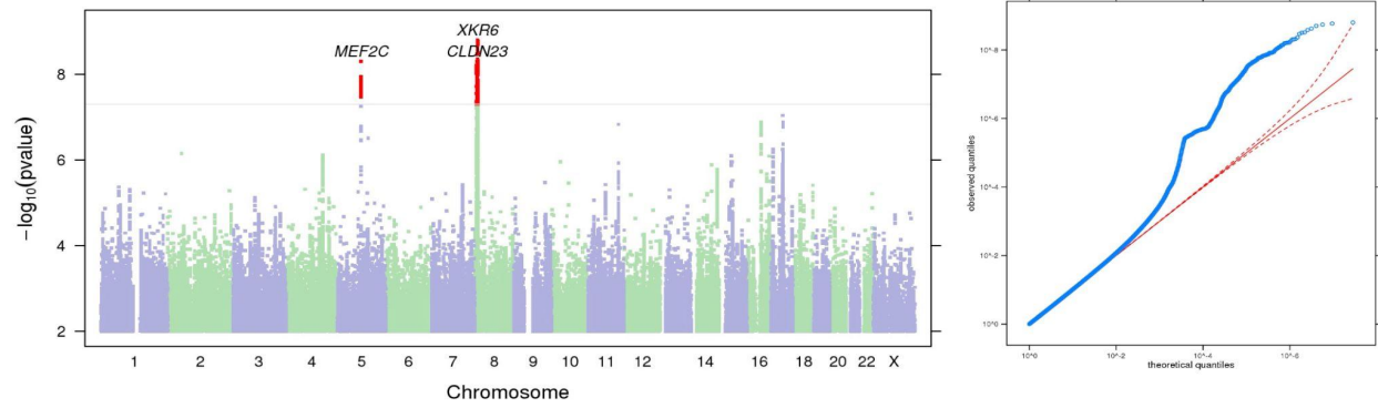
Figure S10. Manhattan and QQ plots of GWAS results indicating the strongest associations between the 22 autosomes, X chromosome, and UPPS-P Negative Urgency . The results have been adjusted for a genomic control inflation factor \lambda=1.002 (sample size = 132,559).
