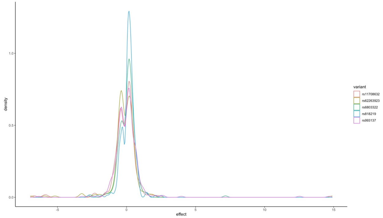
Figure S27. Range of standardized effect sizes (non-standardized \beta = -0.32 to 0.70 ) for FDR-significant traits in European ancestry.
