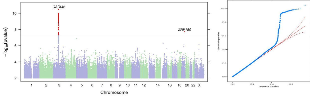
Figure S16. Manhattan and QQ plots of GWAS results indicating the strongest associations between the 22 autosomes, X chromosome, and BIS Motor . The results have been adjusted for a genomic control inflation factor \lambda=1.092 (sample size = 124,104).
