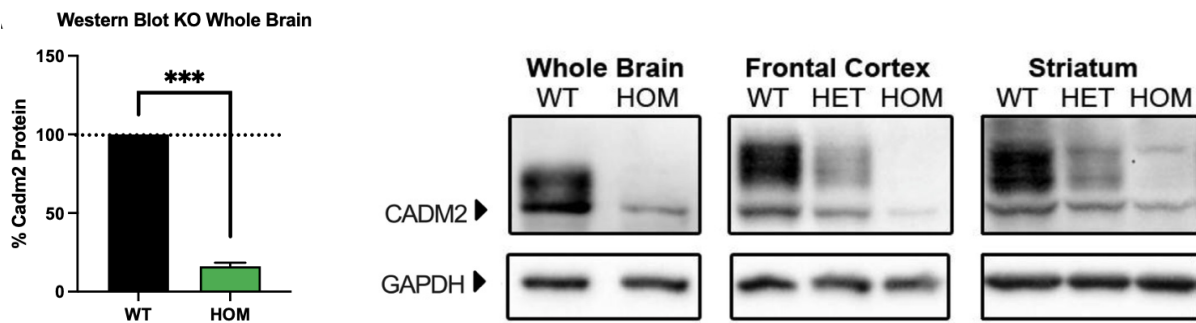
Figure S31. Cadm2 protein expression is significantly reduced in HOM (KO) mice relative to WT littermates. The left panel illustrates how knockout of the Cadm2 gene depletes whole brain CADM2 protein expression by approximately 84% relative to WT littermates. The right panel shows representative Western blots of whole brain, frontal cortex, and striatal lysates probed for CADM2 protein.
