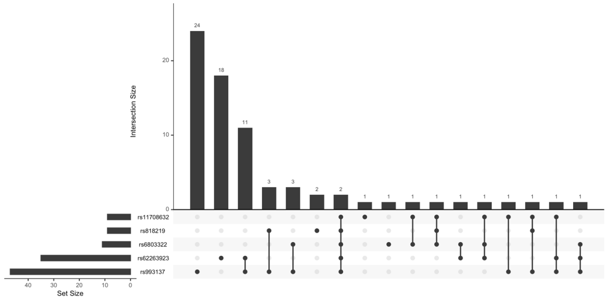
Figure S26. Overlap of FDR-significant traits for each of the tested variants in Latinx ancestry. Set Size denotes the total number of FDR-significant traits for each SNP while Intersection Size shows the number of traits that overlap between the SNPs.
