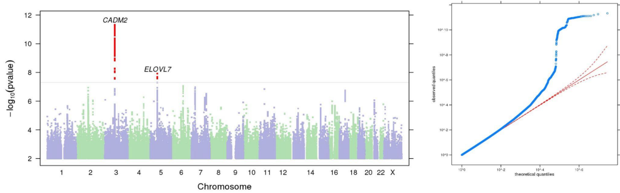
Figure S18. Manhattan and QQ plots of GWAS results indicating the strongest associations between the 22 autosomes, X chromosome, and BIS Nonplanning . The results have been adjusted for a genomic control inflation factor \lambda=1.123 (sample size = 123,509).
