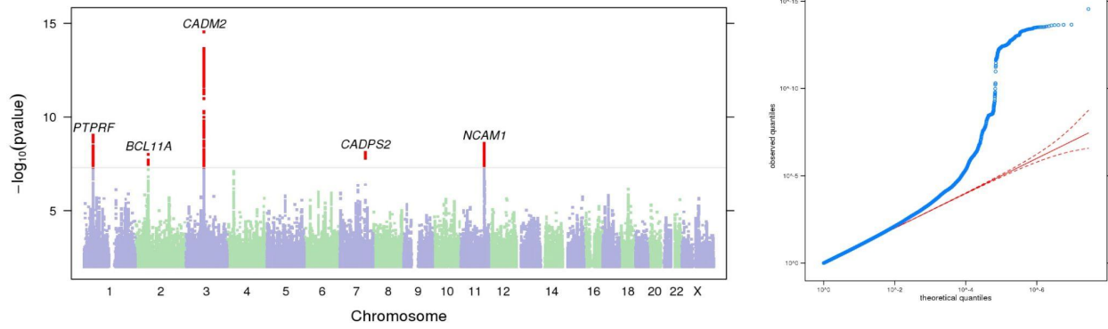
Figure S20. Manhattan and QQ plots of GWAS results indicating the strongest associations between the 22 autosomes, X chromosome, and Drug Experimentation . The results have been adjusted for a genomic control inflation factor \lambda=1.135 (sample size = 130,684).
