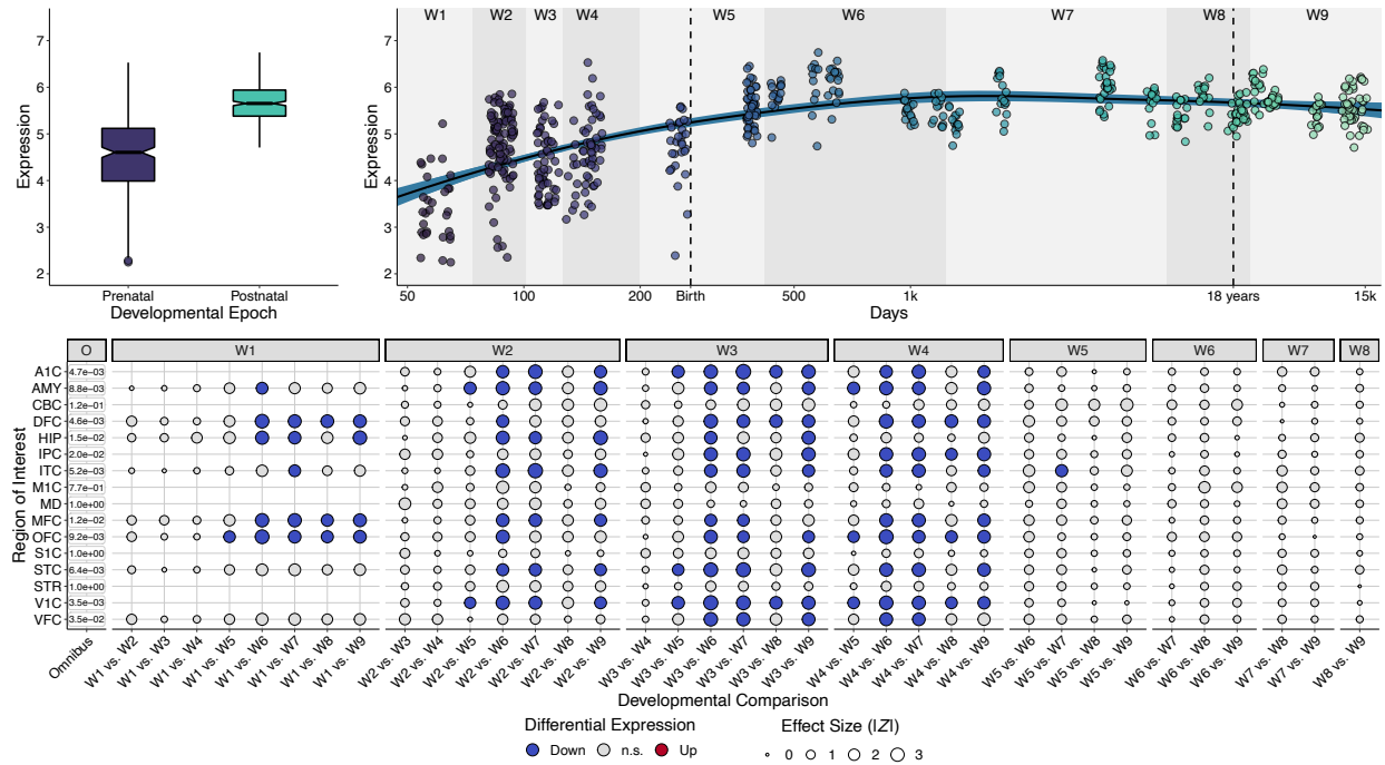
Figure S29. Differential expression of CADM2 across development in human brain tissue, as measured in the PsychENCODE (PEC) dataset. Normalized gene expression values are plotted as \log_2 RPKM + 1. In the top left panel, CADM2 expression in human brain tissue is plotted as box plots stratified by prenatal and postnatal epoch. In the top right panel, the trajectory of CADM2 expression in human brain tissue is plotted across development, as estimated with LOESS. Postconceptional days are plotted in \log_2 scale on the x-axis. In the bottom panel, Kruskal-Wallis and Dunn's tests of differential expression for developmental windows (W1-W9) in specific regions of interest (ROIs) are plotted as a bubble plot. The P values for Kruskal-Wallis tests in the leftmost column are corrected for false discovery rate (FDR) across ROIs (16 tests), whereas the P values for Dunn's tests are corrected within ROIs (up to 36 tests). The ROIs included were primary auditory cortex (A1C), amygdala (AMY), cerebellar cortex (CBC), dorsolateral prefrontal cortex (DFC), hippocampus (HIP), inferior parietal cortex (IPC), inferior temporal cortex (ITC), primary motor cortex (M1C), thalamus (MD) medial prefrontal cortex (MFC), orbital prefrontal cortex (OFC), primary somatosensory cortex (S1C), superior temporal cortex (STC), striatum (STR), primary visual cortex (V1C), and the ventrolateral prefrontal cortex (VFC).
