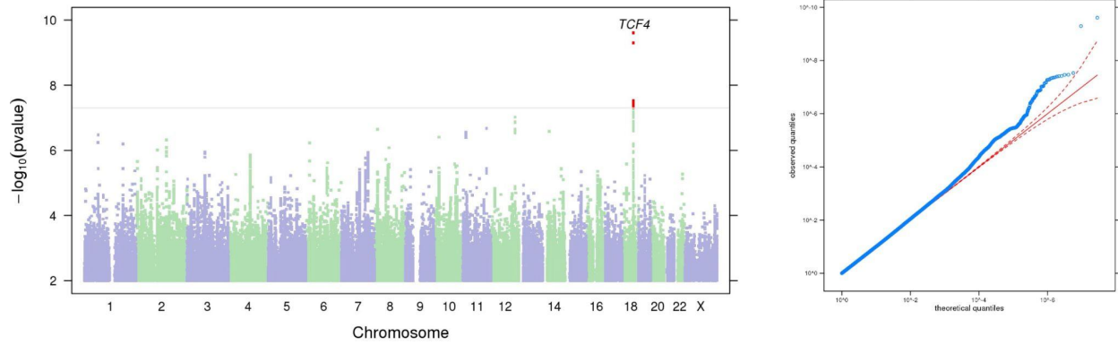
Figure S4. Manhattan and QQ plots of GWAS results indicating the strongest associations between the 22 autosomes, X chromosome, and UPPS-P Premeditation . The results have been adjusted for a genomic control inflation factor \lambda=1.085 (sample size = 132,667).
