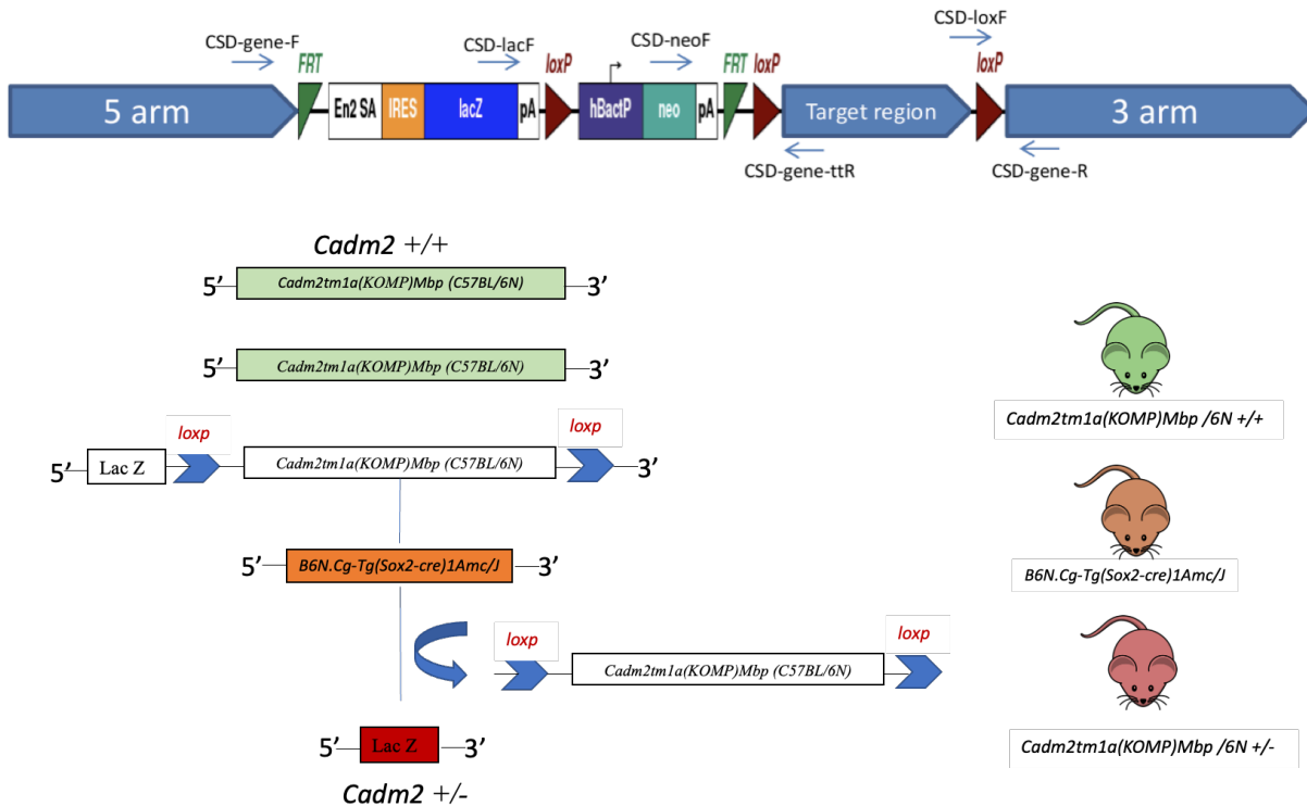
Figure S30. Targeted exon and mouse breeding figure.
