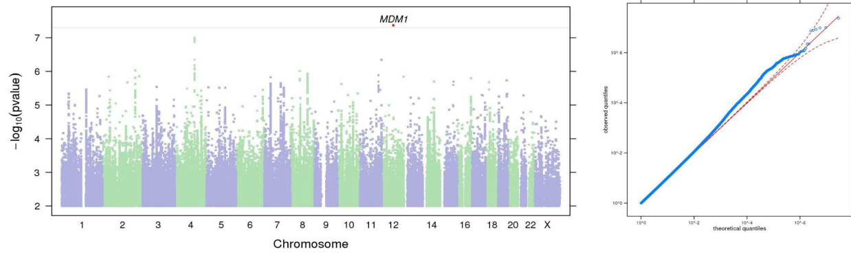
Figure S8. Manhattan and QQ plots of GWAS results indicating the strongest associations between the 22 autosomes, X chromosome, and UPPS-P Positive Urgency . The results have been adjusted for a genomic control inflation factor \lambda=1.001 (sample size = 132,132).
