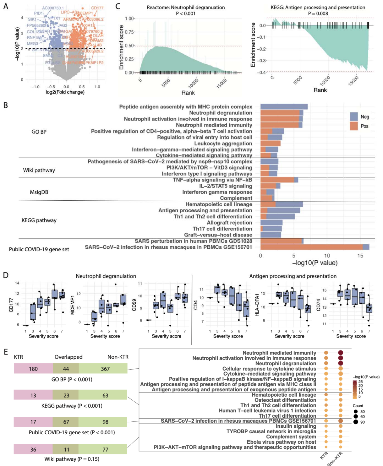
Figure 2. Transcriptome in KTRs with acute COVID-19 shows signature of neutrophil activation and deficient adaptive immune responses with increasing severity. (A) Volcano plot shows gene expression change associated with increasing severity score. The \log_2(\text{fold change}) reflects the direction and magnitude of change in expression per unit increase in severity score (see definition in Table 1). Differentially expressed genes (DEGs) were identified
