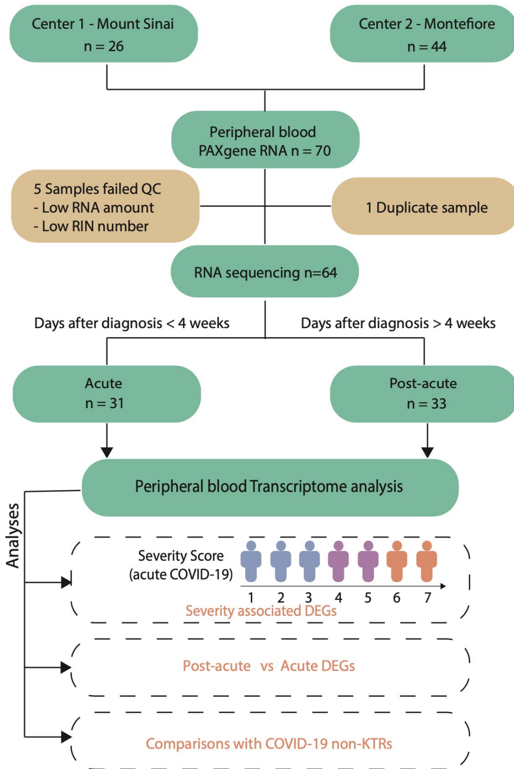
Figure 1. Flow diagram of study design. A total of 70 KTRs with documented evidence of SARS-CoV-2 infection were enrolled from two transplant centers in New York. Blood was
