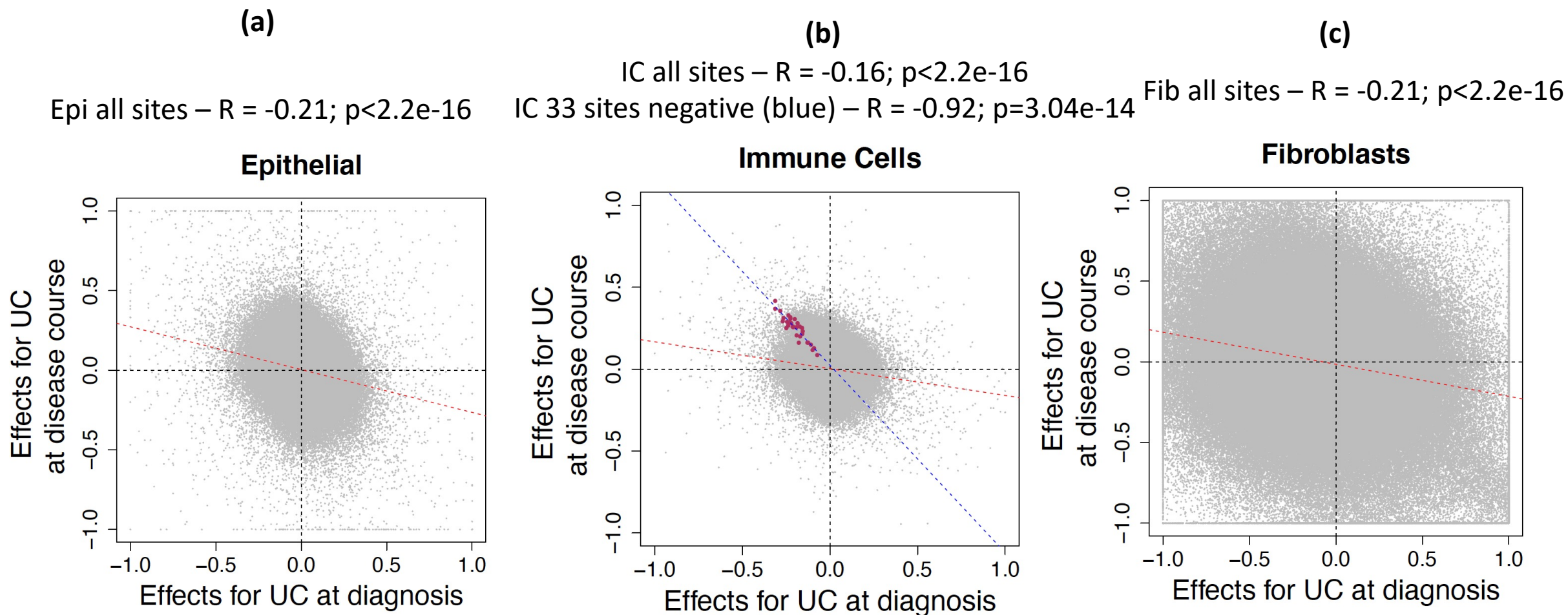
Supplementary Figure 5: The effect sizes for entire 820K DNAm sites were compared between UC at diagnosis and UC at disease course (y-axis) for (a) Epithelial and (b) immune cells, and (c) Fibroblast. In B, maroon dots represents the immune signatures that are significant by FDR < 0.05 at both UC at diagnosis and UC at disease course.
