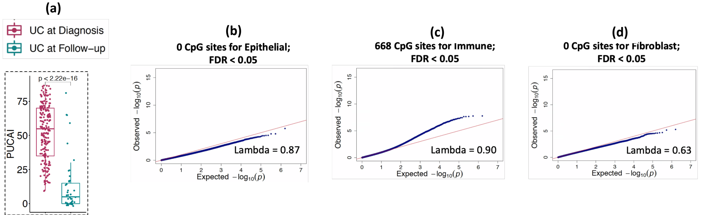
Supplementary Figure 4: (a) Comparison between UC at diagnosis (n=211) and UC follow-up (n=73) for the pediatric ulcerative colitis activity index (PUCAI) showed a significant reduction in the follow-up UC. The P-value is calculated using the Wilcoxon test. (b-d) The QQ plot representation shows no inflation for the CpG sites associated to UC at disease course that are derived from both (b) Epithelial and (c) immune cells, and (d) Fibroblast
