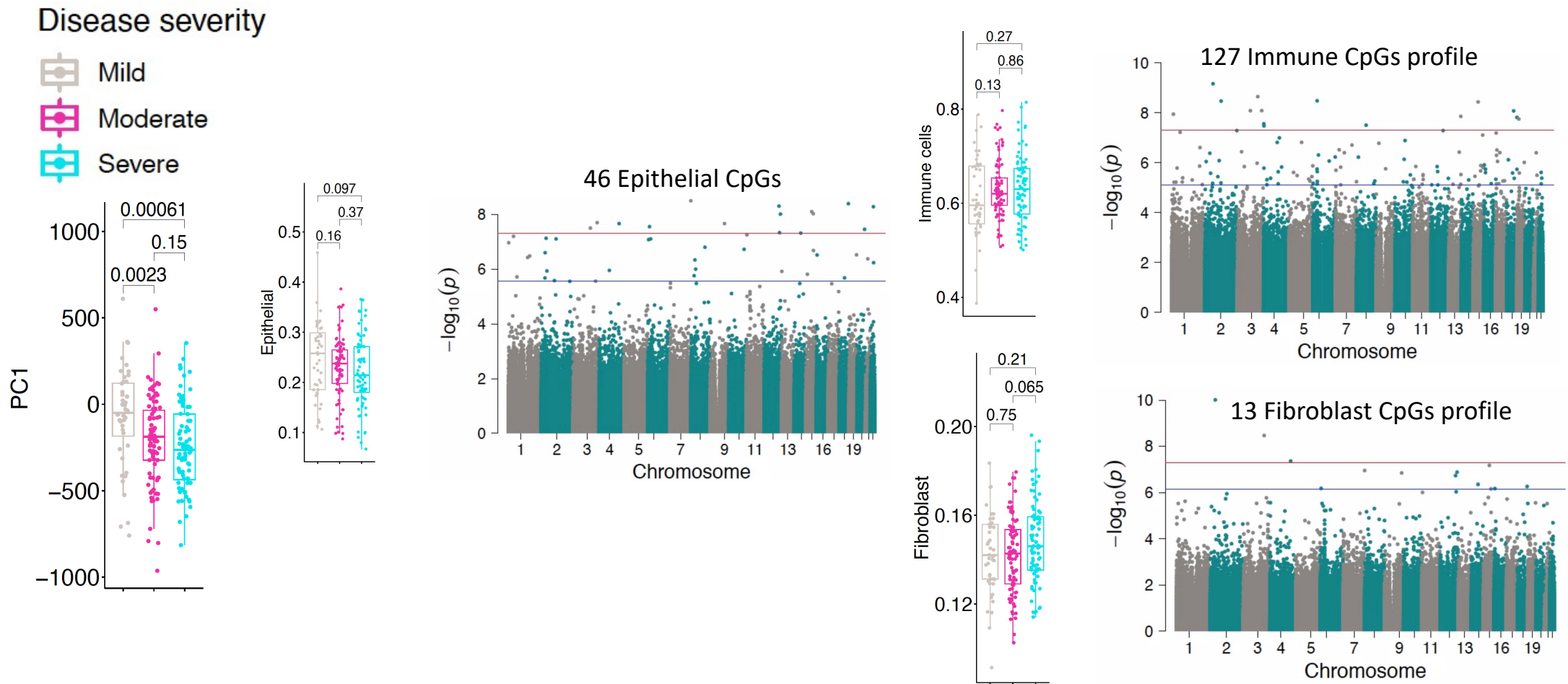
Supplementary Figure 8: DNAm signatures associated with disease severity defined by PUCAI (A) The boxplots show the PC1 obtained from rectal biopsy DNAm profiles compared among mild UC (n=44), moderate UC (n=87) and severe UC (n=80) defined by PUCAI. Top panel shows the epithelial, immune, and fibroblast cell proportions obtained from entire 820K sites at genome-wide (B) Cell-specific EWAS analysis shows differentially methylated sites between for moderate and severe UC combined (n=167), when compared to mild UC. The results shown for all three major cell types from top to bottom for epithelial, immune and fibroblast, respectively. The blue line indicates the sites significant by FDR < 0.05 and the red line represents the sites significant by genome-wide p < 1e-08 .
