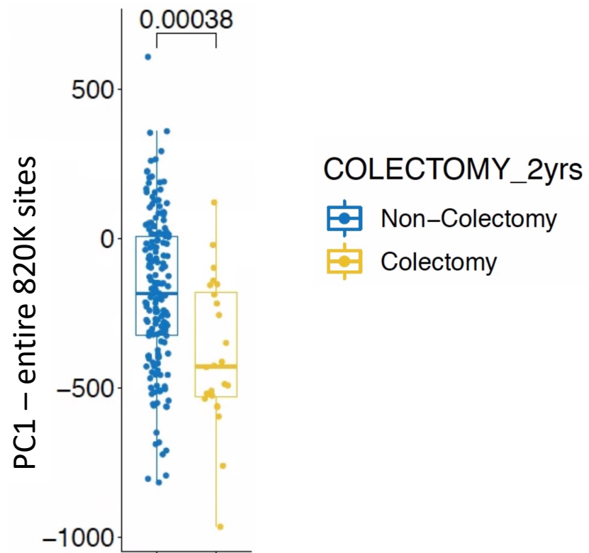
Supplementary Figure 9: Boxplot comparing PC1 of entire 820K sites among colectomy groups at diagnosis. X-axis shows non-colectomy UC patients (n=175) and UC patients who undergone colectomy (n=24) at 2 yrs . Y-axis shows the PC1 values obtained from entire 820K array. The given p-value was calculated by Wilcoxon test.
