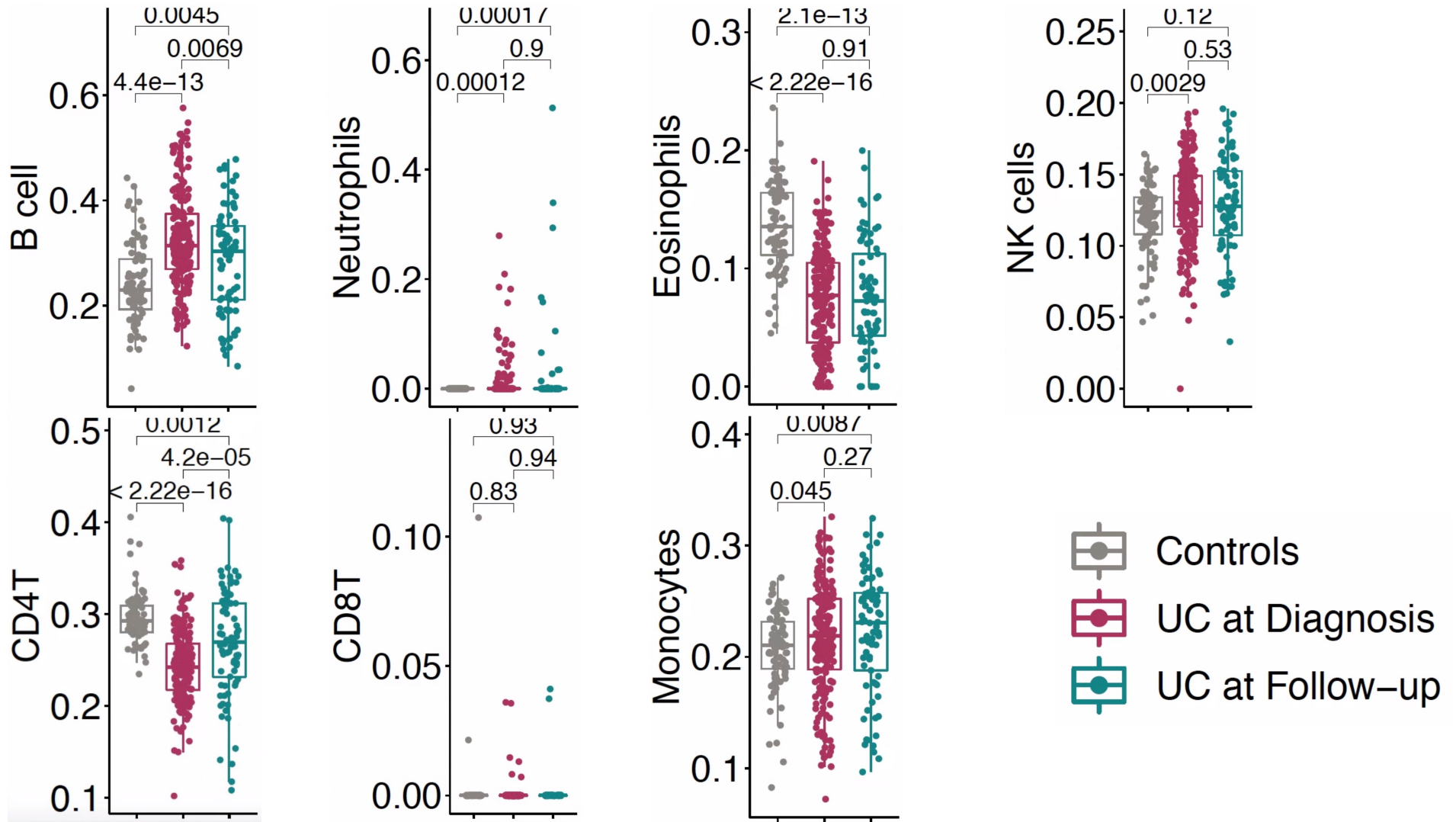
Supplementary Figure 6: Overall estimated cell proportions for immune subtypes from rectal biopsy ~820K DNAm profile and they are compared among controls (n=85), UC at diagnosis (n=211) and UC at follow-up (n=73) are shown. X-axis shows the disease status and y-axis shows the estimated cell proportions from the Epidish CellDMC package. P-values are shown from the Wilcoxon test.
