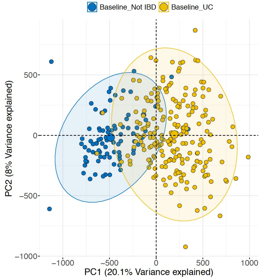
Supplementary Figure 1: The principal component analysis on entire ~820k sites shows two distinct clusters for controls and UC at diagnosis.
