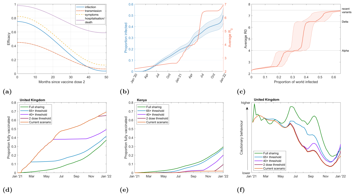
Figure 1: (a) Efficacy profiles used for vaccination following the second dose of vaccination. (b, c) Estimates for infected proportion of the global population (blue) and average R_0 of SARS-CoV-2 strains in circulation (red). Higher and lower infection estimates are indicated by thinner outer lines with median estimates indicated by the thicker central line. Solid lines/shaded region are based on data to date, with the dotted lines/unshaded regions future projection. (b) shows separately the correlation between infection numbers with time (left axis, blue) and R_0 with time (right axis, red), (c) shows the correlation between infected proportion and average R_0 . (d, e) Example plots comparing levels of vaccination over time in each scenario considered for a highly vaccinated nation (the United Kingdom) and a nation with limited vaccination (Kenya). (f) Example plot for a highly vaccinated nation (the United Kingdom) of levels of cautionary behaviour used for each level of vaccine sharing, for scenarios with adapted behaviour.
