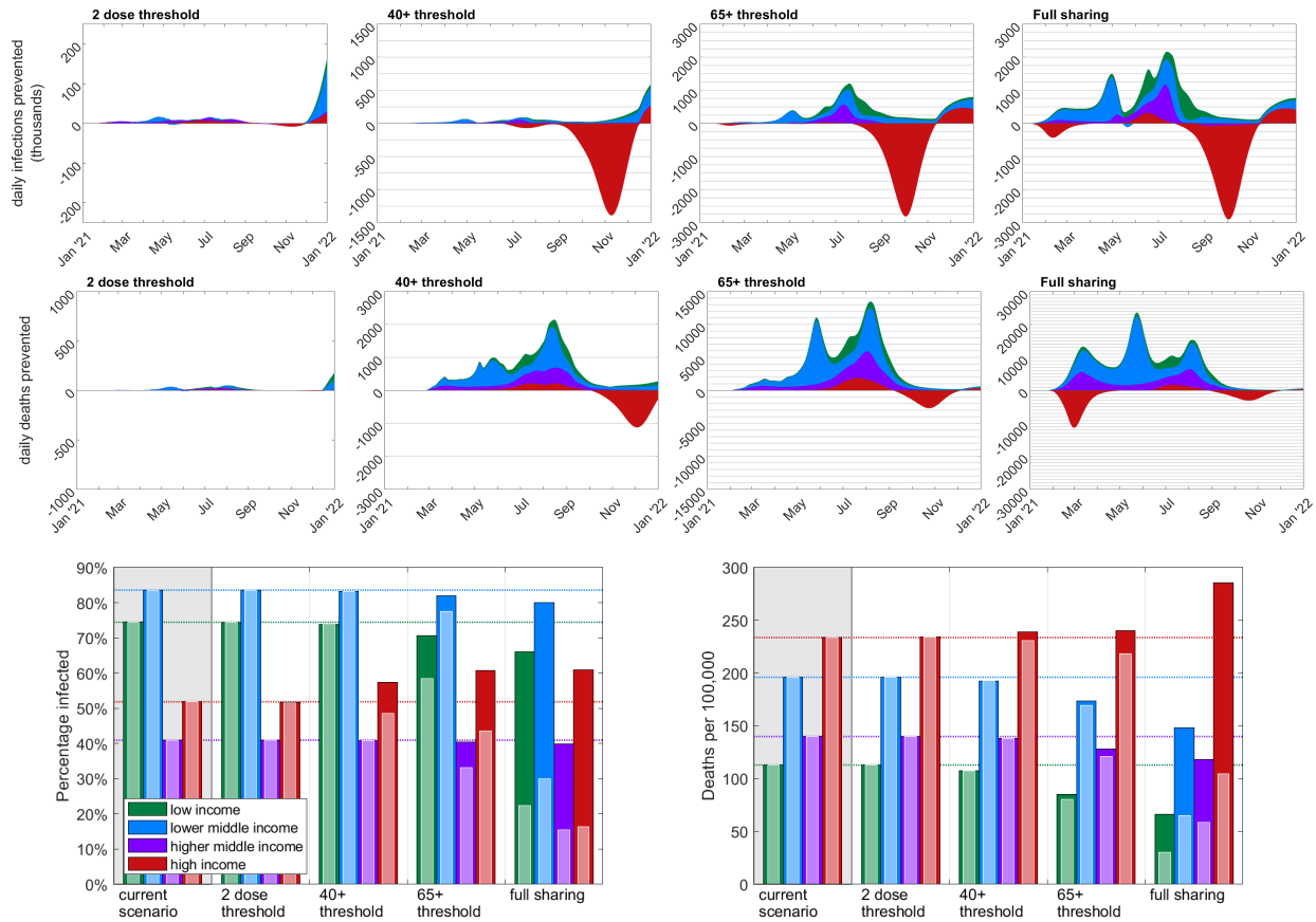
Figure 3: The top two rows give time series plots showing the reduction in the global number of daily infections and daily deaths compared to the default scenario. The different coloured areas represent the proportion of infections/deaths prevented in countries from each economic group: low income (green); lower middle income (blue), higher middle income (purple); high income (red). The columns show the four different vaccine sharing scenarios, each assuming unadapted behaviour. Equivalent figures for adapted behaviour are given in Fig S2. The lower plots show predicted total proportion infected (left) and deaths per 100,000 (right) from COVID-19 by the start of 2022 in each of the economic regions. The darker (rear) bars represent simulations where unadapted behaviour is followed, reflecting the default fitting in each. The lighter (front) bars represent simulations with adapted behaviour in countries commencing vaccine sharing. The first group of bars in each (grey shaded region) and dotted lines, correspond to the default scenario with subsequent bars representing simulations with the four different vaccine sharing strategies. All results presented here are simulation averages, with associated prediction intervals listed in Table 1.
