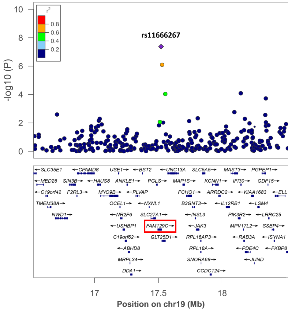
Figure 3 | LocusZoom plot of the region containing rs11666267.
