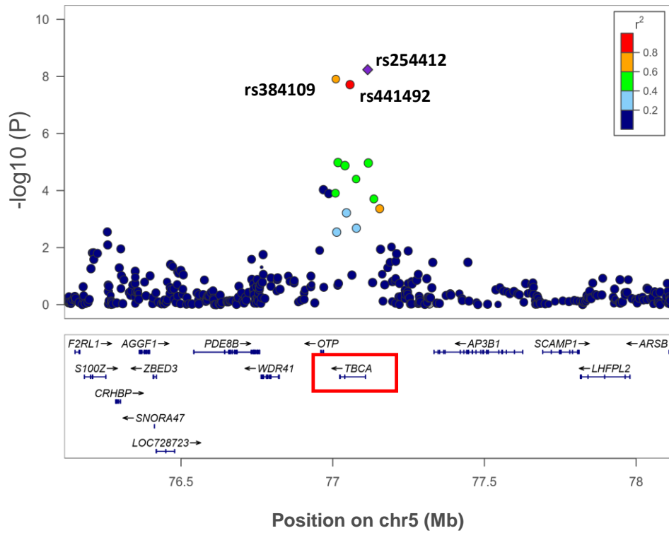
Figure 4 | LocusZoom plot of the region containing rs254412, rs384109 and rs441492.
