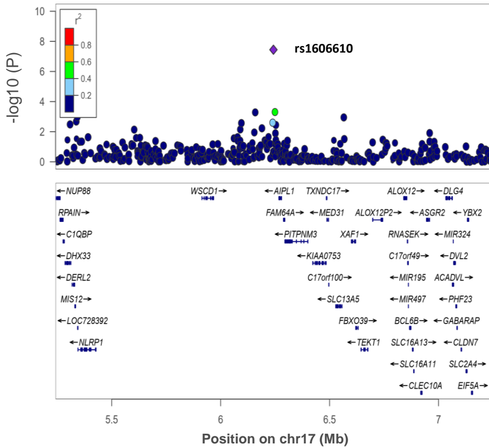
Figure 5 | LocusZoom plot of the region containing rs1606610.
