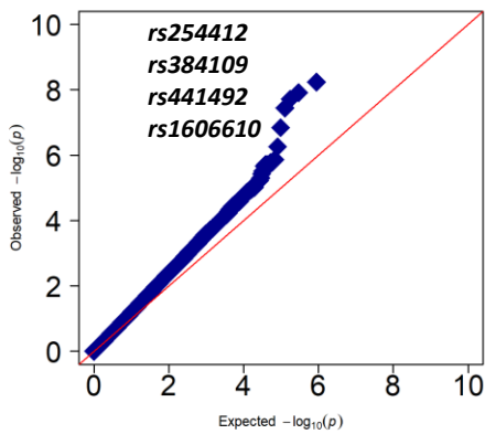
Figure 2 | QQ plots of mitonuclear associations in PD
