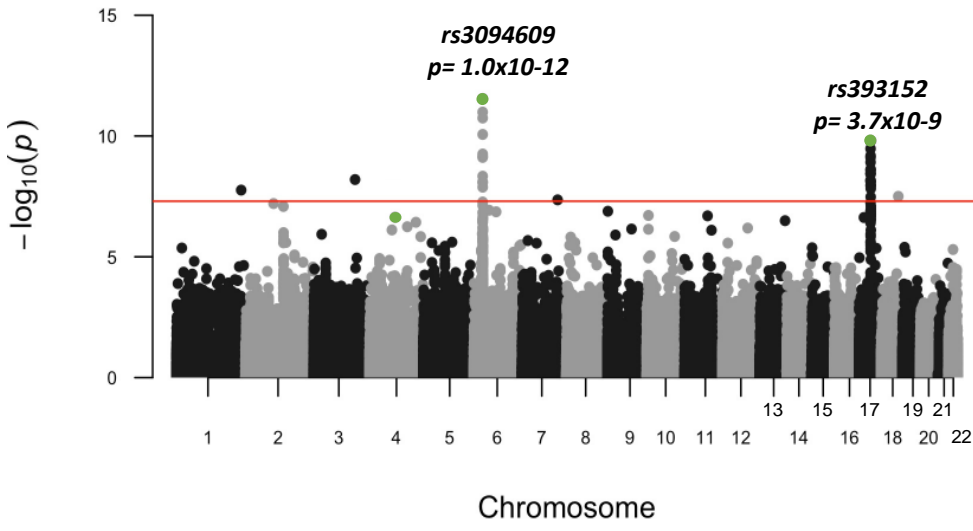
Figure 6 | nSNPs in PD versus Controls (58CNBS).
