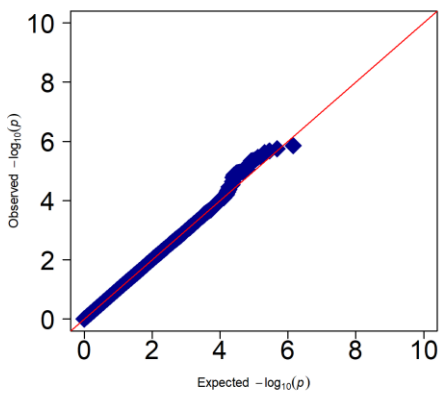
SFigure 1 | QQ plots of mitonuclear associations in 58C/NBS cohorts combined.
