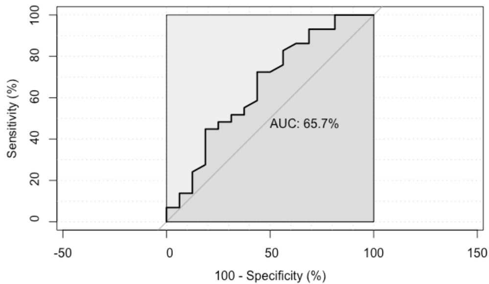
Figure 1: ROC curve analysis of the total study participants (AUC = 66% with the best new cut-off for FIB-4 score = 0.32) (ROC: Receiver operating characteristics, AUC: area under the curve)
