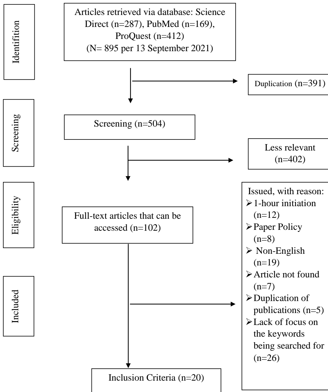
Figure 1. PRISMA Flowchart
