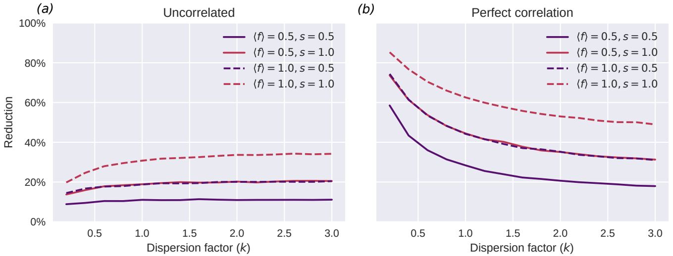
FIG. S1. A Poisson (constant-rate of testing) model of heterogeneous, regular testing performs qualitatively similarly to the fixed-interval model of the main text. a) Uncorrelated test frequency and activity distributions b) Perfectly correlated test frequency and activity distributions.
