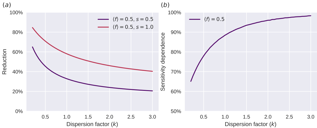
Figure 4. Testing heterogeneity can be turned to an advantage. Here, perfect correlation between social activity and test frequency is assumed. (a) (left): Reduction in the reproductive number as a function of the dispersion coefficient k (lower k corresponding to more pronounced heterogeneity). Note that for the fully correlated case, increased heterogeneity leads to better epidemic control (higher reduction in the reproductive number), in contrast to what was observed in the uncorrelated case (Figure 3). (b) (right): The reduction due to regular testing depends less strongly on test sensitivity when heterogeneity is high, in the fully correlated case. The overall dependence is similar to the one observed for the uncorrelated case (Figure 3), only more pronounced.
