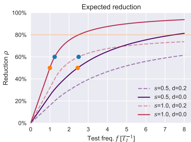
Figure 2. Efficient regular testing depends strongly on frequency and timeliness of results. The reduction in reproductive number obtained through regular testing depends strongly on the overall testing frequency. Concretely, assuming an infectious period of 5 days, a test with a sensitivity of just s = 50\% performed at an interval of 2 days is as effective as a perfect-sensitivity test performed every 5 days (orange dots). However, even a high-frequency testing scheme suffers if results are delayed. Assuming a 5-day infectious period again, a delay of just one day ( d = 0.2 ) has a sizable impact. Concretely, an instantaneous testing scheme performed every 4 days is as effective as delayed one performed every 2 days (blue dots). The dashed (delayed) lines asymptotically trend towards a maximum reduction value of 80% (orange horizontal line) with increasing test frequency. The delayed perfect-sensitivity test (dashed red line) only does so much more rapidly than its 50% sensitivity counterpart (dashed purple line)
