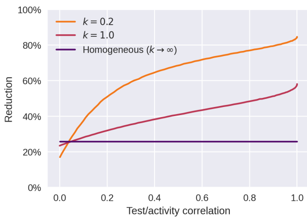
Figure 5. Only weak coupling is needed to leverage heterogeneity Dependency of reduction on the correlation between test frequency and activity. Across all three curves, the test frequency is set at f = 0.5 , and the test sensitivity is assumed ideal, i.e. s = 1 . Note that the turning point at which heterogeneity becomes an advantage rather than a disadvantage occurs at quite low correlations – as long as a correlation of more than \approx 5\% is attained, the heterogeneous scenarios ( k = 0.2 and k = 1.0 ) fare better than the homogeneous one ( k \rightarrow \infty ).
