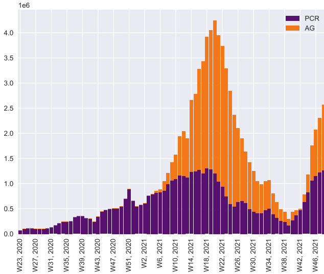
Figure 1. Overall level of testing over time, Danish data. Denmark has employed an extensive SARS-CoV-2 mass screening program. Assuming an infectious period of five days, the peak level of testing of approx. 4.4 million tests per week (attained around May 2021) corresponds to an average testing frequency of \langle f \rangle \approx 0.5 in our model.
