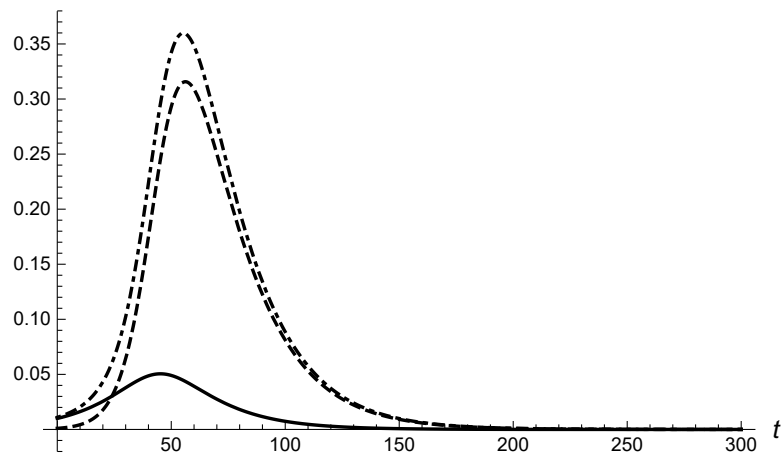
Figure 2: Fractions of the viruses 1 and 2 carriers as a function of time (in days): y_1(t) for virus 1 (solid line), y_2(t) for more contagious virus 2 (dashed line) and the sum y_1(t) + y_2(t) (dashed-dotted line) of the infected at moment t . The parameters p_1 = 0.1 , p_2 = 0.2 , T_1 = T_2 = 20 days, u(0) = 0.989 .
