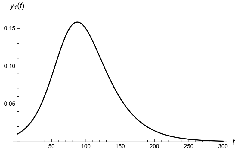
Figure 1: Function y_1(t) of virus 1 carriers for the case when second virus is absent at all (time in days). The parameters are p_2 = 0 , y_1(0) = 0.01 , u(0) = 0.99 and the average duration of the virus carrier T_1 = 20 days.
