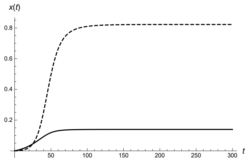
Figure 4: The functions x_1(t) and x_2(t) of the affected by the viruses 1 and 2 people in the case II .
