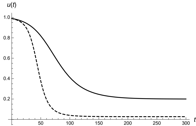
Figure 3: Time behavior of function u(t) for the cases I and II .
