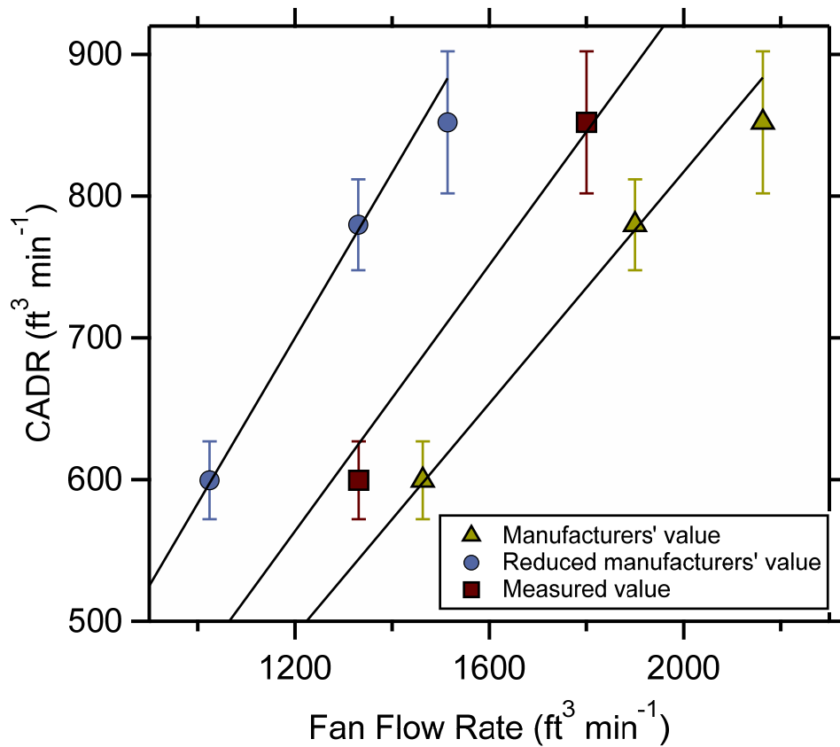
Figure S4. Relationship between CADR for the Corsi-Rosenthal Box and the manufacturer reported (yellow triangles), the reduced manufacturer reported (blue circles), and air-velocity-estimated (red squares) air flow rates for the original box fan. The lines are linear fits forced through zero (slopes = 0.41, 0.58, and 0.47, respectively).
