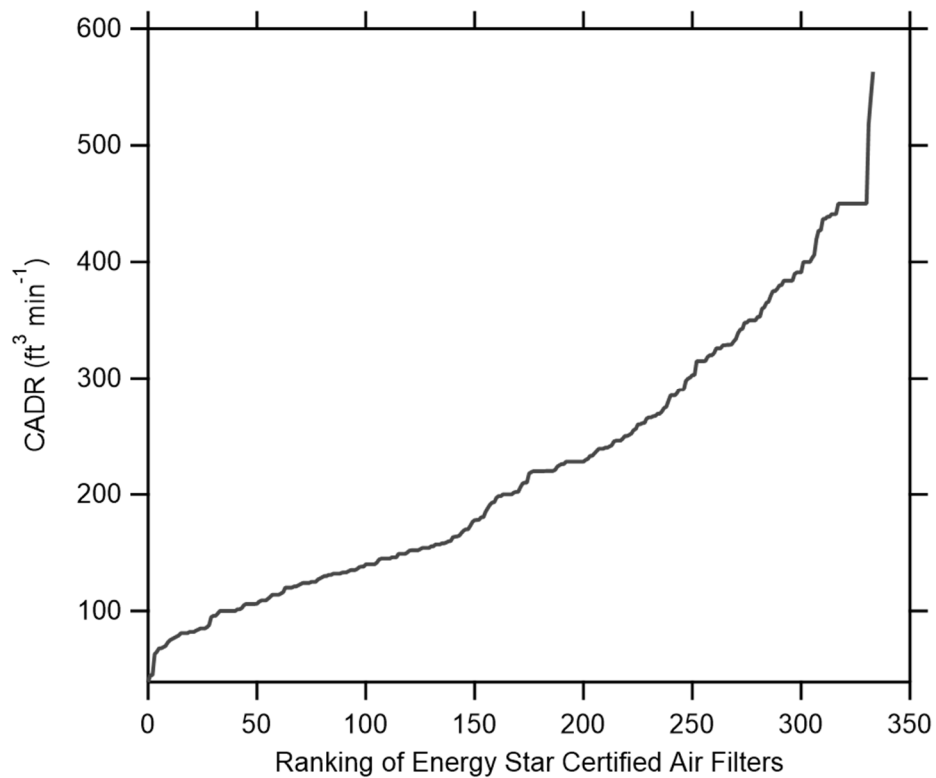
Figure S5. The distribution of maximum CADR values for commercially available air filters in the Energy Star database. These can be compared with the Corsi-Rosenthal Box.
