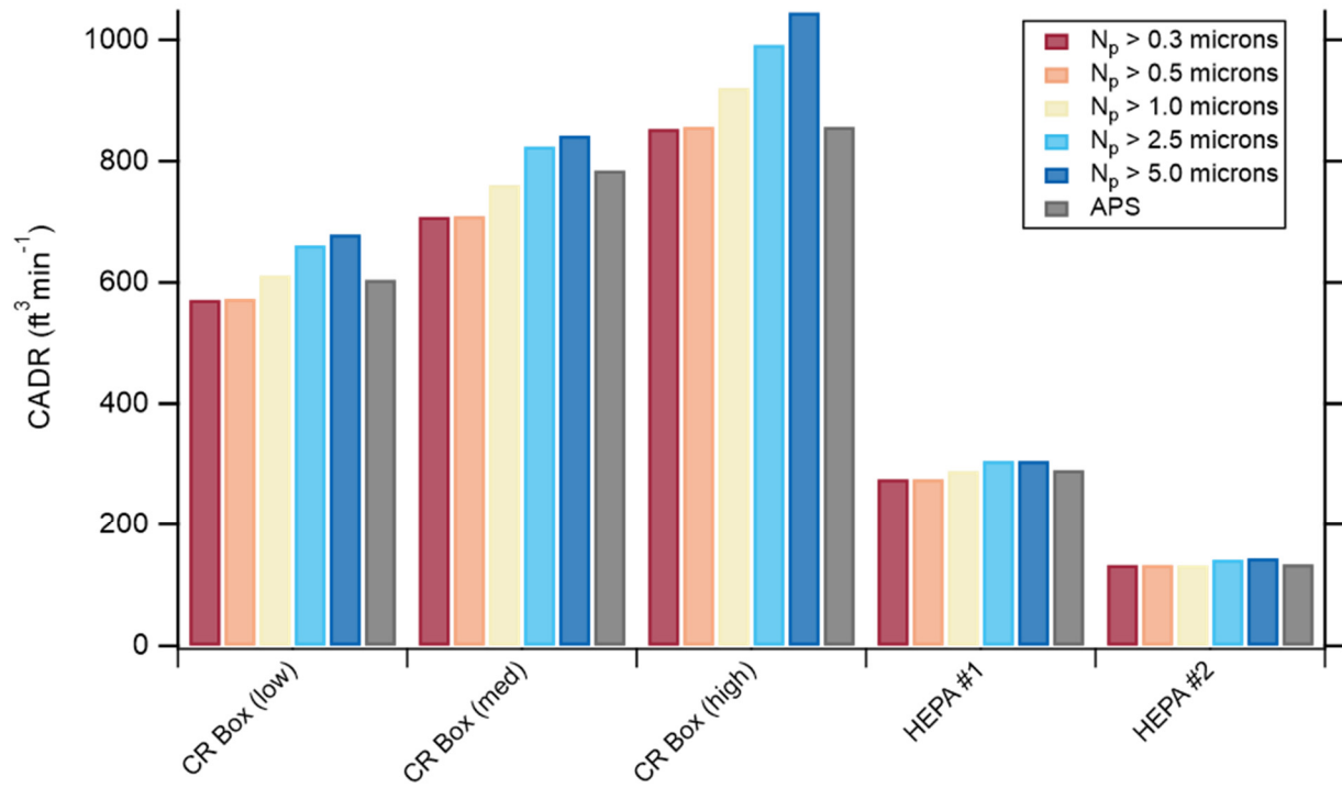
Figure S6. Comparison of the CADR values determined using the different apparent size bin number concentrations from the low-cost sensor (colors) compared to the CADR_{N_p} determined from the APS. Measurements are from the home office.
