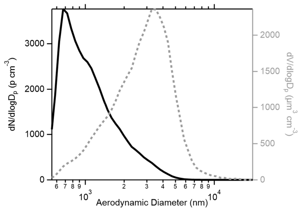
Figure S1. Number weighted (black solid, left axis) and volume weighted (gray dashed, right axis) particle size distributions for the particles produced from the nebulizer.
