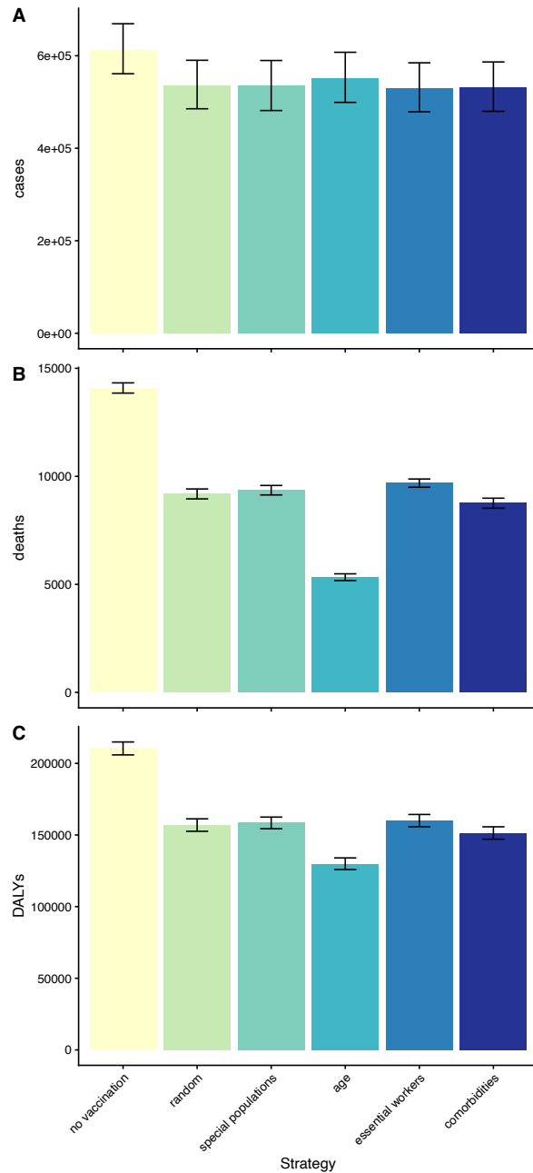
Figure 3. Simulated impact of different COVID-19 vaccine prioritization strategies in California on numbers of COVID-19 clinical cases, deaths and DALYs for 5 million people vaccinated. Simulated (A) clinical cases, (B) deaths and (C) DALYs in California in the first 6 months of 2021. Five different prioritization strategies were considered: (i) random allocation, (ii) targeting special populations (prisoners, education workers, people experiencing homelessness), (iii) age targeting, (iv) targeting essential workers, (v) targeting individuals with comorbidities. All strategies assumed that all healthcare workers and long-term care facility residents were vaccinated first as per the US CDC recommendation 12 . Vaccine efficacies against clinical disease and death were assumed to be initially 90% and 95% and to wane gradually over time (see Supplementary Information). Bars show mean estimates across 1000 simulations, error bars show 95% uncertainty intervals from stochastic uncertainty and parameter uncertainty. Results for 2 million and 10 million individuals vaccinated are shown in Figure S3.
