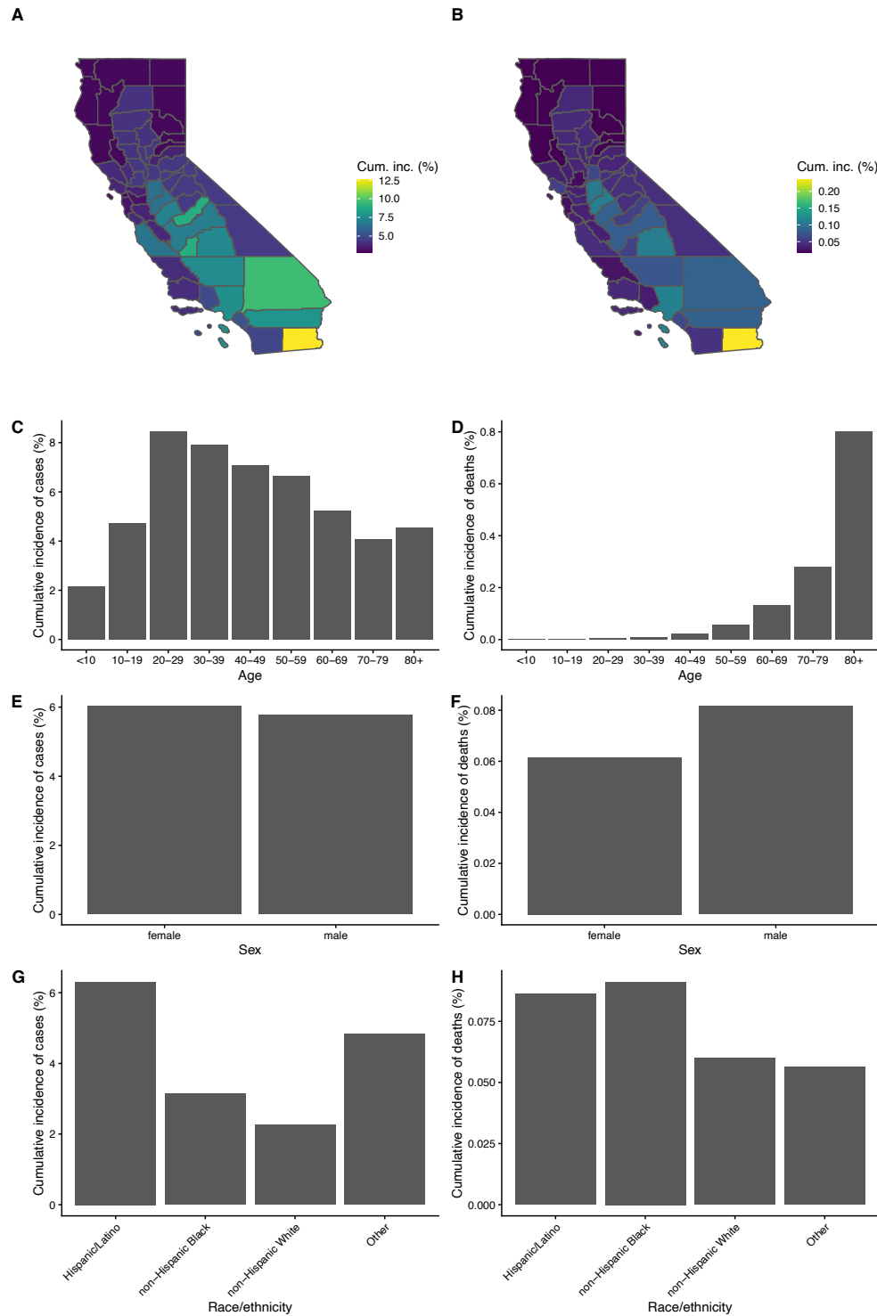
Figure 1. Cumulative incidence of confirmed COVID-19 cases (left column) and deaths (right column) in California up to December 30, 2020, by key demographic factors (rows). Cumulative incidence by (A-B) county of residence, (C-D) age, (E-F) sex, and (G-H) race/ethnicity. Data from California Department of Public Health. Counties with population <250,000 (except Imperial) were combined into a single region by their economic region, San Benito County was combined with Santa Cruz County, and Napa County was combined with Sonoma County. Plotted cumulative incidence for these counties represents the cumulative incidence of the combined region.
