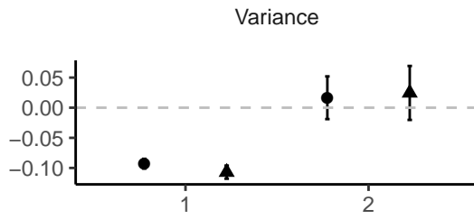
Testosterone SHBG (rs1799941) Sex
