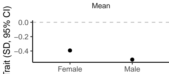
Testosterone SHBG (rs1799941) Sex
