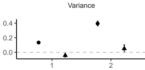
ALT TM6SF2 (rs58542926) BMI
