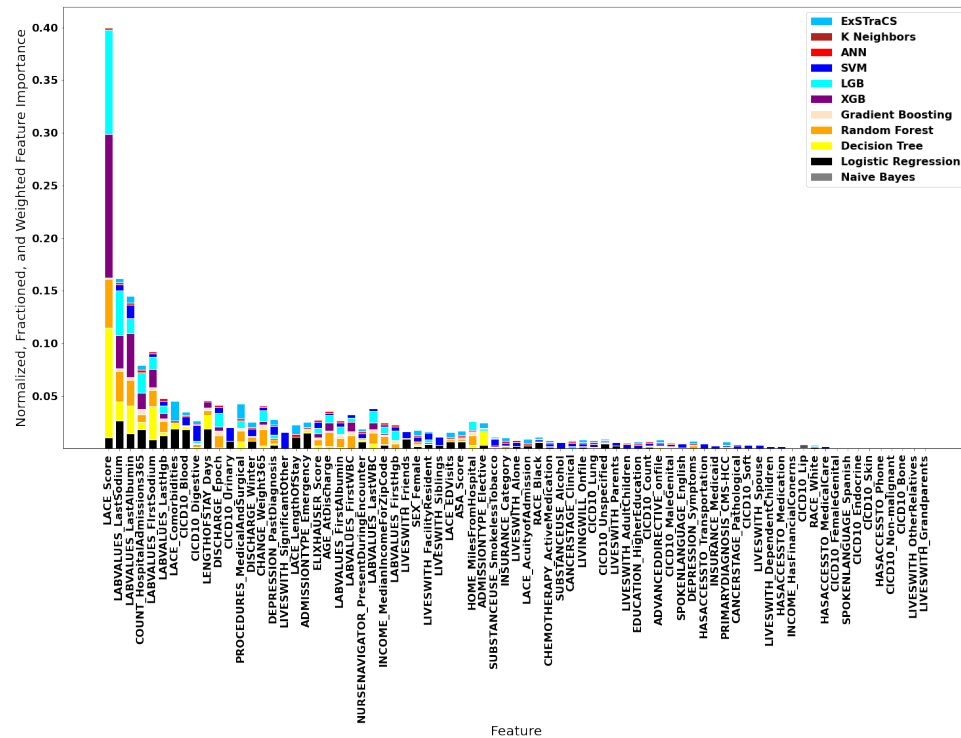
Figure 6: Plots of feature importance for all features
