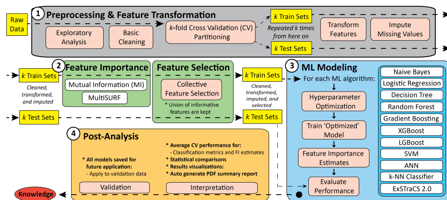
Figure 1: Schematic of the rigorous ML analysis pipeline applied in this study separated into four phases
