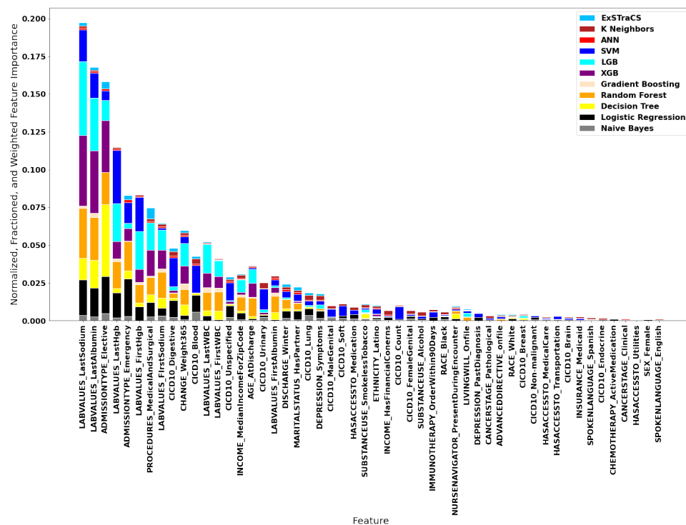
Figure 7: Plots of feature importance for 48-hr features
