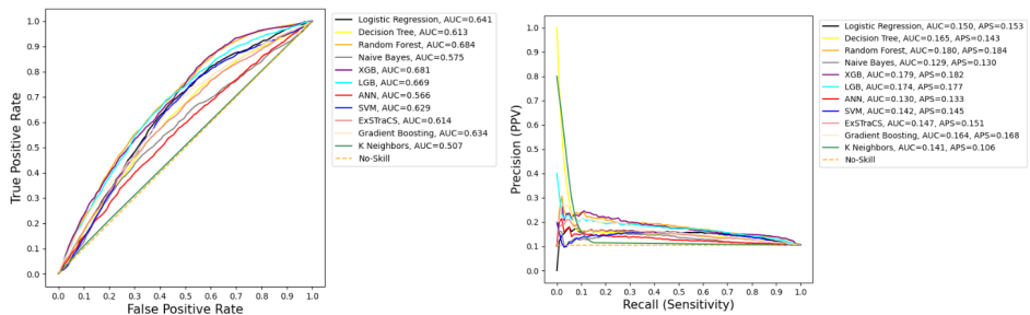
Figure 4: AUROC, 48-hr features, validation set Figure 5: AUPRC, 48-hr features, validation set
