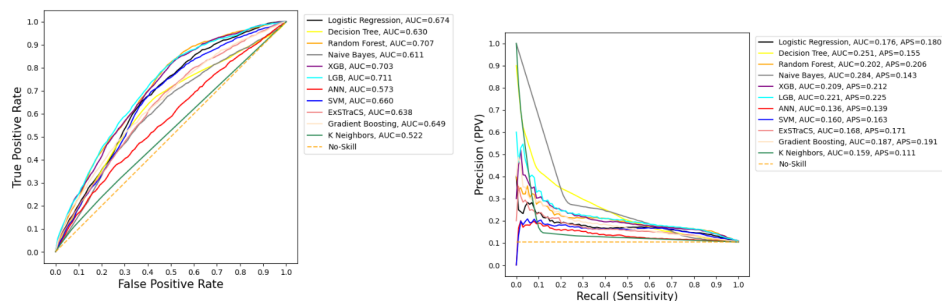
Figure 2: AUROC, all features, validation set Figure 3: AUPRC, all features, validation set
