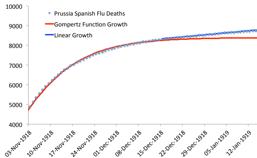
Figure 75: Transition from Gompertz Function growth to linear growth in cumulative Spanish Flu deaths in Prussia.
