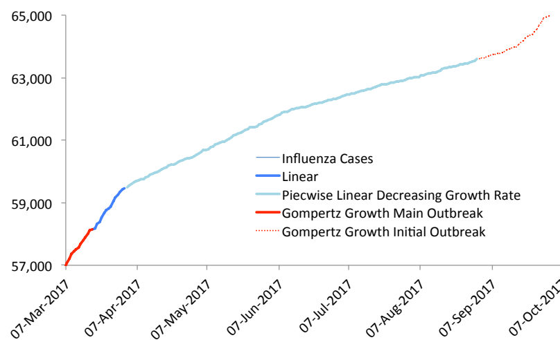
Figure 62: Detail of the 2016-17 cycle shows declining growth in the piecewise linear phase and a very rapid increase in September.
