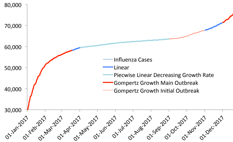
Figure 61: The annual cycle Gompertz Growth to Linear Growth to Gompertz Growth.
