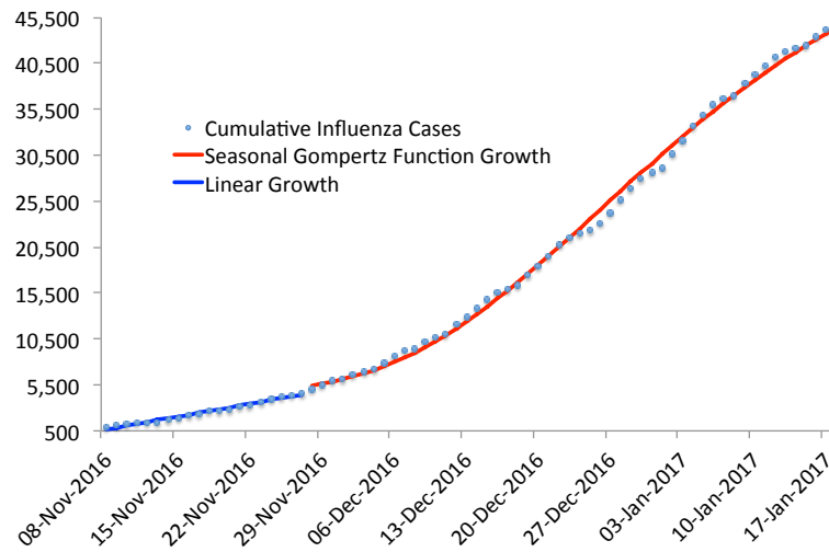
Figure 58: The 2016-2017 Influenza Season begins with the transition from Linear to Gompertz Function Growth.
