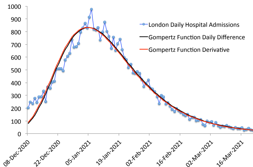
Figure 50: \dot{X} and Daily Differences for London Hospital Admissions 8 Dec 2020 to 21 Mar 2021 show the characteristic rapid rise and slow decline in \dot{X} .
