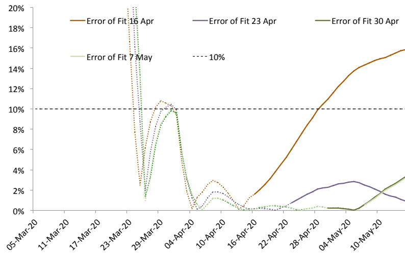
Figure 46: Evolution of errors in Gompertz Function fits to Portuguese Hospital Admissions.
