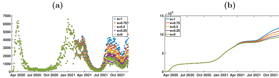
Figure 4: We plot \widehat{\text{CR}}_{\text{Data}}(t)' in (a), and we plot \widehat{\text{CR}}_{\text{Data}}(t) in (b) for New York City, and e = 0, 0.25, 0.5, 0.75, 1 . In (a), the green dots for e = 0 corresponds to the original daily number of reported cases \text{CR}_{\text{Data}}(t)' . In (b), the green curve for e = 0 also corresponds to the original cumulative number of reported cases \text{CR}_{\text{Data}}(t) .
