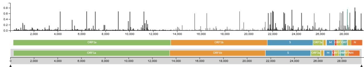
Figure 1a. Mutational hotspots as measured by entropy score across the SARS-COV-2 genome
