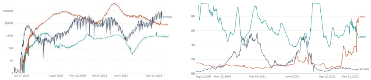
Figure 5. Confirmed cases and fatality rate of SARS-CoV-2. A) Daily confirmed cases of SARS-CoV-2 B) Moving average case fatality rate of SARS-CoV-2
