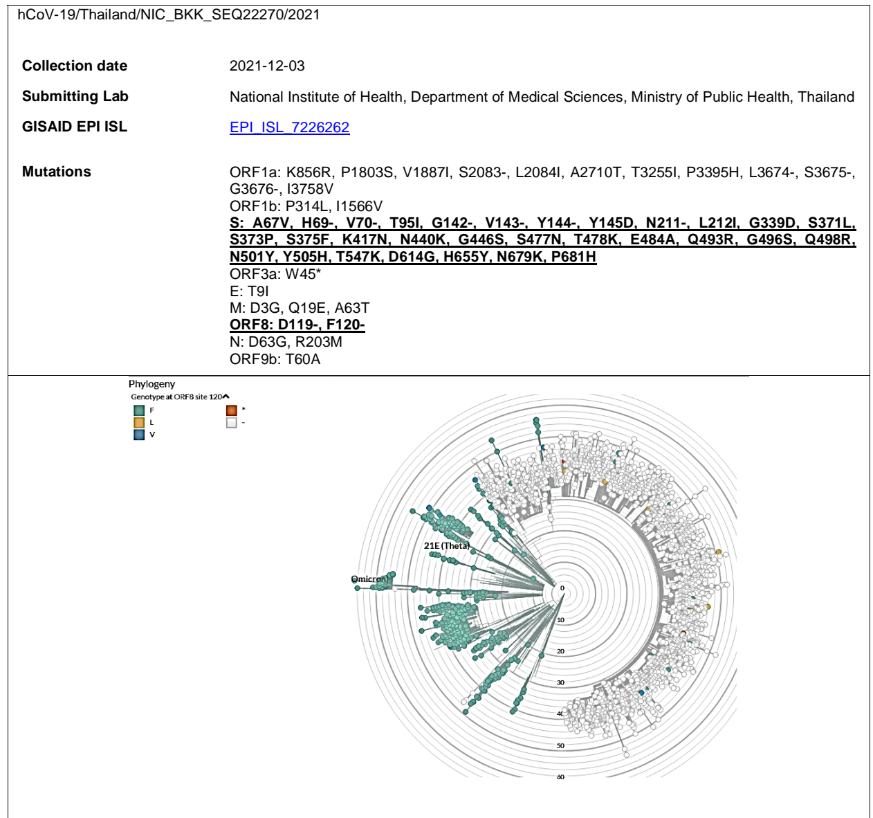
Figure 6. Omicron variant with the F120- mutation in ORF8 is indicated by white open circle and been fund in Sri Lanka, Thailand, Botswana, South Africa, and Ghana
