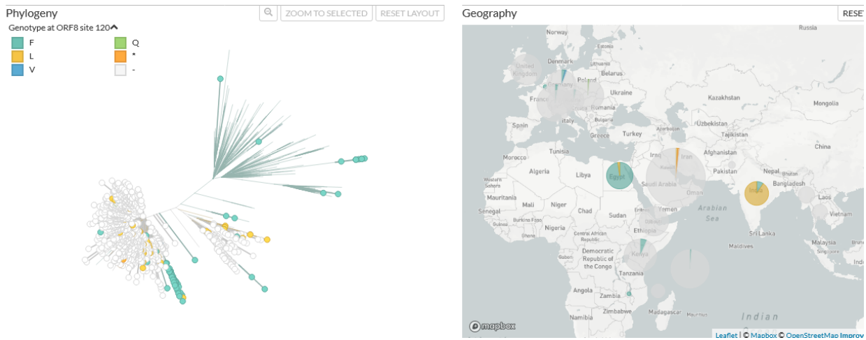
Figure 4. Phylogeny tree of residue 120 ORF8. The variants dominate Egypt for F mutation and L mutation for India.
