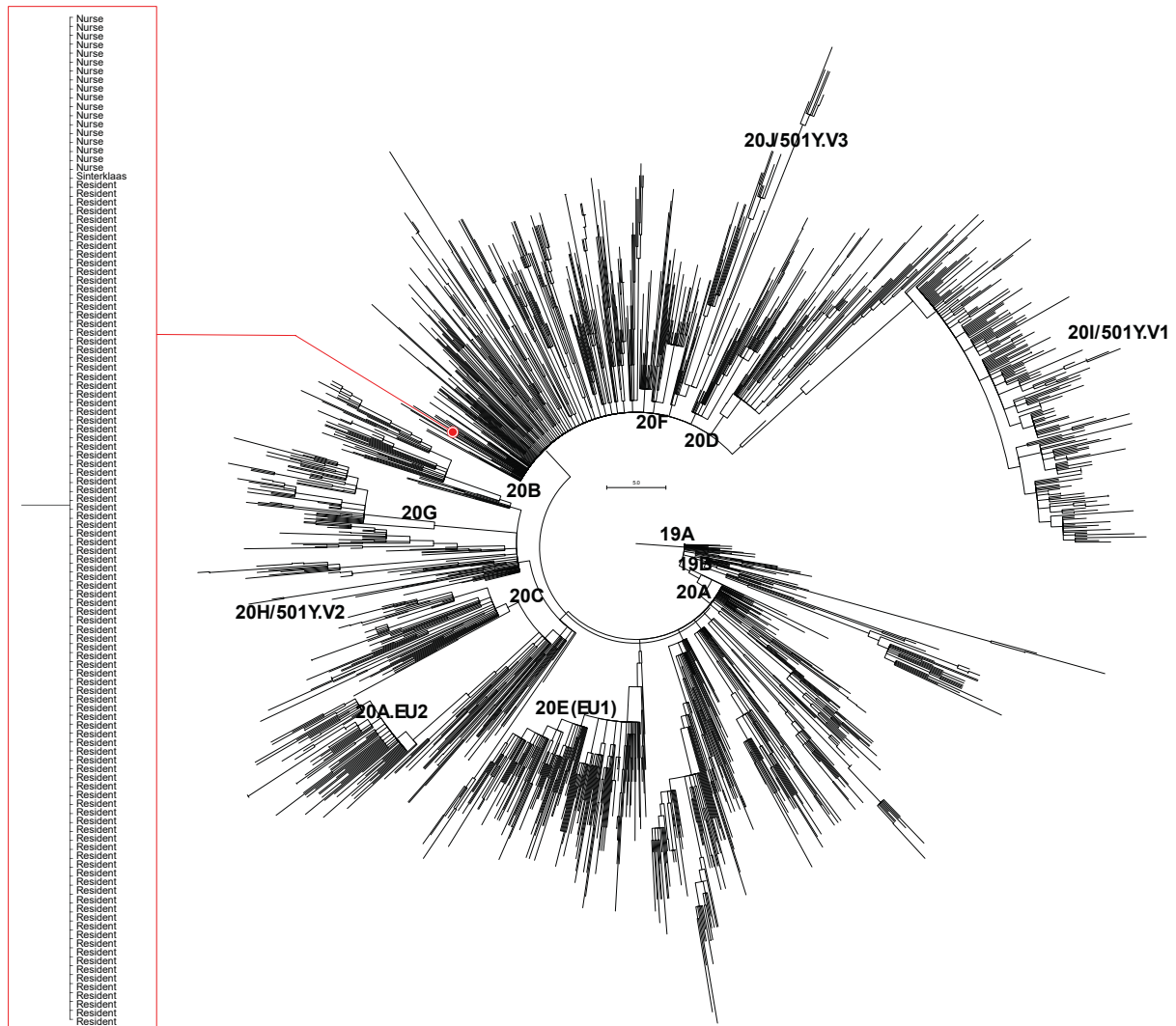
Figure 2. Phylogenetic tree of B.1.1. Maximum likelihood tree showing the genomes of the nursing home outbreak cluster as one large monophyletic cluster (see inset) within the SARS-CoV-2 lineage 20B cluster, confirming a single introduction event into the nursing home.
