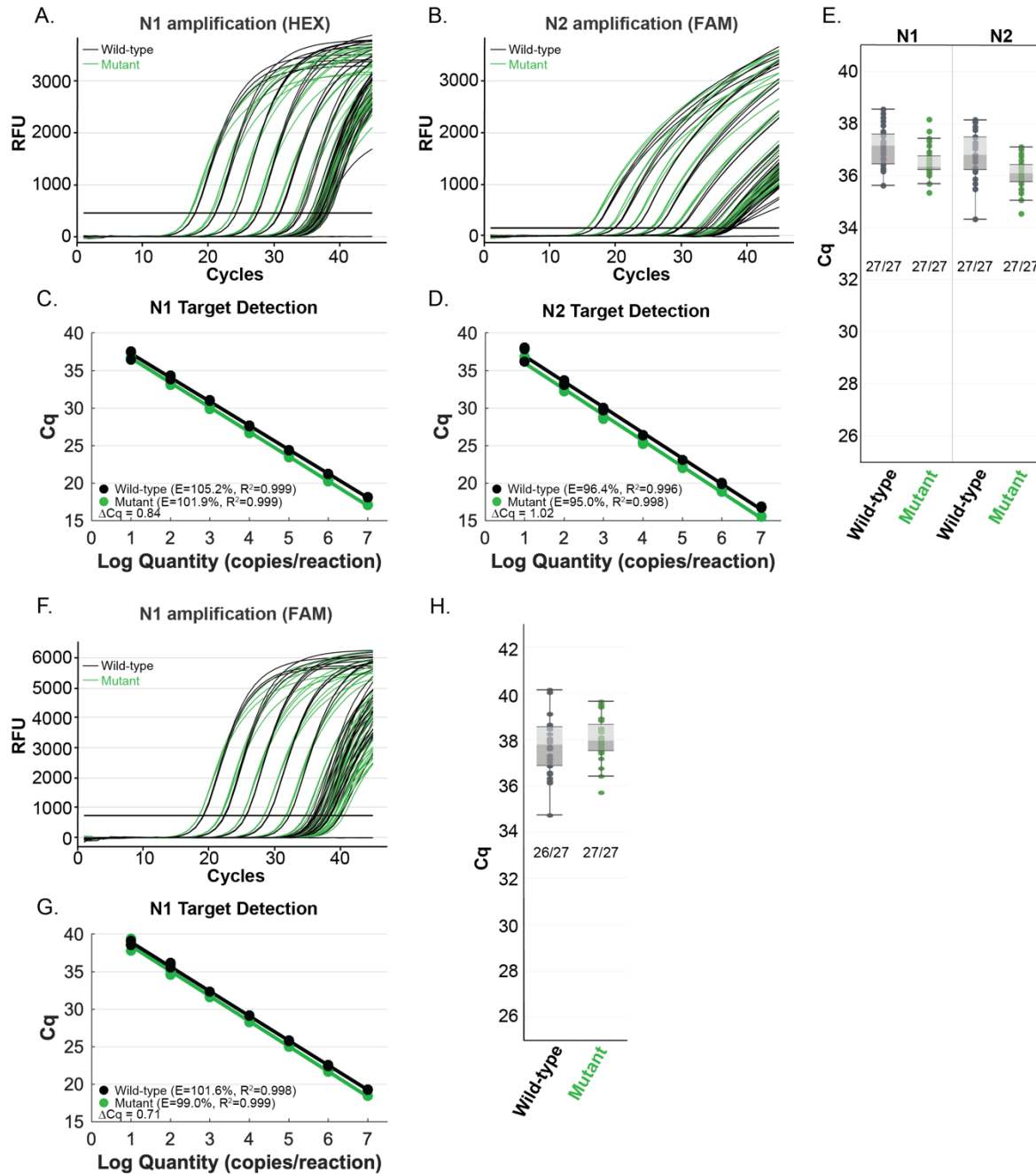
Figure 2. The NEB SARS-CoV-2 Multiplex Assay (A-E) and the SalivaDirect RT-qPCR protocol (F-H) efficiently detect N gene IVT RNA carrying the Omicron mutation with the CDC 2019-nCoV_N1 primer-probe set. Amplification efficiency in A-D and F-G was evaluated in triplicate over a 7-log range ( 10^7 -10 copies/reaction) of synthetic wild-type RNA (black) versus the Omicron mutant RNA (green). Detection sensitivity (E and H) was evaluated with 10 copies of RNA per reaction with 27 replicates per condition. All reactions tested with 10 copies of input RNA were detected by qPCR, except one wild-type sample amplified using the SalivaDirect RT-qPCR protocol.
