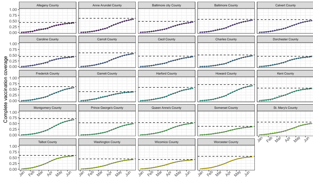
(c) Maryland model fits
