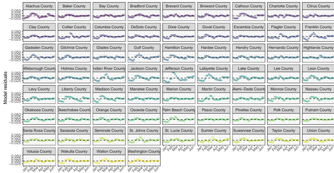
(a) Florida model fits
