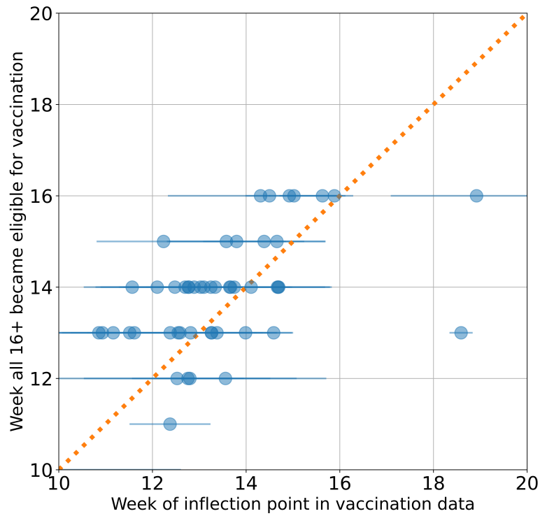
Figure S8: Transitions in vaccination We show the relationship between [x-axis] the model-fitted timing (week of 2021) of the inflection point (i.e., the transition between acceleration and deceleration in vaccination progress) for each state, with the standard deviation across counties and [y-axis] the week at which the state opened vaccination eligibility to the general public. The two outliers are NH and VT and NH has a significant discontinuity in its data making the model fit less accurate.
