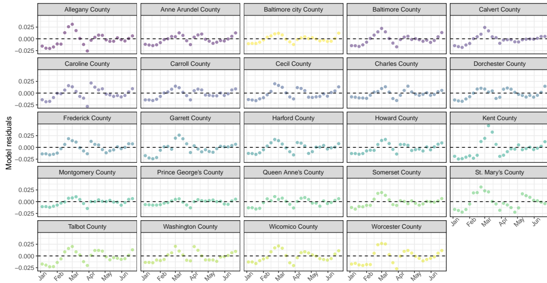
(c) Maryland model fits
