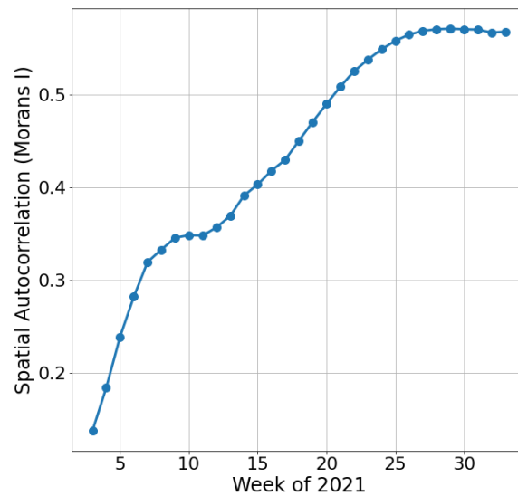
Figure S3: Spatial autocorrelation in county-level complete vaccination coverage as measured by Moran's I for every week of data through 2021.
