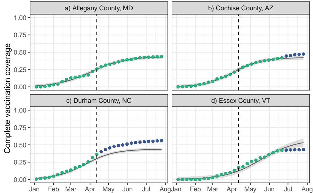
Figure 5: Vaccination dynamics compared to a simple model of growth. We provide examples of counties with the comparison of the vaccination data against the model fit from the logistic growth model. Weekly observations are colored by whether they fall inside (green) or outside (purple) the 95% prediction interval. The vertical dashed line marks week 15 (week ending April 18, 2021), the week after which deviations are identified. (a) The vaccination rates in Allegany County, MD show close adherence to the model expectation. All observations fall within the 95% prediction interval. (b) The vaccination rates in Cochise County, AZ rise above model expectations in late June. (c) The vaccination rates in Durham County, NC exceed model expectations beginning in mid-April. (d) The vaccination rates in Essex County, VT are lower than model expectations starting in late June.
