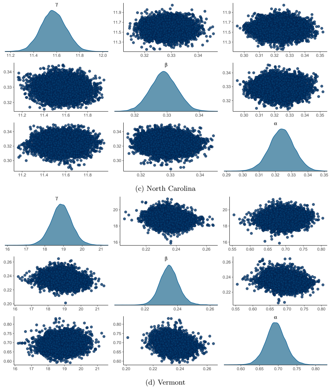
Figure S7: Density plots for marginal posterior distributions of main model parameters. We provide here a selection of marginal distributions for the four state models referenced in Figure 5. \alpha represents the asymptote parameter, \beta represents the rate parameter, and \gamma represents the inflection point parameter. Univariate marginal distributions are along the diagonal. Bivariate distributions are represented by the off-diagonal scatterplots.
