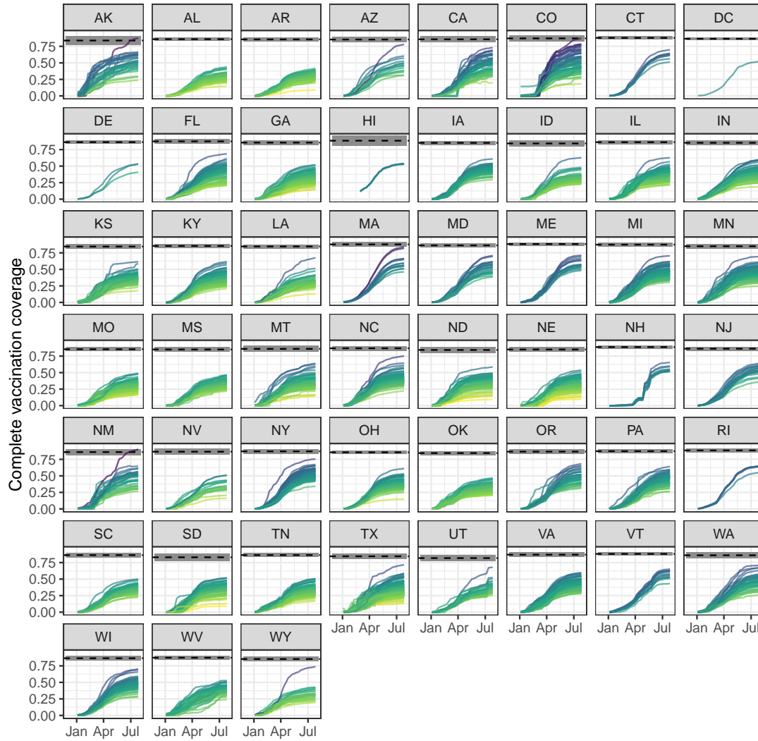
Figure 3: COVID-19 vaccination progress over time. Vaccination progress in each county generally follows a sigmoid shape through time, with an initial period of accelerated growth followed by a deceleration. Vaccination growth rate in most counties slows after June 2021, despite low coverage levels. Counties are colored by the complete vaccination coverage they reach by week 30, with lighter shades denoting lower coverage and darker shades denoting higher coverage. The average eligible population size (aged 12 years and above) for each state is denoted by the dashed black line, with a range of one standard deviation shaded in gray.
