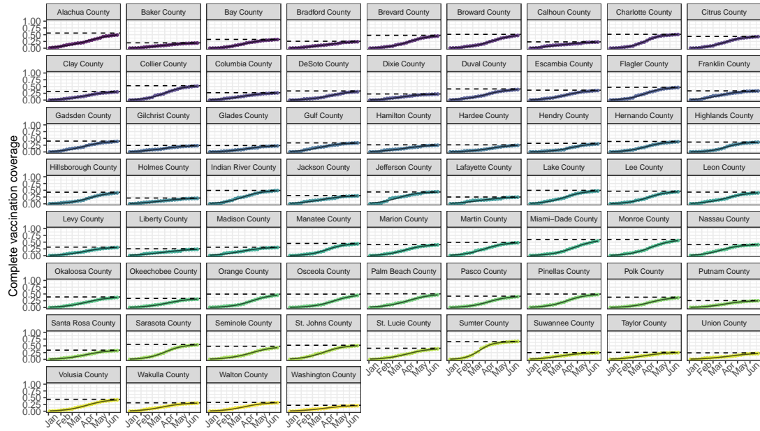
(a) Florida model fits
