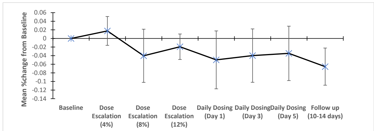
Figure 5: Graph showing LCI %change from baseline for all subjects (N=6). Values represent the mean change (%) in LCI from baseline \pm SE (error bars). The first week of the study period included Dose Escalation with 4,8 and 12% CO 2 . The second week of treatment includes Daily Dosing Days 1-5. Follow up was conducted 10-14 days after the final treatment. A lower absolute value indicates a positive treatment effect. Note: LCI graphs for individual CF subjects in supplementary Figures E-D are represented as % improvement in LCI values and are thus positive.
