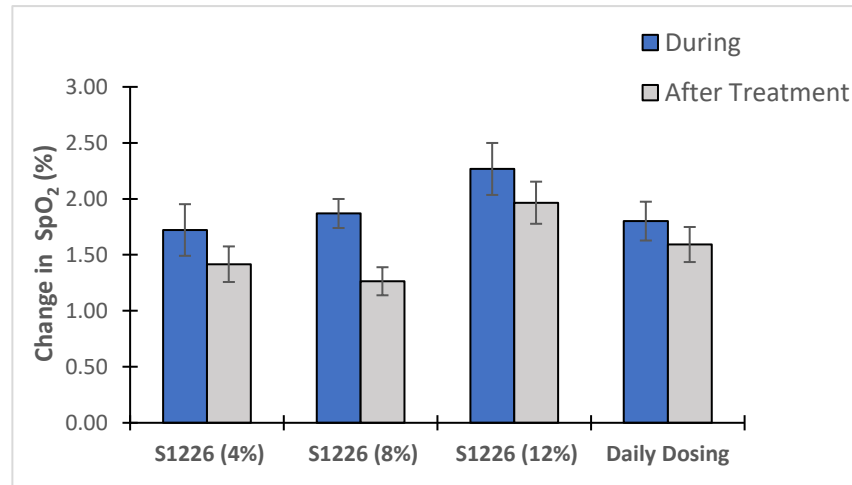
Figure 3: Absolute Change in % SpO 2 from baseline during (0-2mins) and immediately following treatment (2-4mins). for all subjects (n=6). All subjects showed increases in SpO 2 above baseline for all three concentrations of S-1226, (4, 8 and 12%). Subjects also showed a dose response relationship following treatment with S-1226. Error bars represent ± Standard Error (SE).
