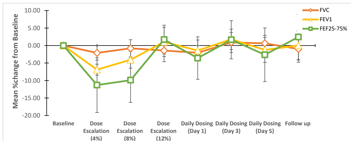
Figure 4: Spirometry results for all subjects (N=6). Values represent the average %change in FVC, FEV 1 and FEV 25-75% absolute values from baseline ±SE (error bars). The first week of the study period included Dose Escalation 4,8 and 12%. The second week of treatment includes Daily Dosing Day 1-5. Follow up was conducted 10-14 days after the final treatment.
