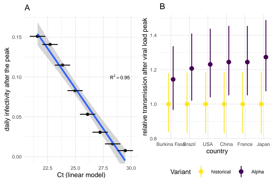
Figure 4: Impact of the differential viral genome copies on the transmissibility. A. Relationship between infectivity and Ct, after the viral genome copies peak, for the historical strain. B. The linear models parameters were used, with the demography of each country, to infer the transmission advantage of the variants. The error bars represent the 95% bootstrap quantile.
